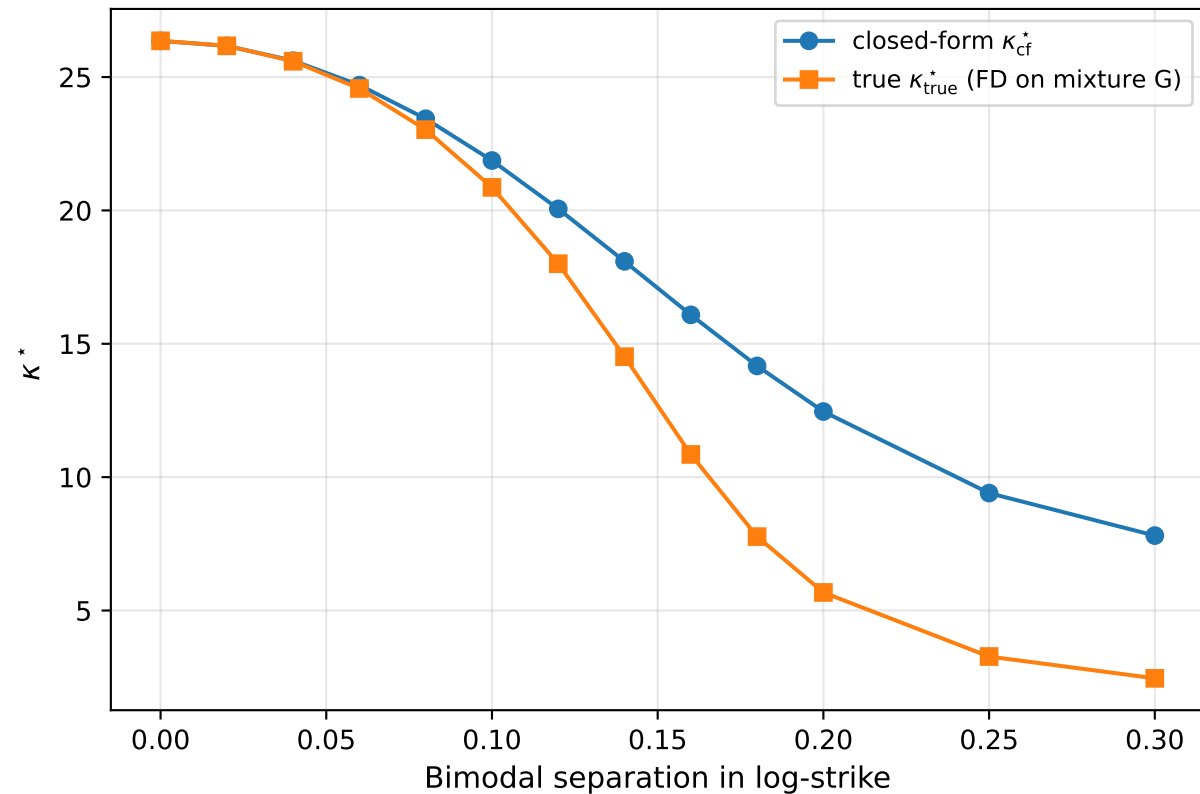
Closed-form vs true Hopf threshold
