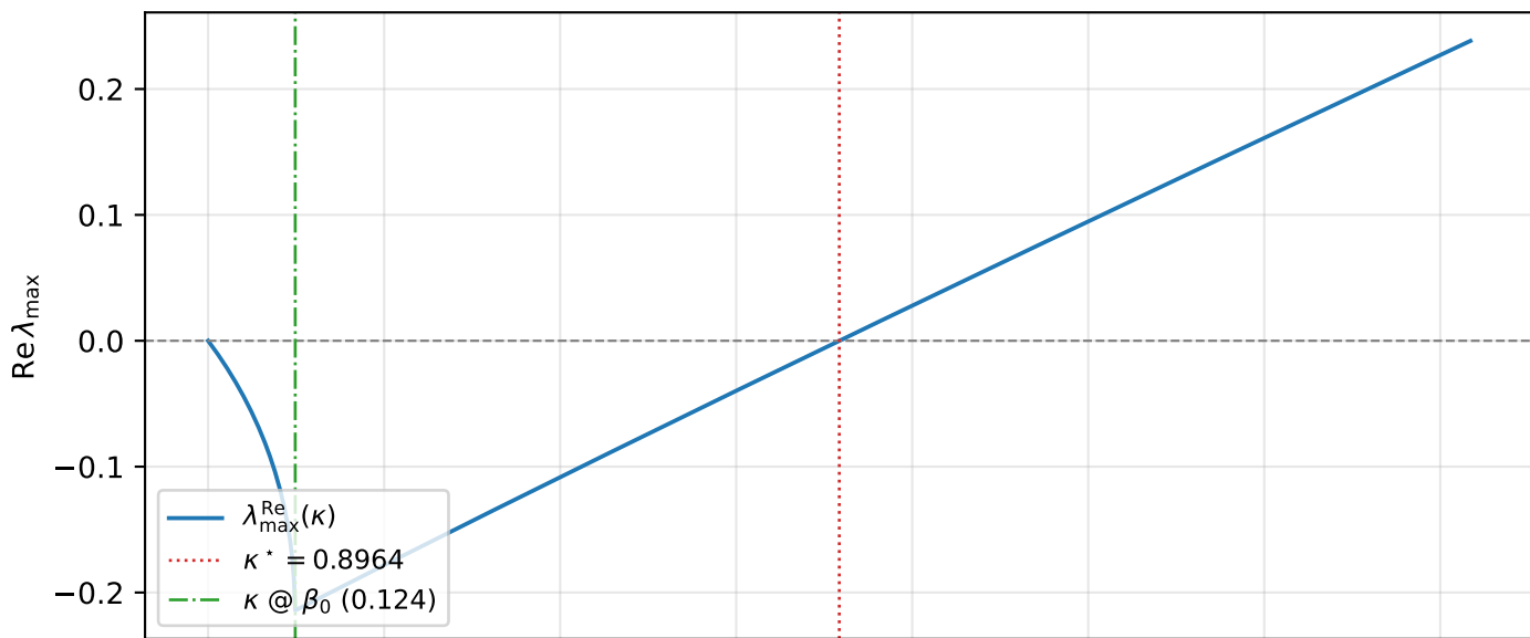
Leading-eigenvalue real part of J(\kappa)
