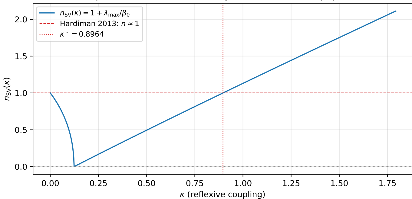
SV-equivalent Hawkes branching ratio (Theorem 2, paper §3.7)
