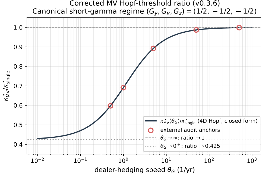
Figure 7: Corrected MV Hopf-threshold ratio \rho(\theta_G) = \kappa_{\text{MV}}^*/\kappa_{\text{single}}^* at the canonical short-gamma regime , log-x axis. Smooth monotonic approach to \rho(\infty^-) = 1 from BELOW; frozen-dealer limit \rho(0^+) = 8/21/\kappa_{\text{single}}^* \approx 0.425 . The five audit-table anchors (table 4) are overlaid as scatter markers. Run dir: runs/mckean_vlasov_validation/ .
