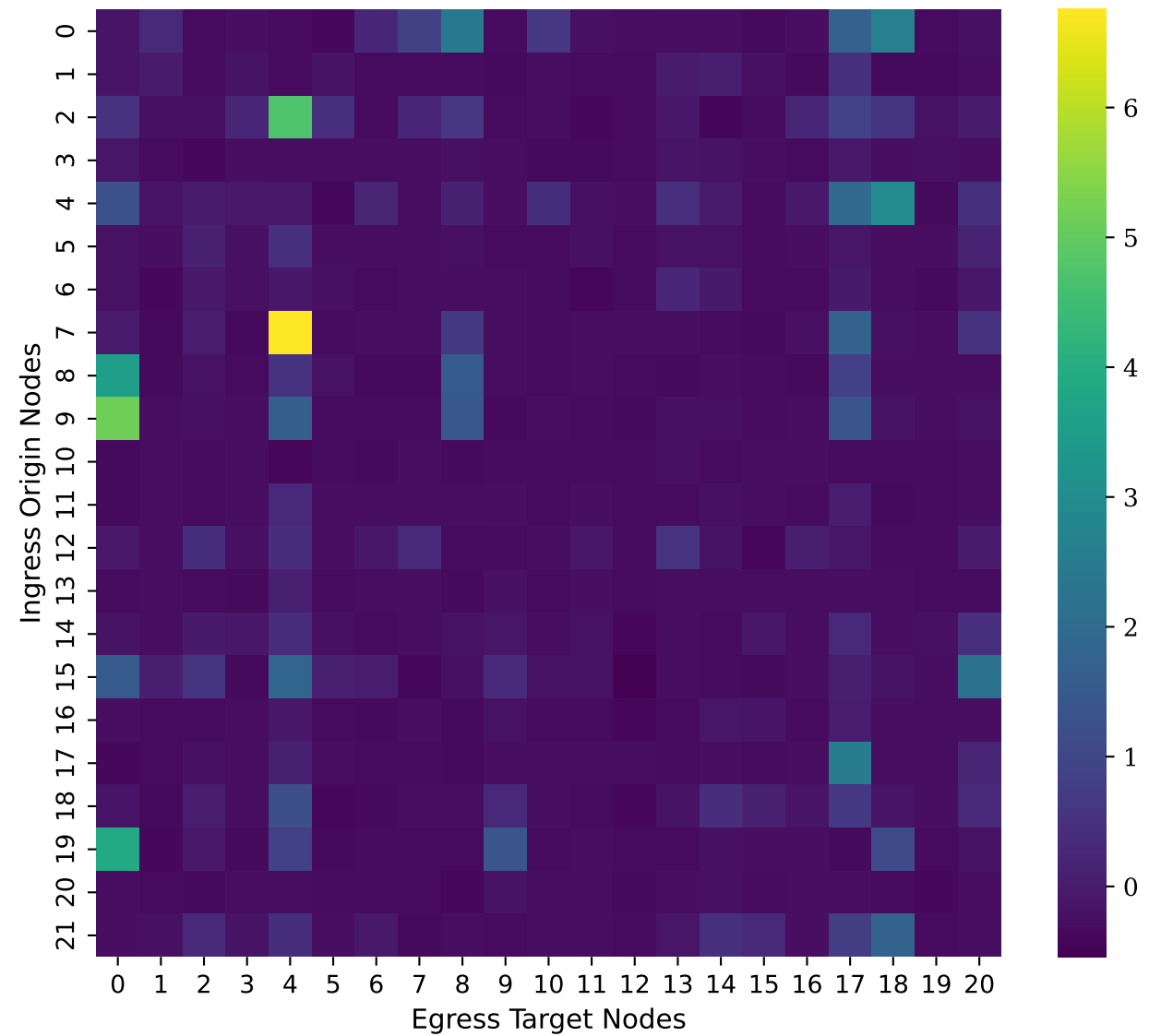
HaiFormer-6G Predicted Matrix ( \hat{Y} )
