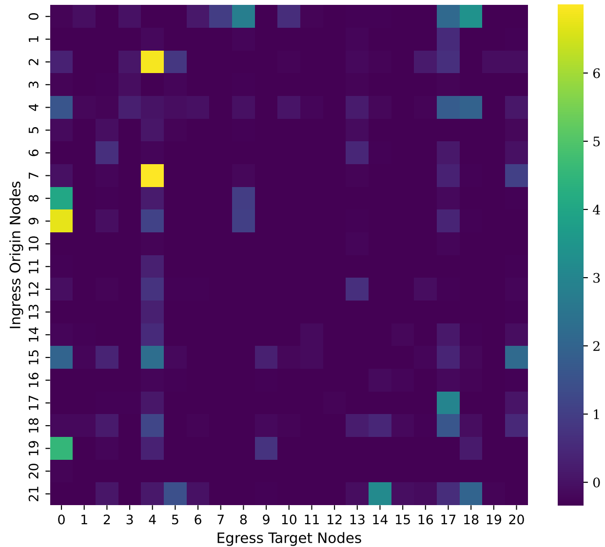
Empirical Ground Truth Matrix ( Y )
