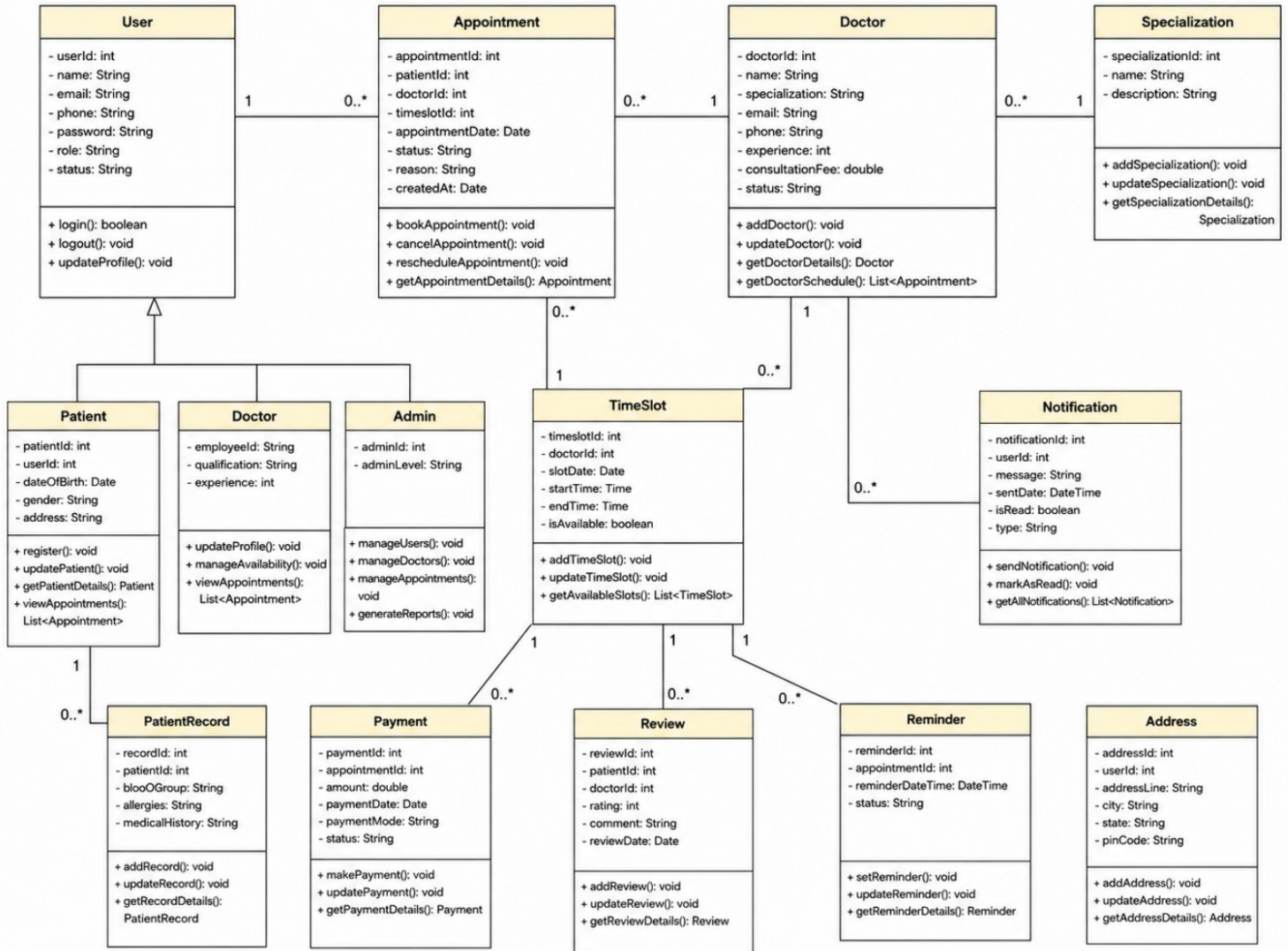
Class Diagram – Appointment Management System
