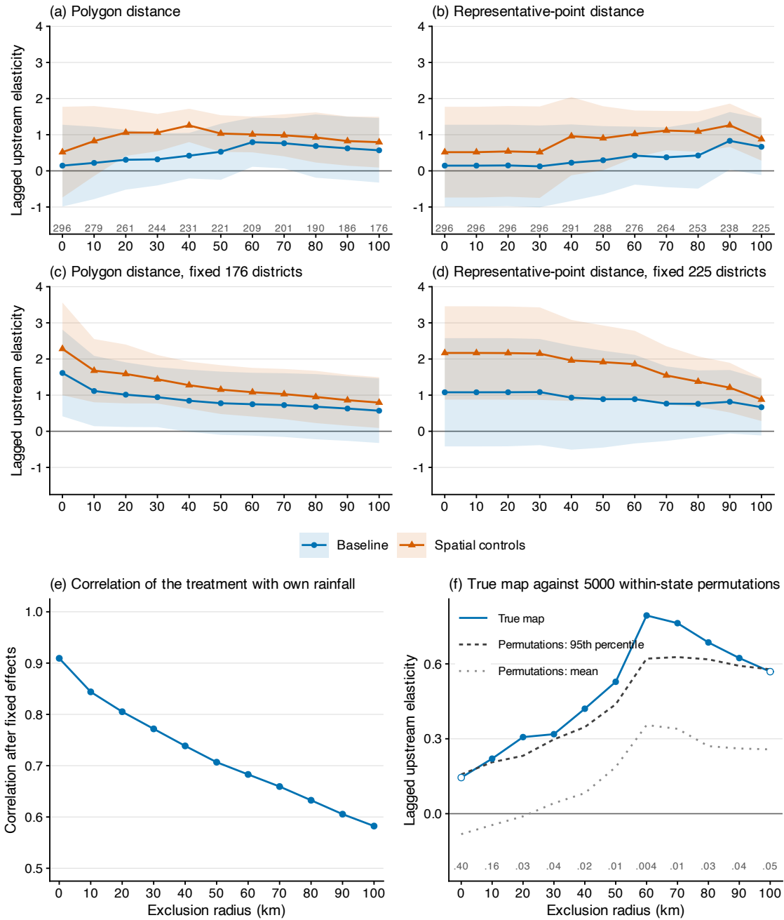
Figure A.2: The lagged upstream elasticity across a continuous exclusion radius
