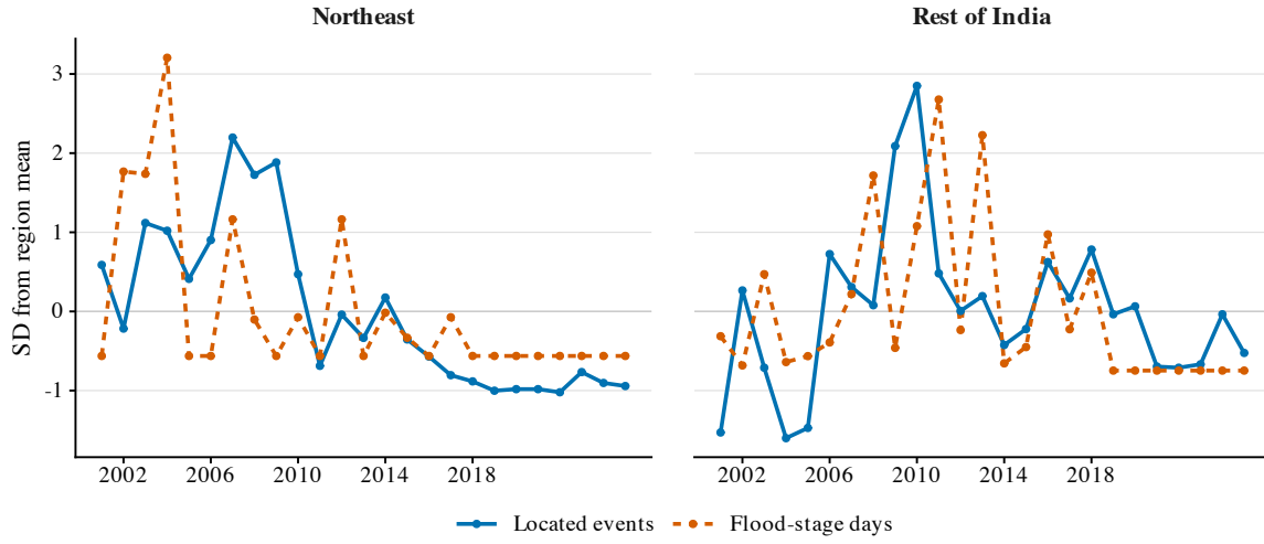
Figure E.15: Regional co-movement of conflict and routed flooding on the estimation sample, standardized within region (one axis; the two series have different units)
