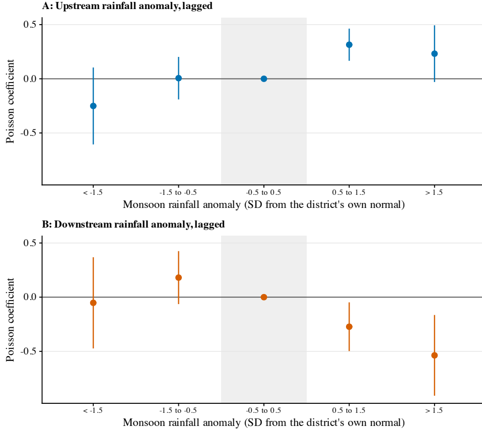
Figure D.2: The dose–response in upstream and downstream rainfall anomalies
