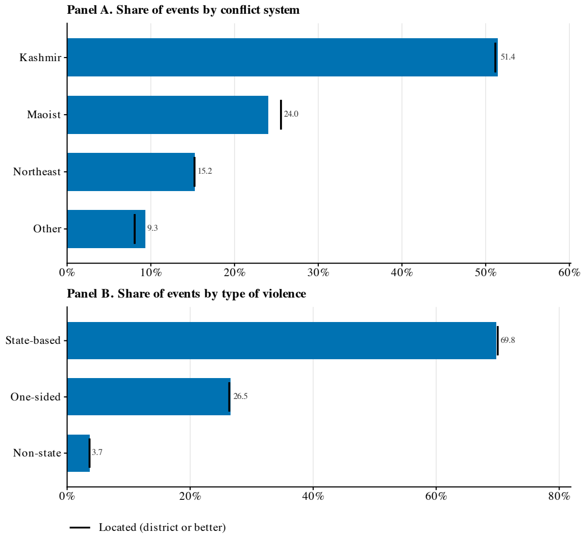
Figure E.2: Composition of UCDP events in India, 1989–2025
