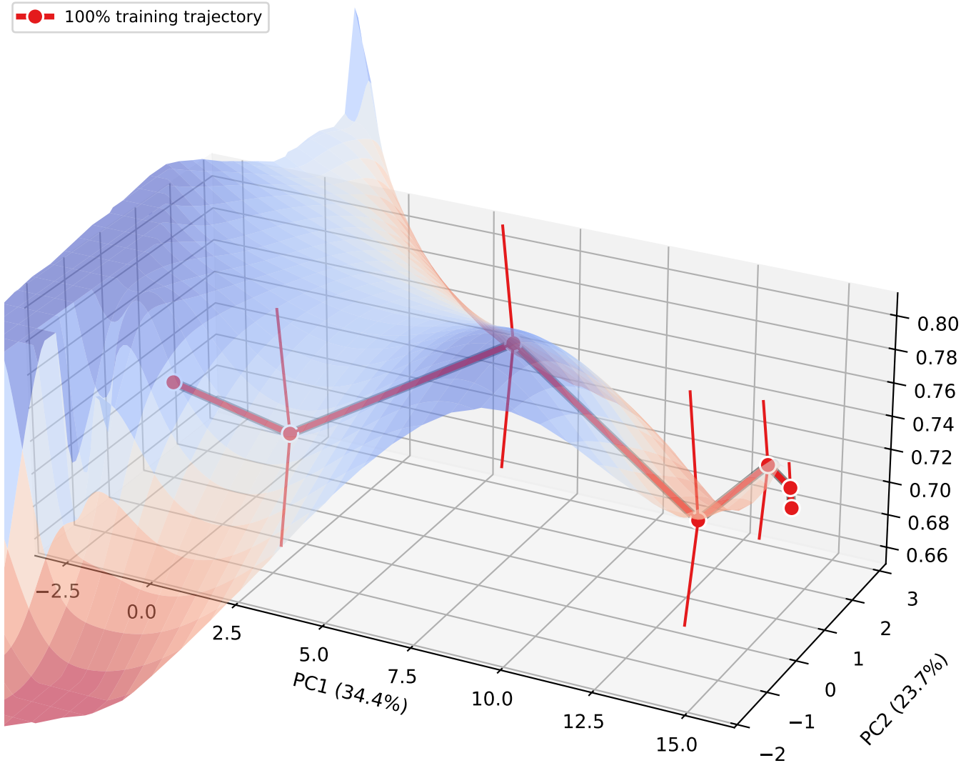
100% Training Trajectory on LoRA Loss Surface (loss surface fitted from all checkpoint losses)
