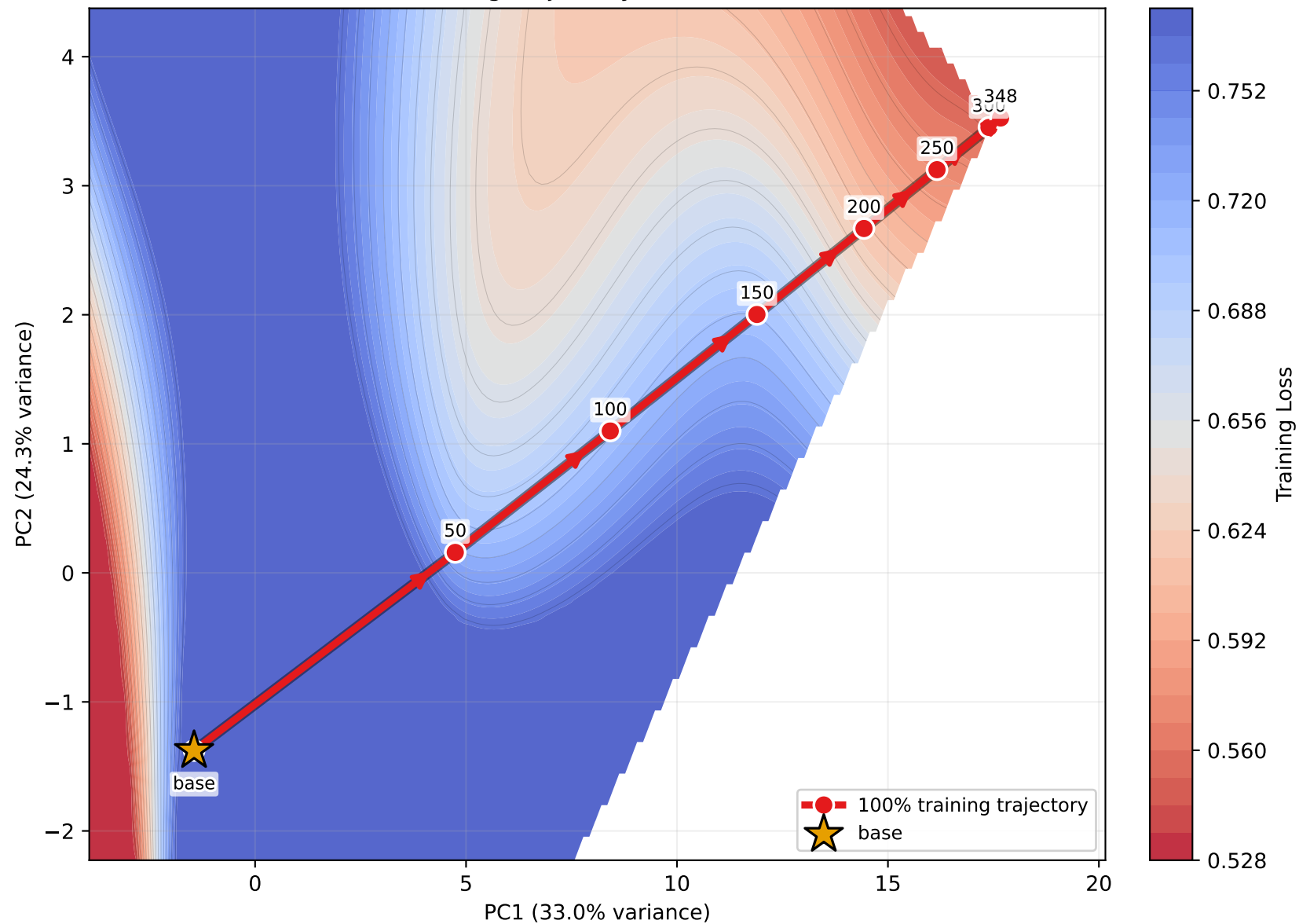
100% Fine-Tuning Trajectory on LoRA Loss Surface
