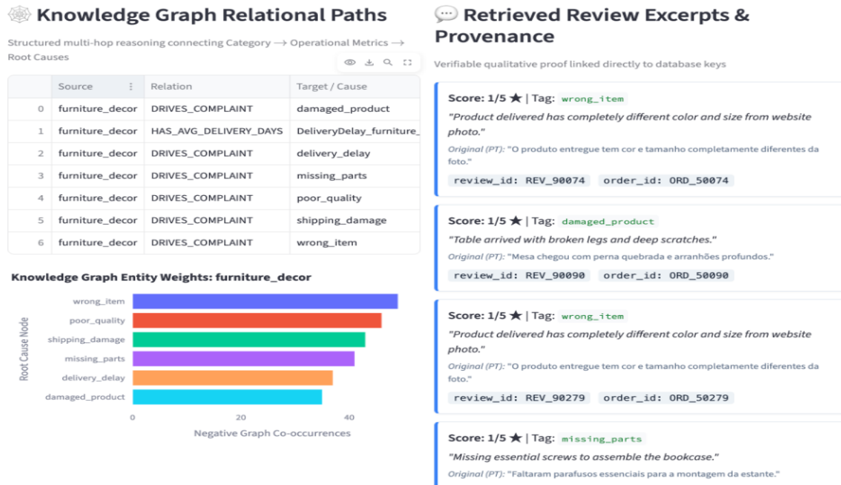
Figure 1 Caption: Live interface in Stage 3 Human–AI Co-Design showing (Left) NetworkX multi-hop entity traversal linking product categories to root-cause complaint weights, and (Right) qualitative customer review evidence cards with verified review_id and order_id provenance tags.
