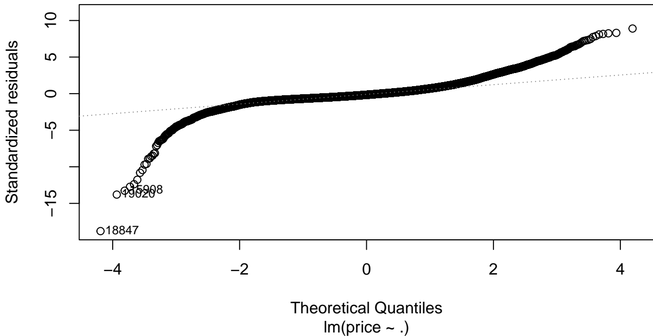
Q-Q Residuals
