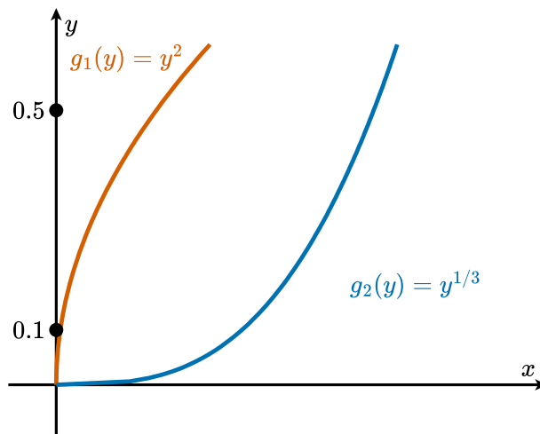
Figure 2.2.4 The graphs of x = g_1(y) = y^2 and x = g_2(y) = y^{1/3} . Shade the region R of Example 2.2.3 on them, and draw a typical strip.
