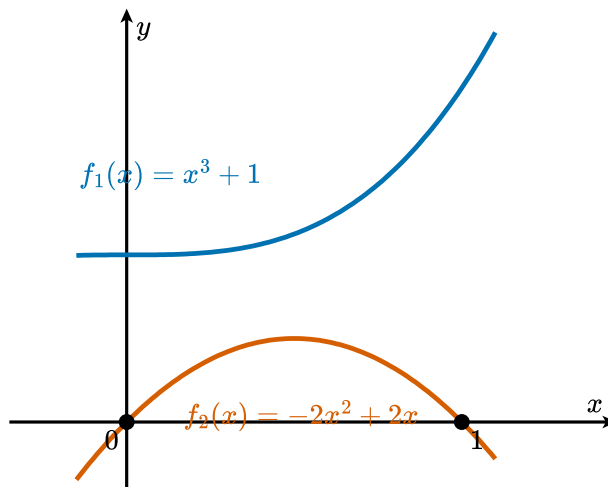
Figure 2.2.2 The graphs of f_1(x) = x^3 + 1 and f_2(x) = -2x^2 + 2x . Shade the region R of Example 2.2.1 on them, and draw a typical strip.
