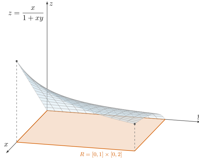
Figure 2.1.10 The surface z = \frac{x}{1 + xy} over the rectangle 0 \leq x \leq 1 , 0 \leq y \leq 2 . The double integral of Example 2.1.9 is the volume between this surface and the shaded base rectangle.
