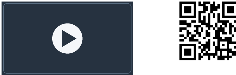
Figure 1.4.7 As the object moves through the field \mathbf{F} = \langle x, y \rangle along the trajectory, the work W = \int_C \mathbf{F} \cdot d\mathbf{r} accumulates moment by moment from the tangential component of the force.
