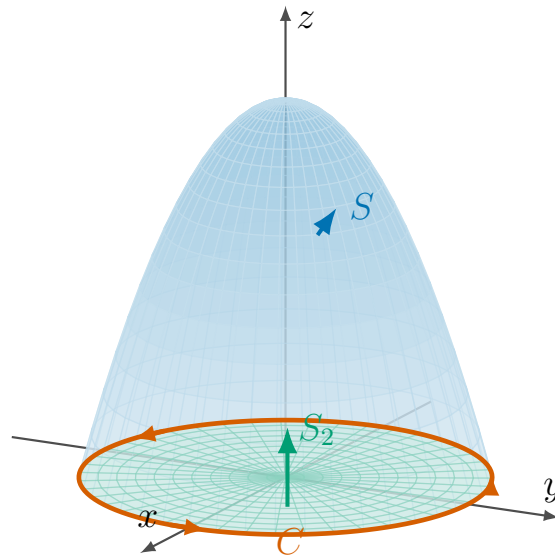
Figure 3.2.21 The two surfaces of Example 3.2.20 : the paraboloid S and the flat disk S_2 , which share the boundary circle C and carry orientations that give the extension questions bring out—the role played by the domain of the vector field.
