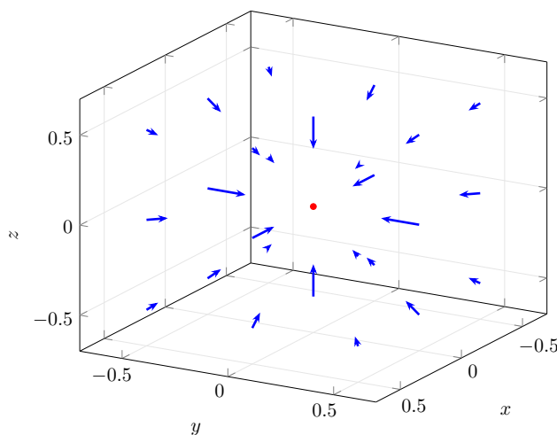
Figure 1.4.3 The field \mathbf{F} = -\mathbf{r} / \|\mathbf{r}\|^3 , which depends on x , y and z exactly as the gravitational force does. All arrows point toward the origin and shrink with the square of the distance.
