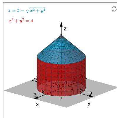
Figure 2.6.13 The solid of part (h).
