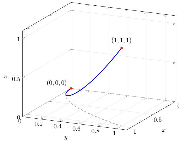
Figure 1.4.9 The twisted cubic \mathbf{r}(t) = \langle t, t^2, t^3 \rangle , 0 \leq t \leq 1 , from the origin to (1, 1, 1) . The dashed gray curve is its shadow on the plane z = 0 .
