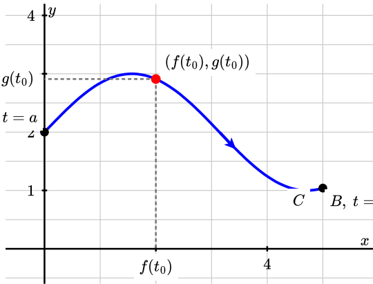
Figure 1.1.2 The trajectory of a moving point whose coordinates are given by the parametric equations x = f(t) , y = g(t) . At the instant t_0 the point is at (f(t_0), g(t_0)) .
