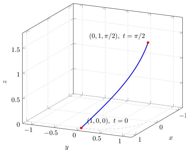
Figure 1.3.4 The helical wire \mathbf{r}(t) = \langle \cos t, \sin t, t \rangle for 0 \leq t \leq \pi/2 , from its bottom end (1, 0, 0) to its top end (0, 1, \pi/2) . The dashed gray curve is its shadow on the plane z = 0 .
