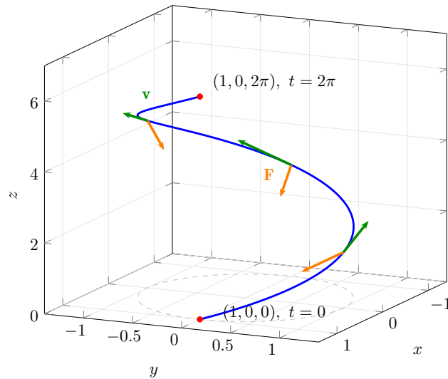
Figure 1.4.11 The helix \mathbf{r}(t) = \langle \cos t, \sin t, t \rangle , 0 \leq t \leq 2\pi , climbing through the field \mathbf{F} = -\mathbf{r}/\|\mathbf{r}\|^3 (orange arrows, direction only). At the same three points the velocity \mathbf{v} is drawn in green: at every one of them the field leans away from the direction of travel, which is why the work comes out negative.
