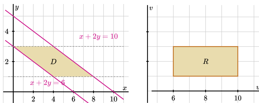
Figure 2.9.8 The parallelogram D between the lines x + 2y = 6 , x + 2y = 10 , y = 1 , and y = 3 (left), and the corresponding rectangle R in the uv -plane (right).
