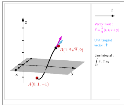
Figure 1.5.24 The same field \mathbf{F} = \frac{1}{3} \langle z, z, x+y \rangle and the same endpoints as in Figure 1.5.22, but now joined by the curve \mathbf{r}(t) = \langle \frac{\ln t}{\ln 2}, t^{3/2}, t \cos(\pi t) \rangle .
