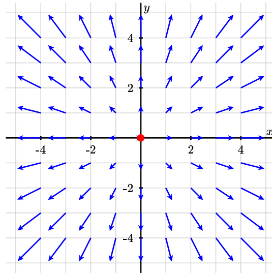
Figure 1.4.1 The vector field \mathbf{F}(x, y) = \langle x, y \rangle . Every arrow points directly away from the origin, and the arrows get longer as the distance from the origin grows.
