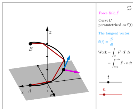
Figure 1.4.6 A point climbs the curve C while the force field \mathbf{F} and the velocity \mathbf{v} are drawn at its current position. The work is the accumulated \mathbf{F} \cdot \mathbf{v} , so the angle between the two arrows is what decides its sign.
