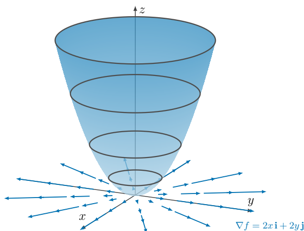
Figure 1.5.2 The surface z = f(x, y) = x^2 + y^2 together with its gradient field \nabla f = 2x \mathbf{i} + 2y \mathbf{j} , drawn in the xy -plane. The gradient vectors point radially away from the origin, the direction of steepest ascent, and grow longer as we move away from the origin.
