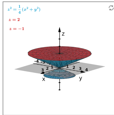
Figure 2.6.12 The solid of part (g).
