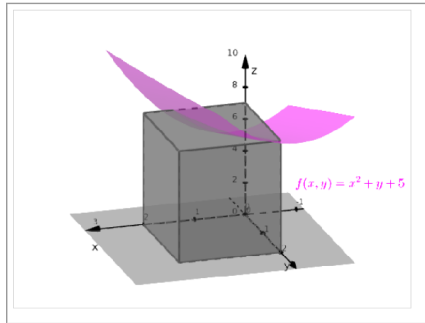
Figure 2.1.3 A first, very rough estimate of the volume under z = x^2 + y + 5 over the square R = [0, 2] \times [0, 2] : a single cuboid whose height is sampled at the center of the square. Turn the picture around: seen from any direction, part of the box sticks out above the surface and part of the volume under the surface is left uncovered.
