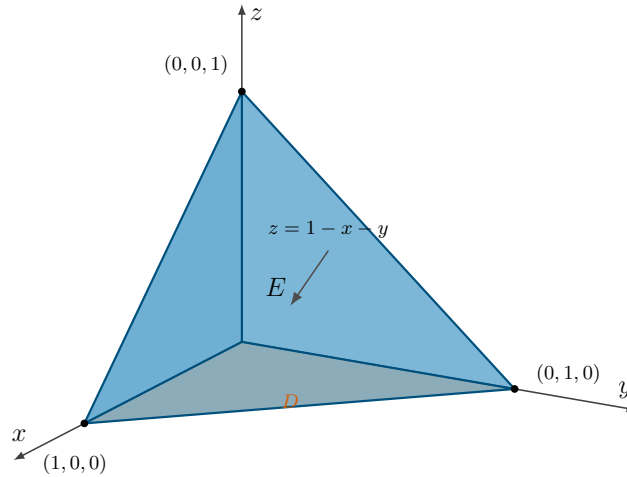
Figure 2.5.2 The tetrahedron E of Example 2.5.1 , bounded by the three coordinate planes and the plane z = 1 - x - y . Its projection into the xy -plane is the triangle D .
