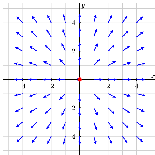
Figure 1.4.2 The normalized field \mathbf{F}(x, y) = \frac{\langle x, y \rangle}{\sqrt{x^2 + y^2}} : same directions as Figure 1.4.1, but every arrow has length one.
