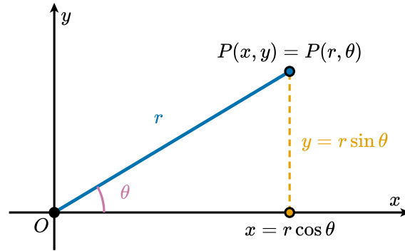
Figure 2.3.1 The same point P in both coordinate systems: in Cartesian coordinates it is P(x, y) , and in polar coordinates it is P(r, \theta) , where r is the directed distance from the origin O and \theta is the directed angle measured counterclockwise from the positive x -axis. The two are related by x = r \cos \theta and y = r \sin \theta .
