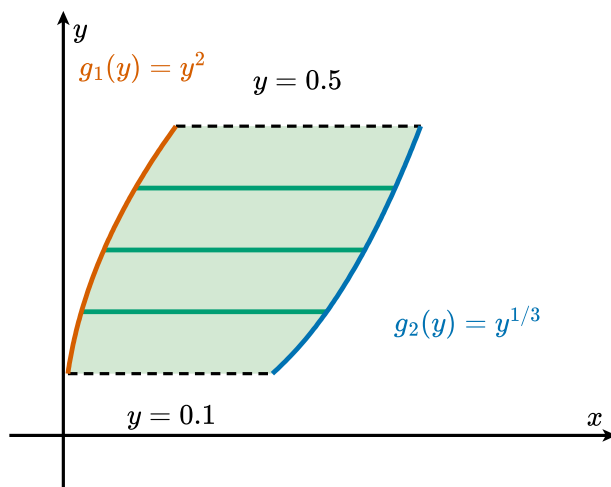
Figure 2.2.4 The region R of Example 2.2.3 , bounded on the left by g_1(y) = y^2 and on the right by g_2(y) = y^{1/3} for 0.1 \leq y \leq 0.5 . For each fixed y , the inner integral runs along a horizontal strip from the left curve to the right curve.
