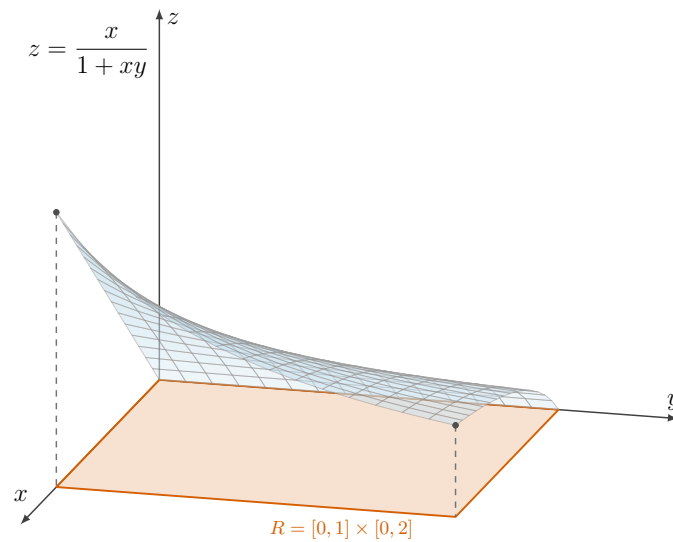
Figure 2.1.10 The surface z = \frac{x}{1+xy} over the rectangle 0 \leq x \leq 1 , 0 \leq y \leq 2 . The double integral of Example 2.1.9 is the volume between this surface and the shaded base rectangle.
