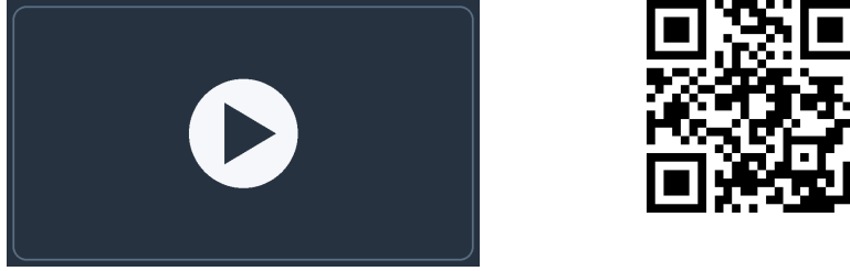
Figure 2.6.4 Animation of the cylindrical setup for Example 2.6.2 . A column at (r, \theta) runs from the paraboloid floor up to the plane z = 4 , and sweeps through the solid as \theta goes around the axis, illustrating dV = r \, dz \, dr \, d\theta .
