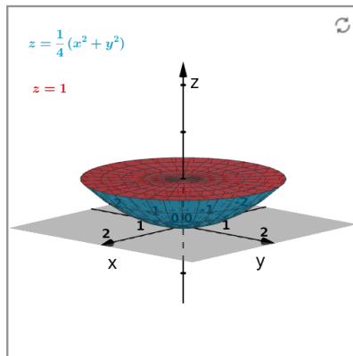
Figure 2.6.7 The solid of part (b).
