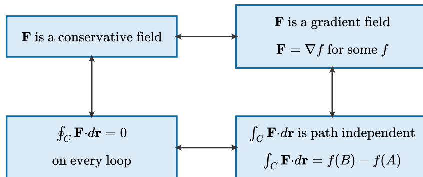
Figure 1.5.18 The four statements are equivalent. Each double arrow joins the middle of one box to the middle of the next, and may be read in either direction.
