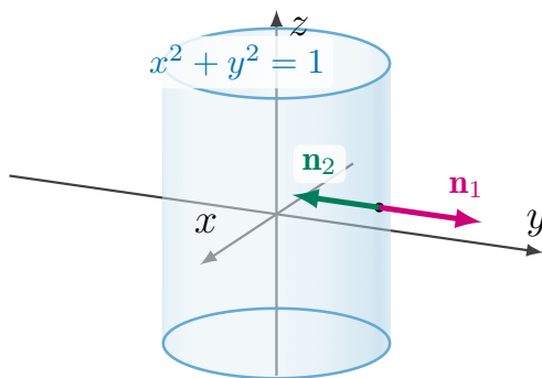
Figure 2.10.8 The cylinder x^2 + y^2 = 1 with its two possible orientations: \mathbf{n}_1 points away from the z -axis and \mathbf{n}_2 = -\mathbf{n}_1 points toward it.
