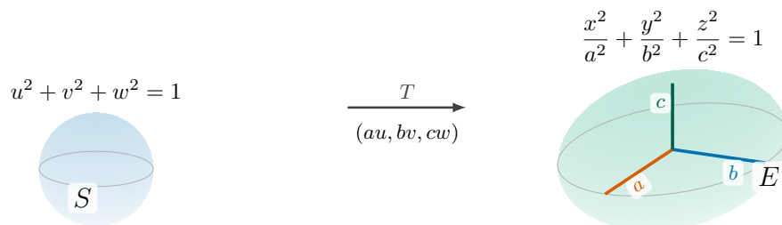
Figure 2.9.18 The transformation T(u, v, w) = (au, bv, cw) carries the unit ball S onto the solid ellipsoid E with semi-axes a , b , c .
