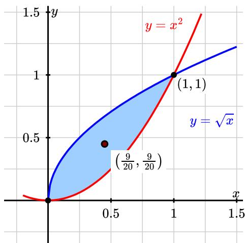
Figure 2.8.9 The region between y = \sqrt{x} (blue) and y = x^2 (red) over 0 \leq x \leq 1 , with its centroid marked.
