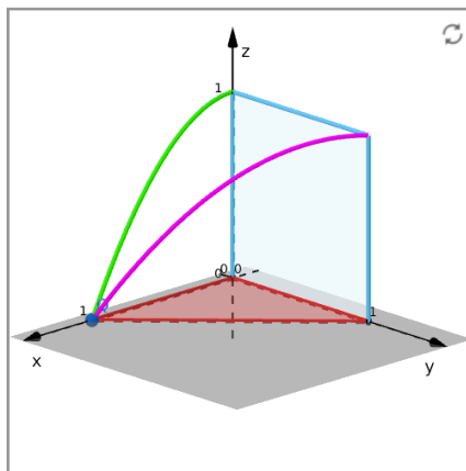
Figure 2.5.8 The solid R itself, to turn around: the triangular base x + y \leq 1 in the xy -plane, the surface z = 1 - x^2 that caps it, and the two edges of that cap above y = 0 and above y = 1 - x . The vertical plane slices the solid the way the innermost integral does.
