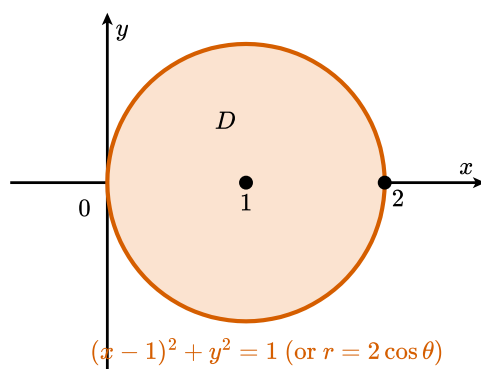
Figure 2.4.8 The base of the solid in Example 2.4.7 : the disk inside the cylinder x^2 + y^2 = 2x .
