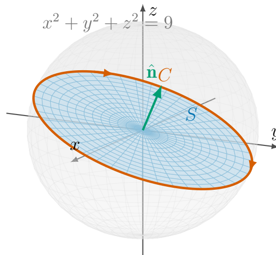
Figure 3.2.15 The curve of Example 3.2.14: the plane z = x cuts the sphere x^2 + y^2 + z^2 = 9 in the circle C , and the surface S is the flat disk that C bounds in that plane, tilted at 45^\circ .
