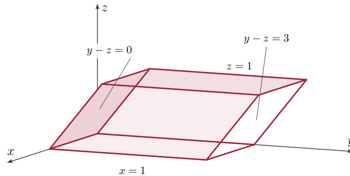
Figure 2.9.15 The parallelepiped bounded by the planes x = 0 , x = 1 , z = 0 , z = 1 , y - z = 0 , and y - z = 3 .
