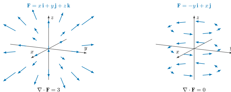
Figure 3.3.4 Left: the field x \mathbf{i} + y \mathbf{j} + z \mathbf{k} , which points radially outward. Right: the field -y \mathbf{i} + x \mathbf{j} , which rotates about the z -axis.
