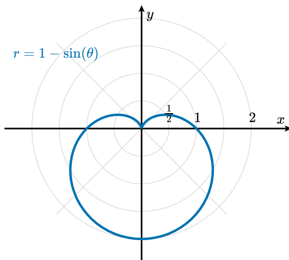
Figure 2.3.9 The cardioid r = 1 - \sin \theta , symmetric about the y -axis.
