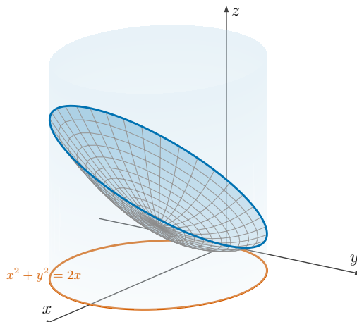
Figure 2.4.9 The solid of Example 2.4.7 : the region under the paraboloid z = x^2 + y^2 , above the xy -plane, and inside the cylinder x^2 + y^2 = 2x .
