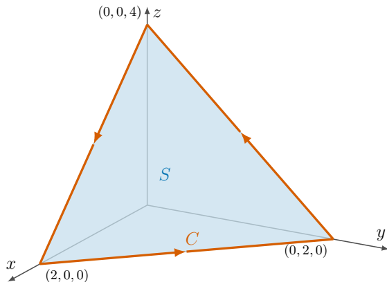
Figure 3.2.17 The oriented triangle of Example 3.2.16 : from (2, 0, 0) to (0, 2, 0) to (0, 0, 4) and back, bounding a piece of the plane \frac{x}{2} + \frac{y}{2} + \frac{z}{4} = 1 . The traversal is counterclockwise seen from above, pairing with the upward normal by the right-hand rule.
