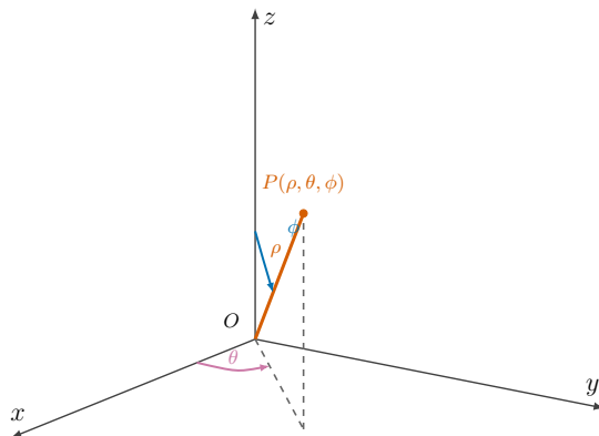
Figure 2.7.1 A point P(\rho, \theta, \phi) in spherical coordinates: \rho is the distance from the origin, \theta is the usual polar angle of the projection into the xy -plane, and \phi is the angle between \overrightarrow{OP} and the positive z -axis.
