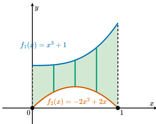
Figure 2.2.2 The region R of Example 2.2.1 , bounded above by f_1(x) = x^3 + 1 and below by f_2(x) = -2x^2 + 2x for 0 \leq x \leq 1 . For each fixed x , the inner integral runs along a vertical strip from the lower curve to the upper curve.
