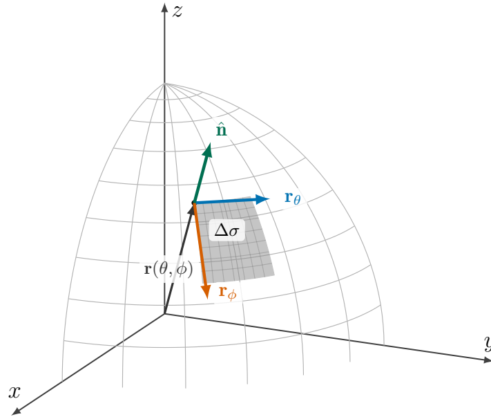
Figure 2.10.5 A small coordinate patch on the unit sphere. The tangent vectors \mathbf{r}_\theta and \mathbf{r}_\phi span the patch, and their cross product points along the outward normal \hat{\mathbf{n}} .
