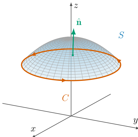
Figure 3.2.6 The orientation in Theorem 3.2.4 . The unit normal \hat{\mathbf{n}} and the direction of travel along the boundary C are related by the right-hand rule: with the thumb along \hat{\mathbf{n}} , the fingers curl the way C is traversed.
