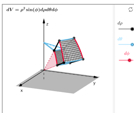
Figure 2.7.4 The spherical volume element (spherical wedge), with sliders for the three increments. Its three mutually perpendicular sides have lengths d\rho , \rho d\phi , and \rho \sin \phi d\theta .
