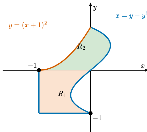
Figure 2.2.12 The region of Example 2.2.10 , split into R_1 (below the x -axis) and R_2 (above it). Both subregions share the right boundary x = y - y^3 ; the left boundary is the vertical line x = -1 for R_1 and the parabola y = (x + 1)^2 for R_2 .
