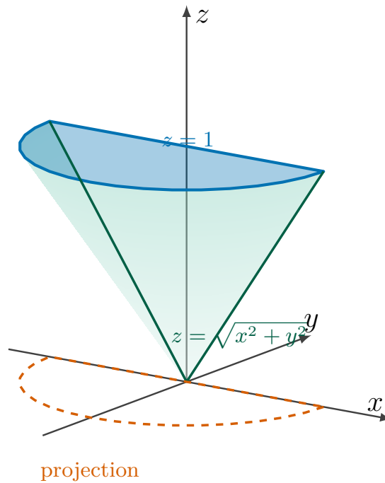
Figure 2.7.12 The solid of Example 2.7.10 : over the lower half disk, between the cone z = \sqrt{x^2 + y^2} and the plane z = 1 .
