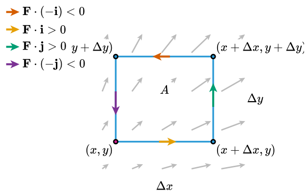
Figure 3.1.6 The counterclockwise circulation of \mathbf{F} = M\mathbf{i} + N\mathbf{j} around the rectangle: along each side we take the component of \mathbf{F} in the direction of travel. Each side's component is drawn in its own color, and the legend gives the dot product it represents.
