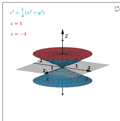
Figure 2.6.10 The solid of part (e).
