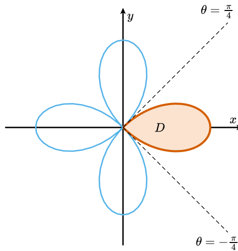
Figure 2.4.6 The four-leaved rose r = \cos(2\theta) , with one loop D shaded. Which angles sweep it out?
