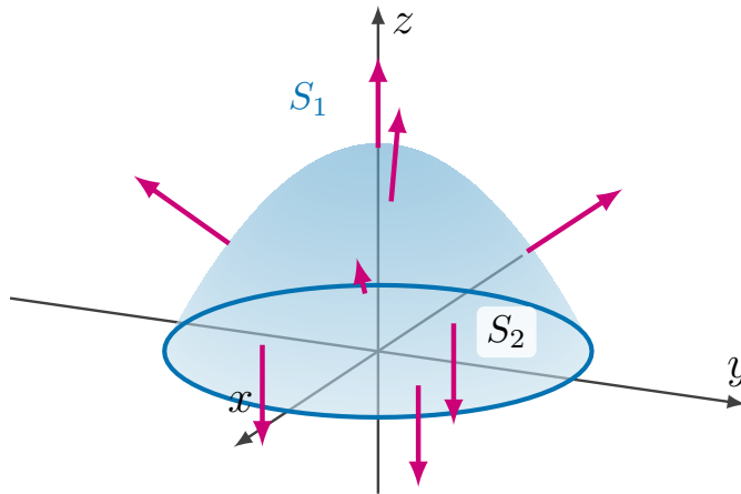
Figure 2.10.15 The boundary S of the solid enclosed by z = 1 - x^2 - y^2 and z = 0 : the cap S_1 with upward-and-outward normals, and the disk S_2 with downward normals.
