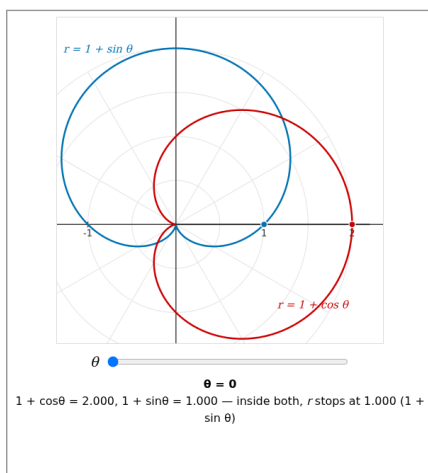
Figure 2.4.17 Figure (4): the cardioids r = 1 + \cos \theta and r = 1 + \sin \theta . Drag the slider to turn the ray of angle \theta ; the overlap is what the ray reaches before it leaves the first of the two curves.
