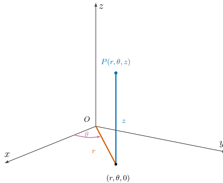
Figure 2.6.1 A point P(r, \theta, z) in cylindrical coordinates: (r, \theta) are the polar coordinates of its projection (r, \theta, 0) into the xy -plane, and z is its usual height.
