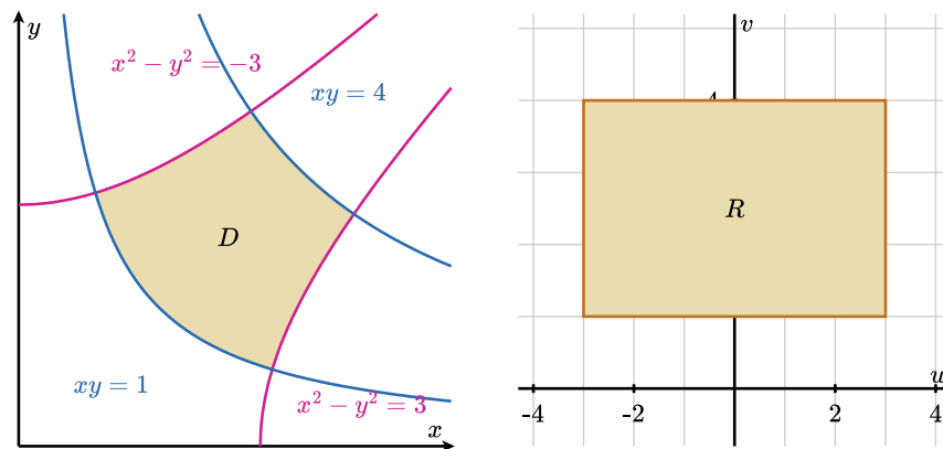
Figure 2.9.11 The region D bounded by the hyperbolas x^2 - y^2 = \pm 3 and xy = 1 , xy = 4 (left) corresponds to a rectangle R in the uv -plane (right).
