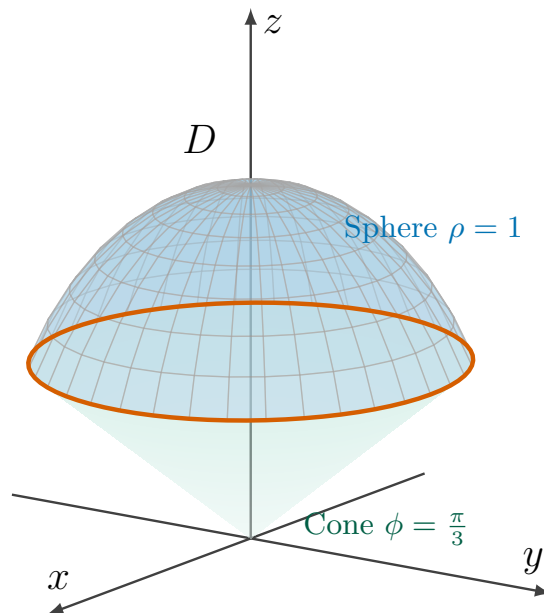
Figure 2.7.6 The “ice cream cone” of Example 2.7.5 : the region inside the sphere \rho = 1 and above the cone \phi = \pi/3 .
