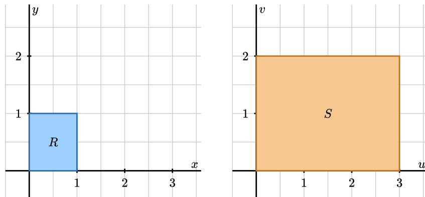
Figure 2.9.5 The rectangle S in the uv -plane (right) and its image, the unit square R , in the xy -plane (left) under T(u, v) = (u/3, v/2) .
