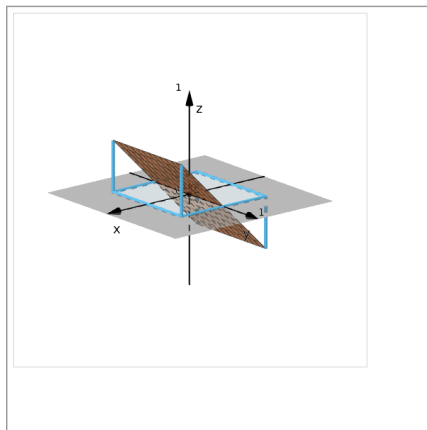
Figure 2.1.14 Figure (2): the plane z = x over the square R , together with R itself in the xy -plane. Half of the plane lies above R and half below.
