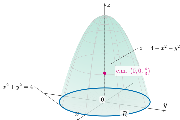
Figure 2.8.5 The solid of constant density bounded by the paraboloid z = 4 - x^2 - y^2 and the disk R: x^2 + y^2 \leq 4 in the plane z = 0 . The center of mass sits on the axis of symmetry.
