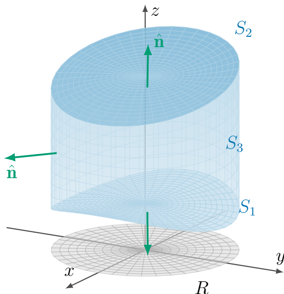
Figure 3.3.6 The solid of Step 1 of the proof of Theorem 3.3.5 : a solid D that is simple in the z -direction. Its boundary is the cap S_2 where z = u_2(x, y) , the floor S_1 where z = u_1(x, y) , and the vertical wall S_3 over the boundary of the shadow R . On the wall \mathbf{k} is tangent, so \mathbf{k} \cdot \hat{\mathbf{n}} = 0 .
