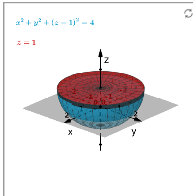
Figure 2.6.9 The solid of part (d).
