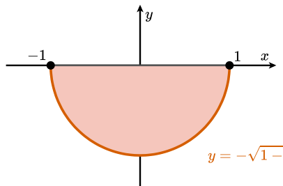
Figure 2.7.11 The xy -projection of the solid in Example 2.7.10 : the lower half of the unit disk.
