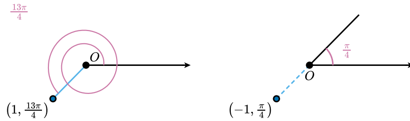
Figure 2.3.4 Two of the many polar representations of the same point. On the left, (1, \frac{13\pi}{4}) : the angle wraps around once before landing on the third-quadrant ray. On the right, (-1, \frac{\pi}{4}) : the negative r places the point on the ray opposite to the angle \frac{\pi}{4} . The pairs (1, \frac{5\pi}{4}) and (1, -\frac{3\pi}{4}) give the same point too.
