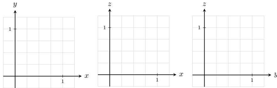
Figure 2.5.7 Sketch the three projections of the solid R . Left: into the xy -plane (order dz dx dy ). Middle: into the xz -plane (order dy dx dz ). Right: into the yz -plane (order dx dy dz ); mark the curve that splits it into R_1 and R_2 .
