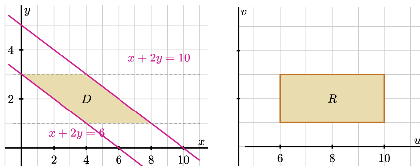
Figure 2.9.8 The parallelogram D between the lines x + 2y = 6 , x + 2y = 10 , y = 1 , and y = 3 (left), and the corresponding rectangle R in the uv -plane (right).
