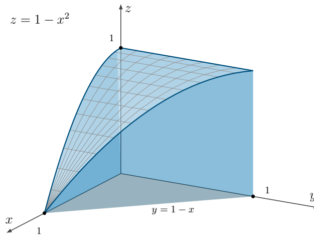
Figure 2.5.6 The solid R of Example 2.5.5, bounded by the parabolic cylinder z = 1 - x^2 , the vertical plane y = 1 - x , and the coordinate planes.
