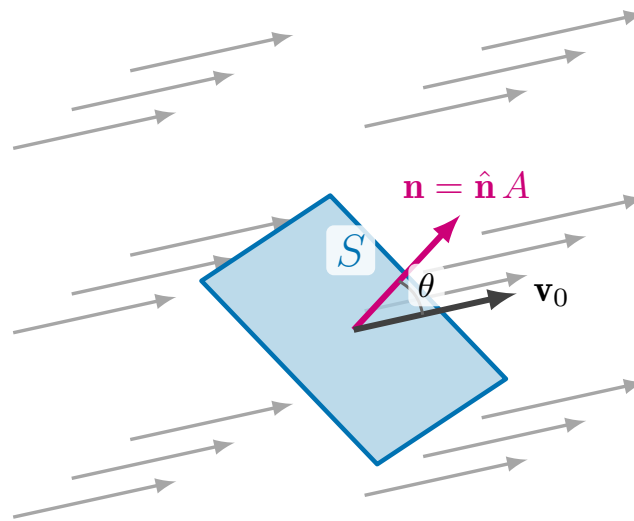
Figure 2.10.1 A tilted plate S of area A in a uniform flow \mathbf{v}_0 . Only the component of \mathbf{v}_0 along the normal \mathbf{n} carries fluid through the plate.
