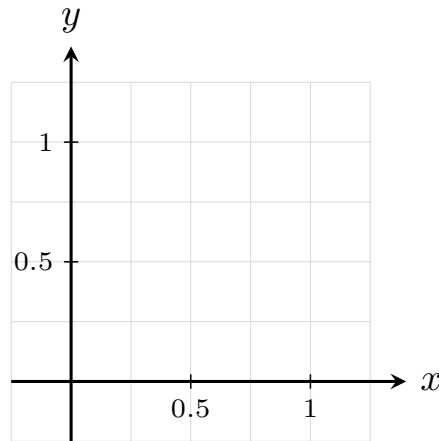
Figure 2.5.3 Sketch the projection D of the tetrahedron into the xy -plane. At a fixed (x, y) in D , the inner z -integration runs up a vertical arrow from the floor to the plane.
