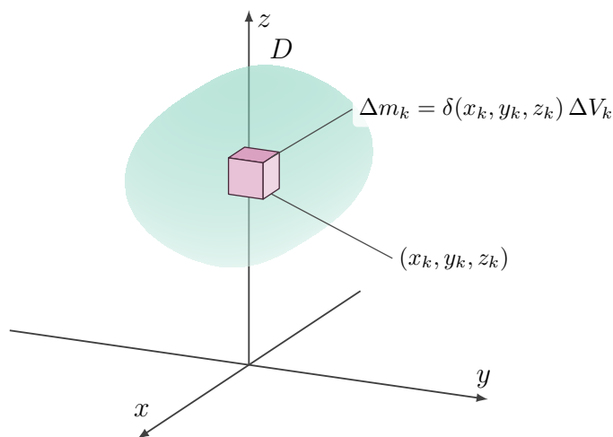
Figure 2.8.2 A solid region D with a small box around the point (x_k, y_k, z_k) . The box has volume \Delta V_k and mass \Delta m_k = \delta(x_k, y_k, z_k) \Delta V_k .
