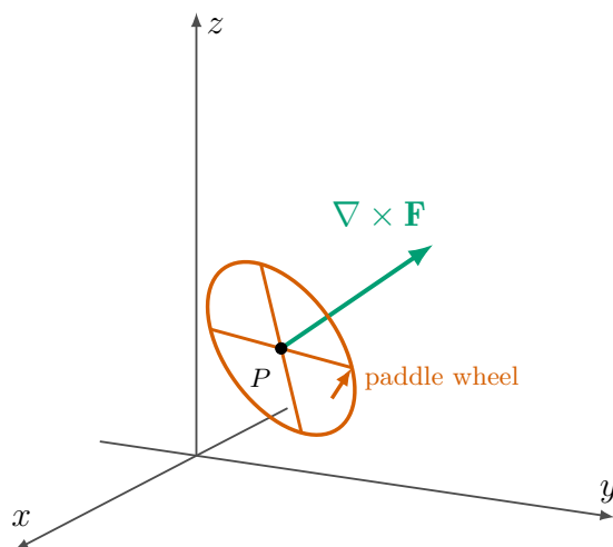
Figure 3.2.3 The curl of Example 3.2.2 at the point P(1, 1, 1) . The curl is the axis of the paddle wheel: put the wheel in the plane perpendicular to it and the field turns the wheel the way the arrow shows. Compare the arrow with the vector you computed.
