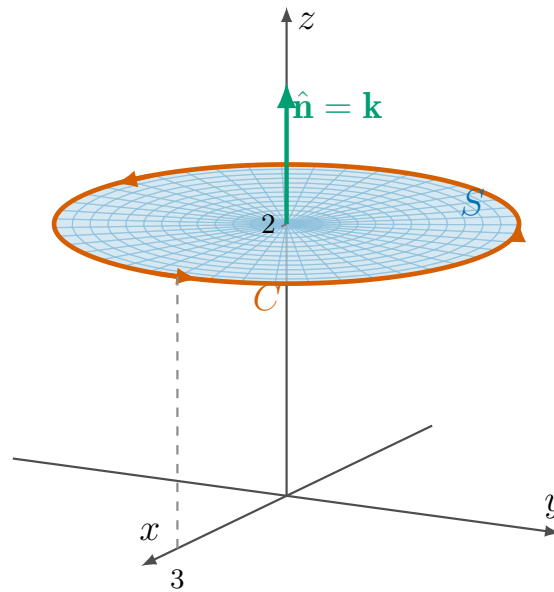
Figure 3.2.13 The cheapest surface for Example 3.2.12: the flat disk S of radius 3 in the plane z = 2 , whose boundary is the given circle C .
