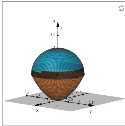
Figure 2.5.15 Figure (3): the region of integration E , bounded below by the paraboloid z = x^2 + y^2 and above by z = 1 + \sqrt{1 - x^2 - y^2} . The two surfaces meet over the circle x^2 + y^2 = 1 .
