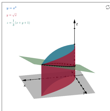
Figure 2.5.17 Figure (4): the solid bounded by the cylinders y = x^2 and y = \sqrt{x} , the plane z = 0 , and the plane z = \frac{1}{3}(x + y + 1) , whose two edges are drawn on the walls.
