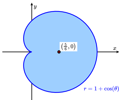
Figure 2.8.12 The cardioid r = 1 + \cos(\theta) . The region is symmetric about the x -axis and its centroid is marked in maroon.
