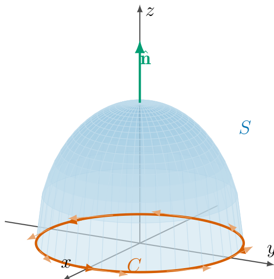
Figure 3.2.9 The surface and boundary of Example 3.2.8 : the upper hemisphere S of x^2 + y^2 + z^2 = 1 with its upward normal, and the unit circle C in the xy -plane, counterclockwise seen from above. The field \mathbf{F} = -y\mathbf{i} + x\mathbf{j} runs tangent to C all the way round, which is why the circulation is as large as it can be.
