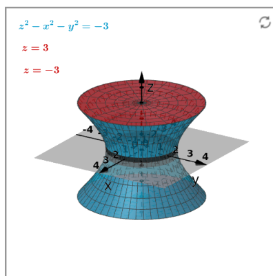
Figure 2.6.11 The solid of part (f).
