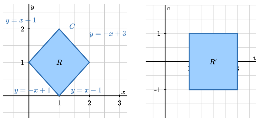
Figure 3.1.20 The square C with vertices (1,0) , (2,1) , (1,2) , (0,1) (left) and the corresponding rectangle in the uv -plane (right).
