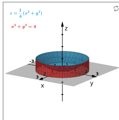
Figure 2.6.8 The solid of part (c).
