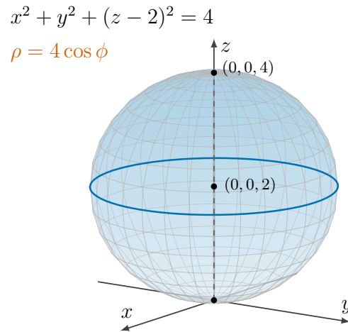
Figure 2.7.9 The sphere x^2 + y^2 + (z - 2)^2 = 4 of Example 2.7.8 . It sits on the xy -plane, touching the origin.
