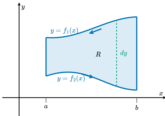
Figure 3.1.13 Step 1 of the proof of Theorem 3.1.12 : a region R cut by vertical lines, with f_2(x) \leq y \leq f_1(x) for a \leq x \leq b . Counterclockwise, the bottom curve is travelled left to right and the top curve right to left; on the two vertical sides dx = 0 , so they contribute nothing to \oint_C M dx .
