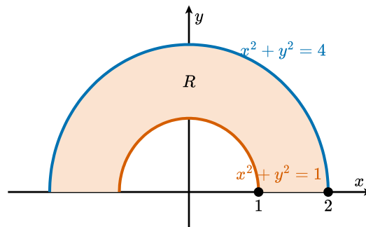
Figure 2.4.4 The region of Example 2.4.3 : the upper half of the annulus between the circles x^2 + y^2 = 1 and x^2 + y^2 = 4 .
