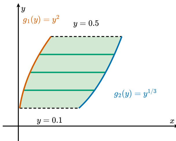
Figure 2.2.4 The region R of Example 2.2.3 , bounded on the left by g_1(y) = y^2 and on the right by g_2(y) = y^{1/3} for 0.1 \leq y \leq 0.5 . For each fixed y , the inner integral runs along a horizontal strip from the left curve to the right curve.
