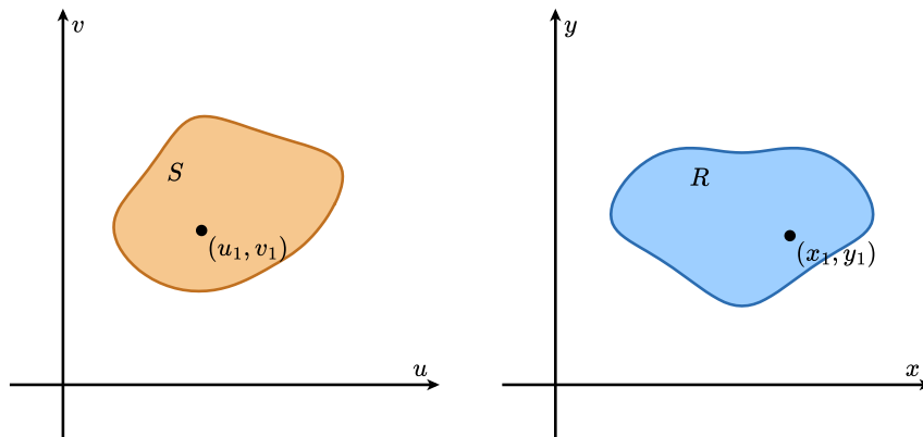
Figure 2.9.1 The transformation T(u, v) = (f(u, v), g(u, v)) carries the region S in the uv -plane onto the region R in the xy -plane; the inverse T^{-1} carries R back onto S . The point (u_1, v_1) is sent to the point (x_1, y_1) .
