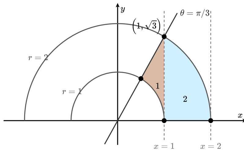
Figure 2.4.12 Figure (1): two regions between the circles r = 1 and r = 2 , cut apart by the vertical line x = 1 and swept by the angles 0 \leq \theta \leq \pi/3 . The line y = \sqrt{3}x is the ray \theta = \pi/3 , and it meets x = 1 exactly on the outer circle.
