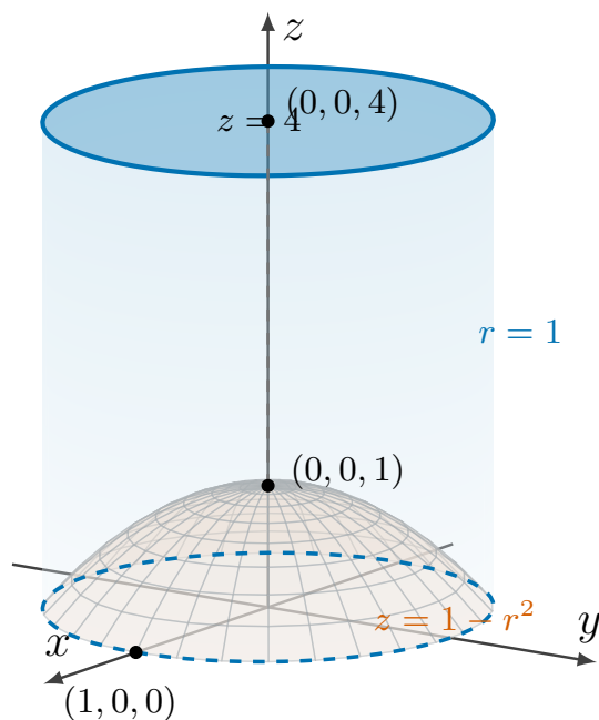
Figure 2.6.3 The solid of Example 2.6.2 : inside the cylinder x^2 + y^2 = 1 , above the paraboloid z = 1 - x^2 - y^2 , and below the plane z = 4 .
