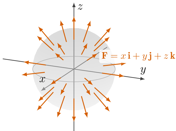
Figure 3.3.9 The radial field \mathbf{F} = x\mathbf{i} + y\mathbf{j} + z\mathbf{k} crossing the unit sphere. Compare with the outward flux you found.
