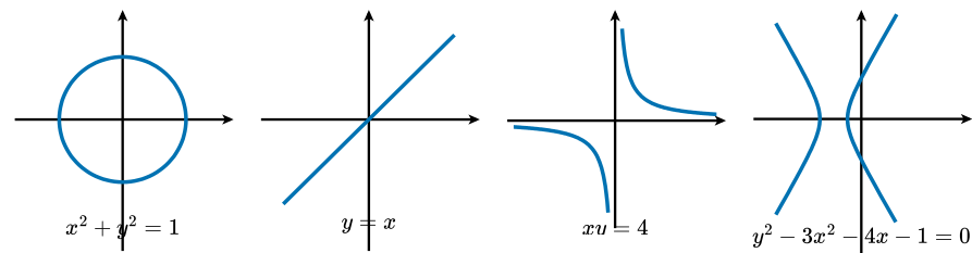
Figure 2.3.6 The four curves of Example 2.3.5 , from left to right: parts A, B, C and D. Match each with the Cartesian equation you found. Next, we would like to learn about graphing polar equations. We will begin by analyzing symmetries of polar equations.
