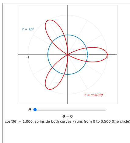
Figure 2.4.14 Figure (2): the rose r = \cos(3\theta) and the circle r = \frac{1}{2} . Drag the slider to turn the ray of angle \theta ; the dots mark where that ray crosses each curve, which is what fixes the limits of r .
