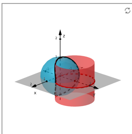
Figure 2.2.14 Figure (4): the sphere x^2 + y^2 + z^2 = 1 and the cylinder x^2 + (y - 1)^2 = 1 . Use this graph to find the region of integration and the integrand. The wall of the cylinder runs straight down to the xy -plane, where the red circle outlines the region of integration.
