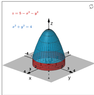
Figure 2.6.6 The solid of part (a).
