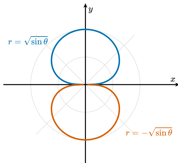
Figure 2.3.11 The graph of r^2 = \sin \theta , made of the branch r = \sqrt{\sin \theta} (in blue) and the branch r = -\sqrt{\sin \theta} (in vermilion). Since replacing r by -r does not change the equation, the graph is symmetric about the origin.
