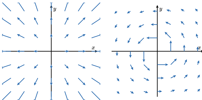
Figure 3.1.5 Left: the field 2x\mathbf{i} + 2y\mathbf{j} , which flows away from the origin. Right: the field \frac{-y\mathbf{i} + x\mathbf{j}}{x^2 + y^2} , which circulates around the origin. Compare with the divergences you computed.
