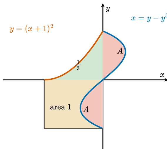
Figure 2.2.11 Method 2: since x = y - y^3 is odd, the piece A removed from the unit square (below the x -axis) is congruent to the piece A added to the right of the y -axis (above it). The area is therefore the area of the square plus the area of the green strip between the parabola y = (x + 1)^2 and the y -axis.
