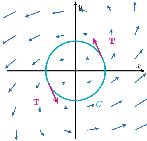
Figure 3.1.17 The vector field \mathbf{F}(x, y) = (x - y)\mathbf{i} + x\mathbf{j} and the unit circle C . The field has a positive (counterclockwise) circulation around C .
