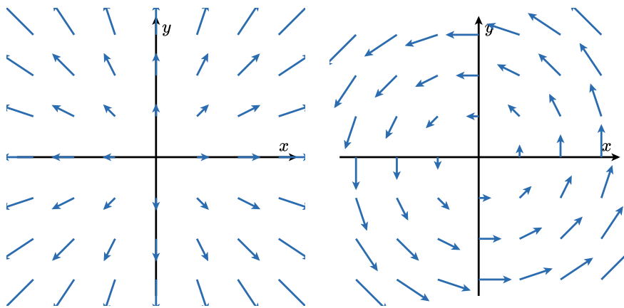
Figure 3.1.10 Left: the radial field 2x\mathbf{i} + 2y\mathbf{j} . Right: the rotational field -2y\mathbf{i} + 2x\mathbf{j} . Compare with the curls you computed: would a paddle wheel spin in each?
