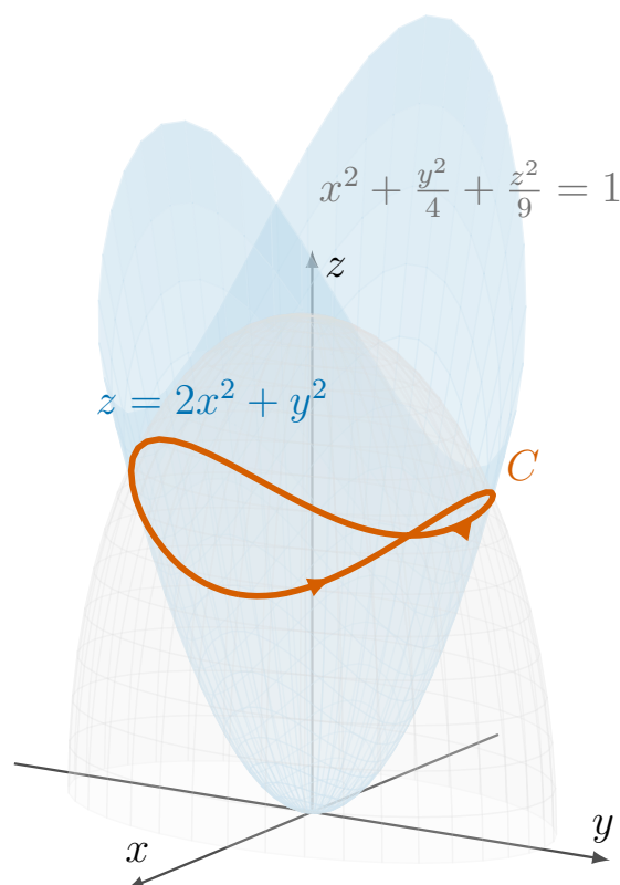
Figure 3.2.19 The curve of Example 3.2.18 : the paraboloid z = 2x^2 + y^2 meets the ellipsoid x^2 + \frac{y^2}{4} + \frac{z^2}{9} = 1 in a warped loop C . Does anything about its shape matter?
