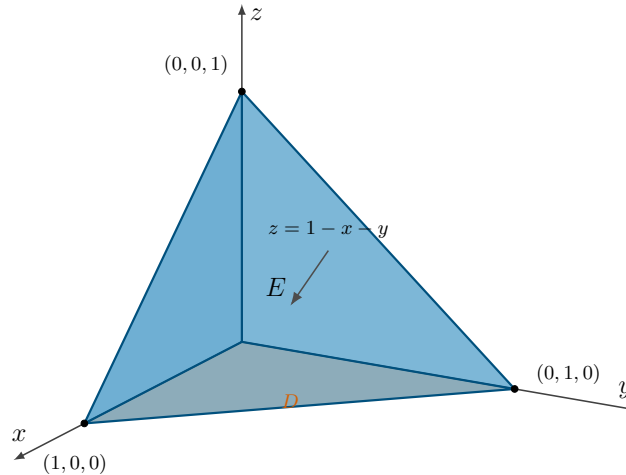
Figure 2.5.2 The tetrahedron E of Example 2.5.1 , bounded by the three coordinate planes and the plane z = 1 - x - y . Its projection into the xy -plane is the triangle D .
