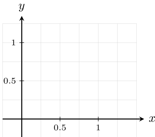
Figure 2.2.8 Sketch the region of integration for Example 2.2.6 : the base of the tetrahedron in the xy -plane, with the lines that bound it and a typical vertical strip.
