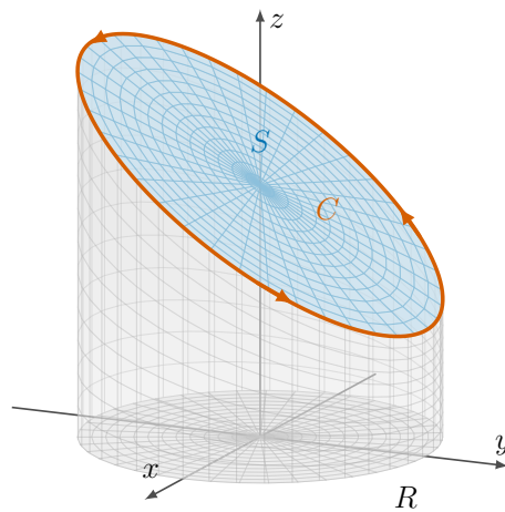
Figure 3.2.11 The curve C of Example 3.2.10 : the plane y + z = 2 cuts the cylinder x^2 + y^2 = 1 in an ellipse. The shaded elliptical region is the surface S used in the solution, and its shadow is the unit disk R .
