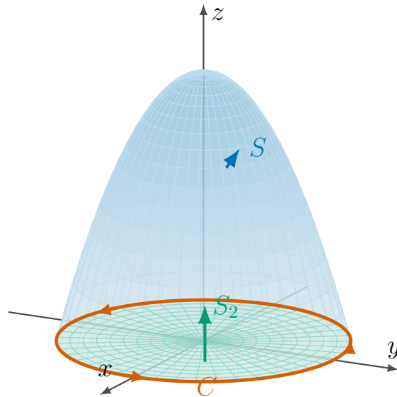
Figure 3.2.21 The two surfaces of Example 3.2.20 : the paraboloid S and the flat disk S_2 , which share the boundary circle C and carry orientations that give the same direction on it. By (3.2.3) the flux of the curl through them is the same, and the disk is the easy one.
