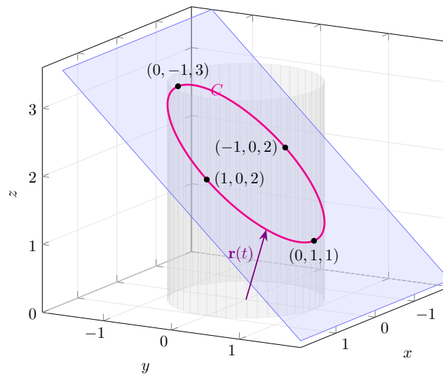
Figure 1.1.17 The cylinder x^2 + y^2 = 1 , the plane y + z = 2 , and the ellipse C in which they meet. The violet arrow is the position vector \mathbf{r}(t) of your parametrization at t = \pi/4 .
