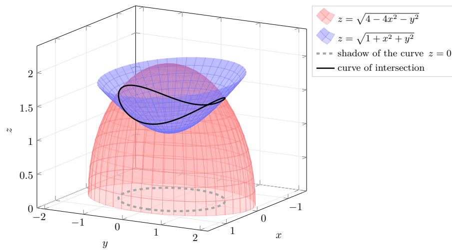
Figure 1.1.19 The upper sheet of z = \sqrt{1 + x^2 + y^2} (blue) and the dome z = \sqrt{4 - 4x^2 - y^2} (red) meet along the closed curve drawn in black. Its shadow in the plane z = 0 is the dashed ellipse; compare it with the equation you found.
