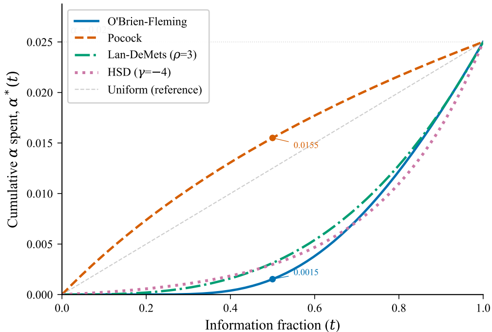
Figure 1. Alpha-spending functions for group-sequential designs
