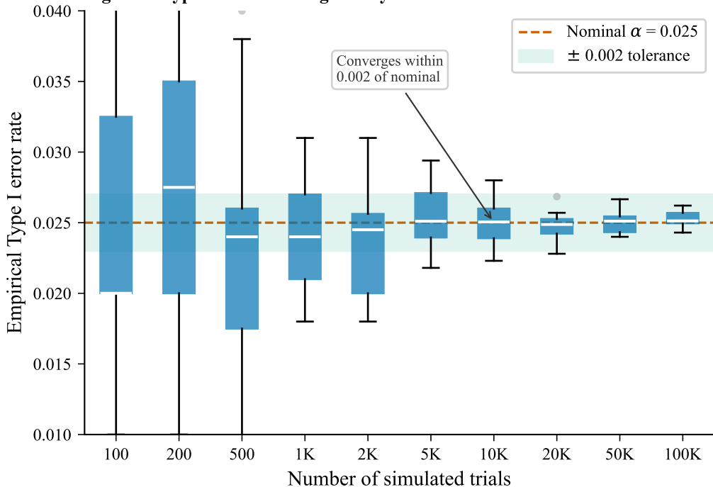
Figure 2. Type I error convergence by simulation count
