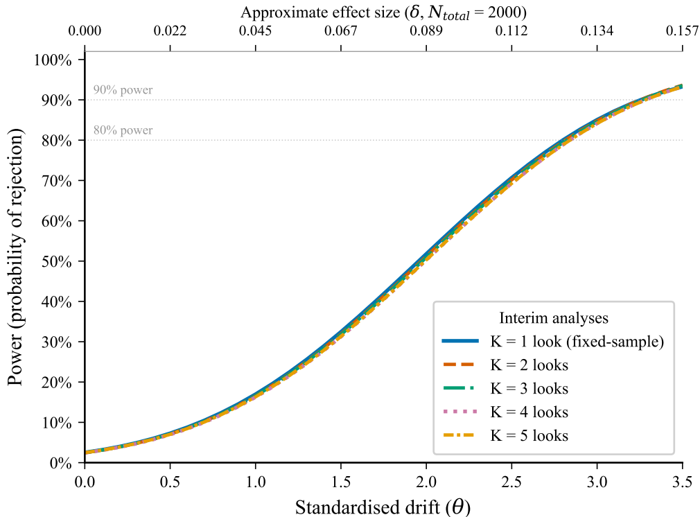
Figure 3. Power by effect size and number of interim analyses (O'Brien-Fleming spending, equally spaced looks)
