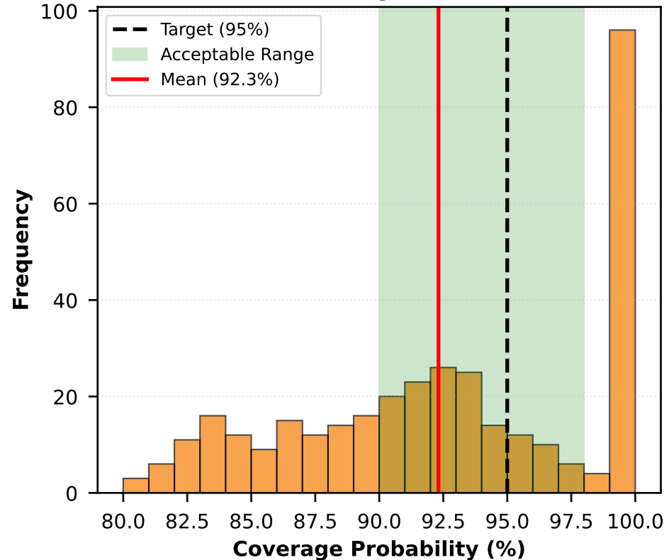
Two-Stage Fixed
