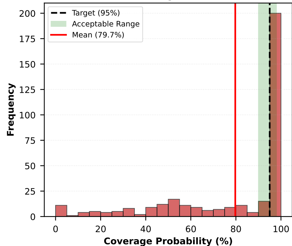
One-Stage REML
