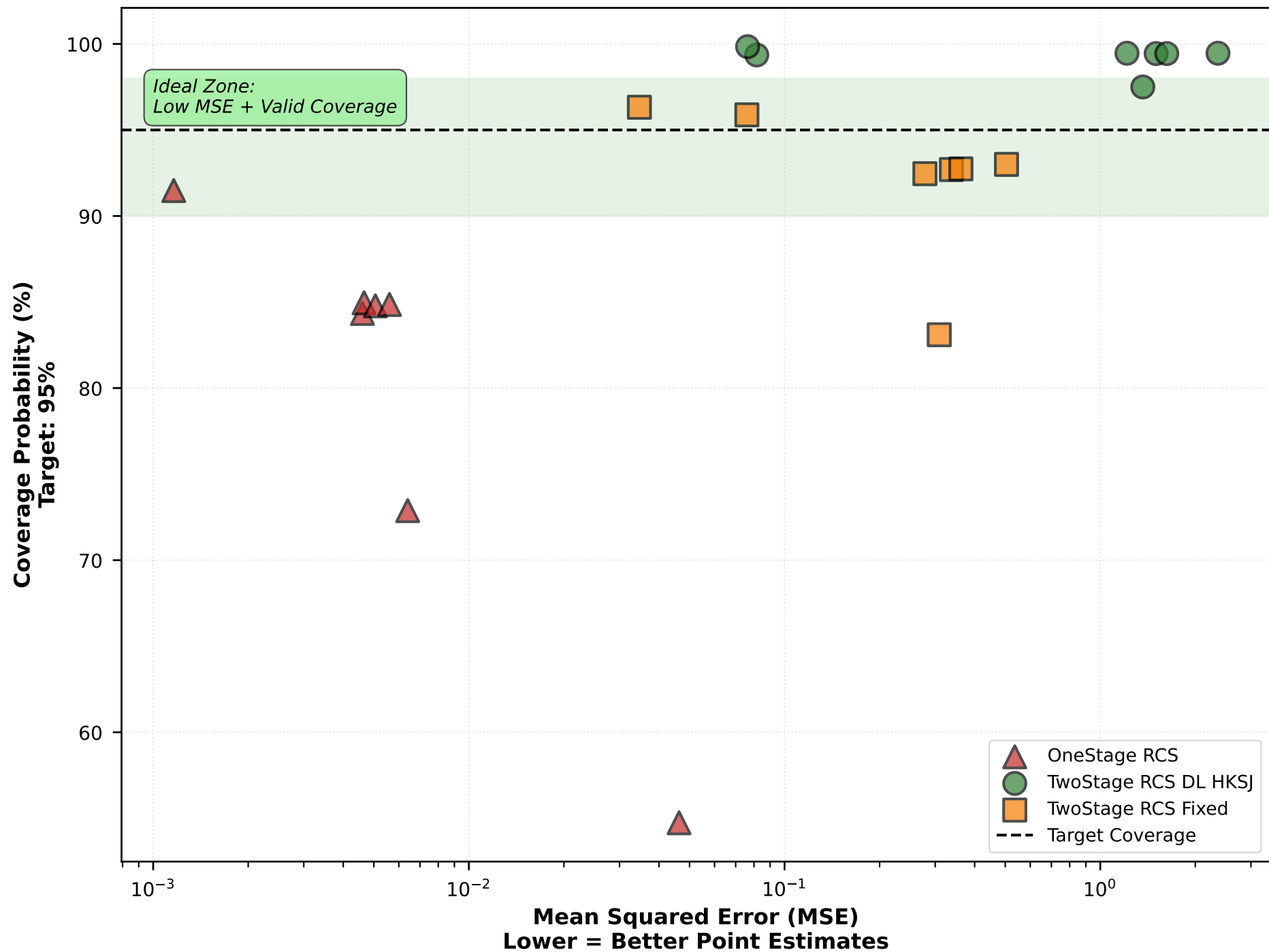
MSE vs. Coverage Tradeoff by Method and Scenario
