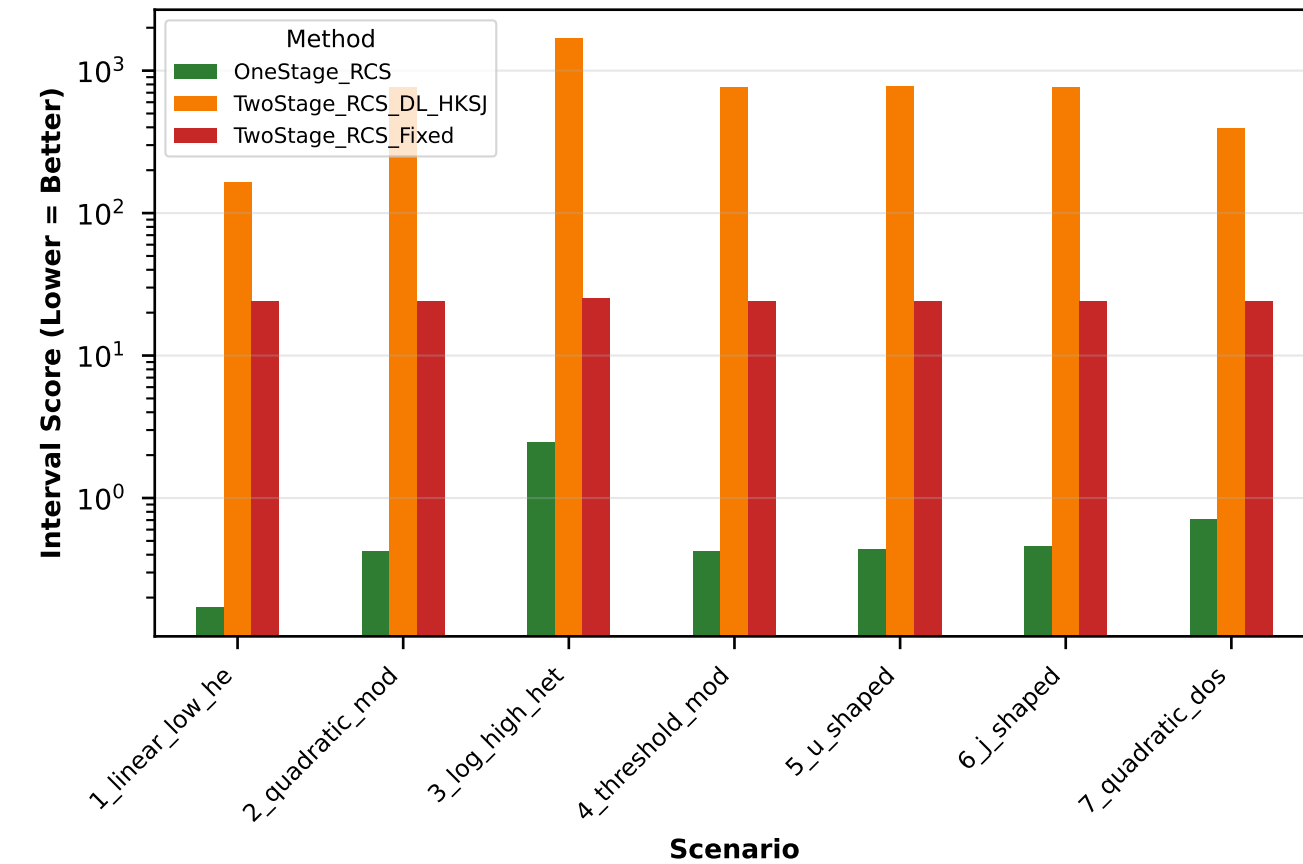
C. Total Interval Score by Scenario
