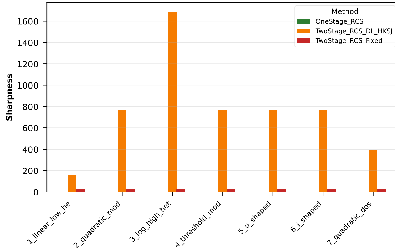
A. Sharpness (Interval Width) by Scenario
