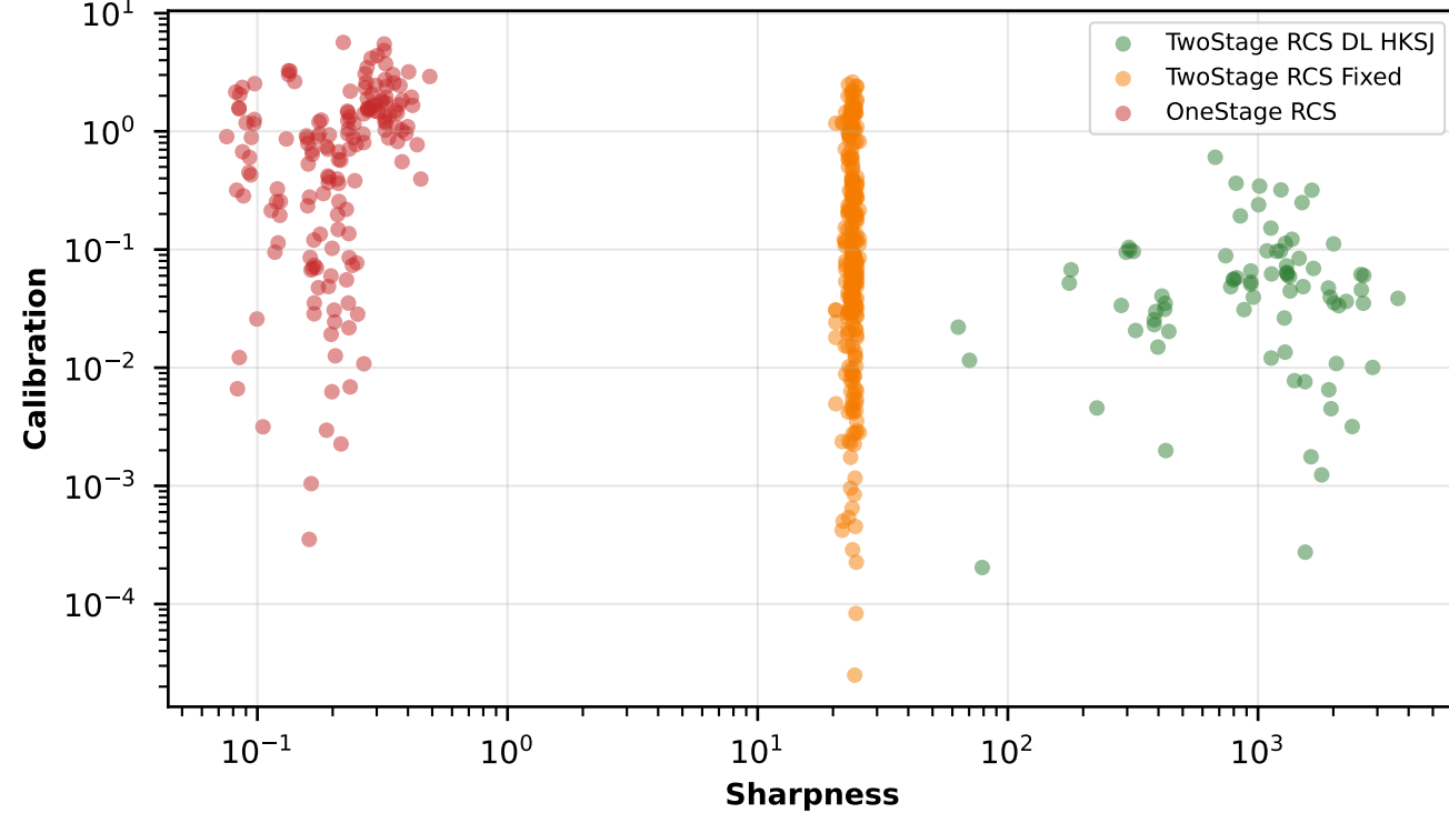
D. Sharpness vs. Calibration (All Simulations)
