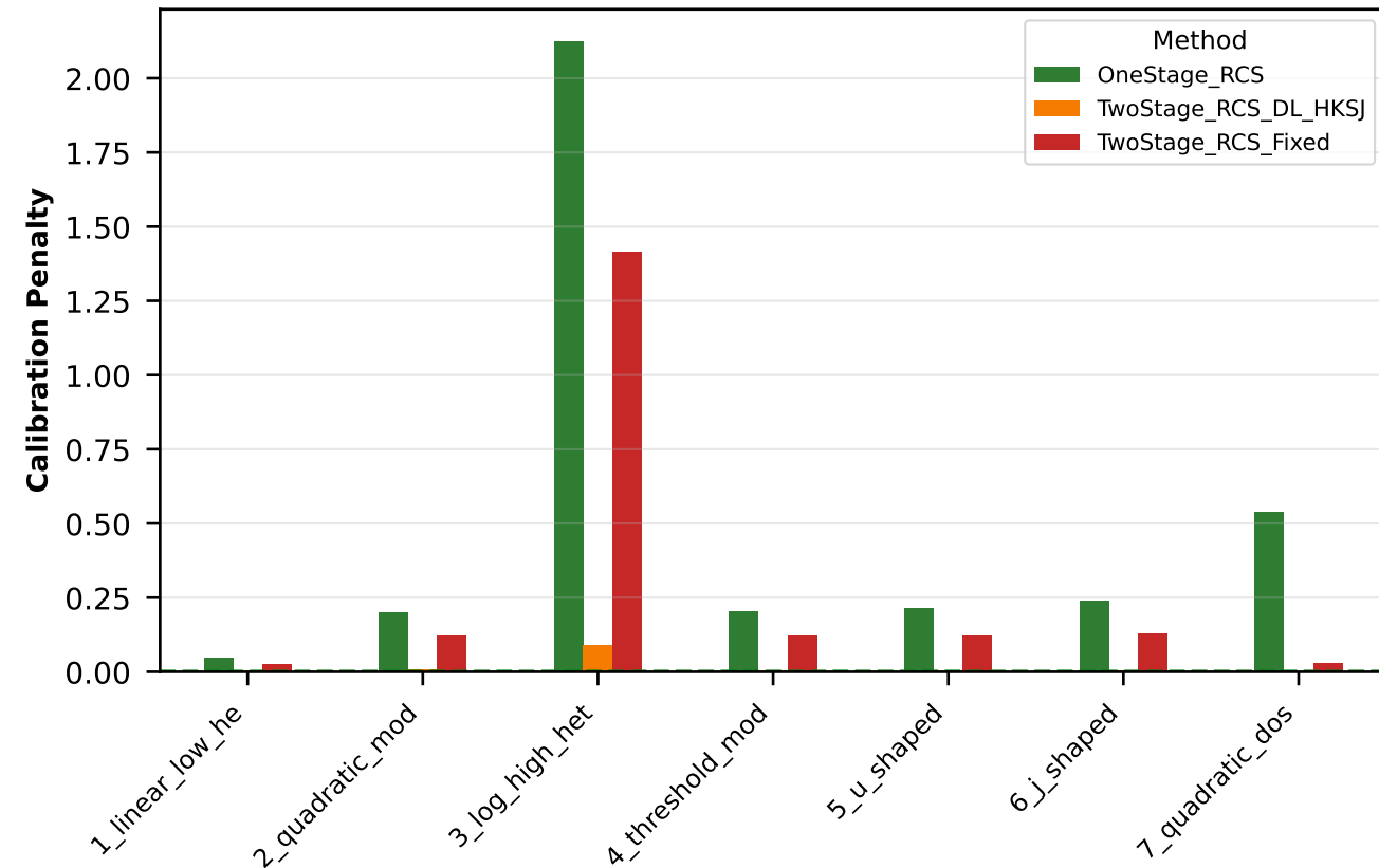
B. Calibration (Miscoverage Penalty) by Scenario
