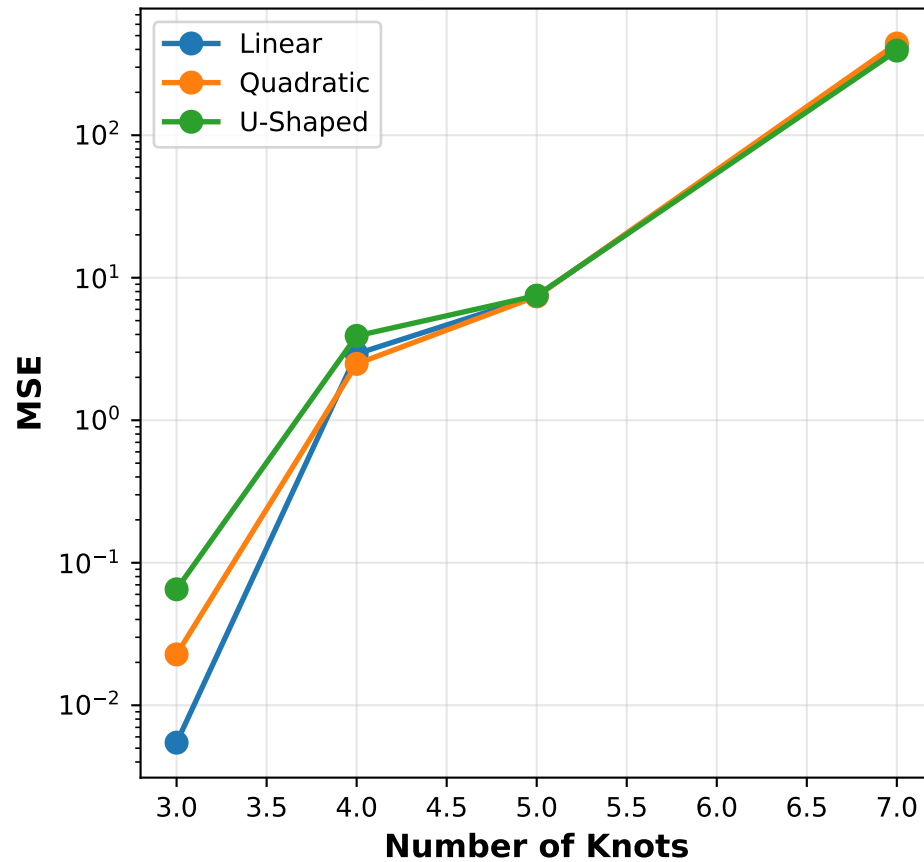
MSE by Number of Knots
