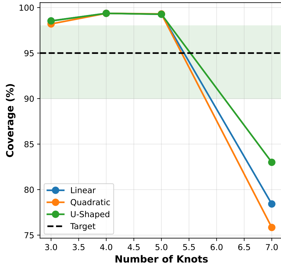
Coverage by Number of Knots
