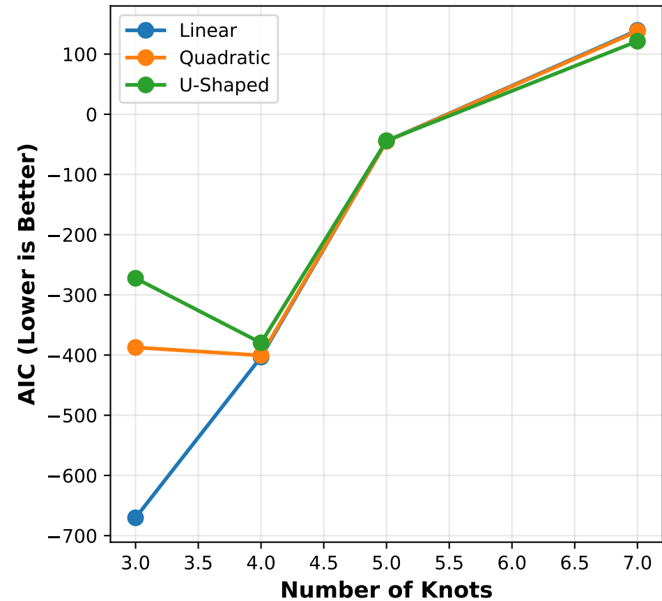
AIC by Number of Knots
