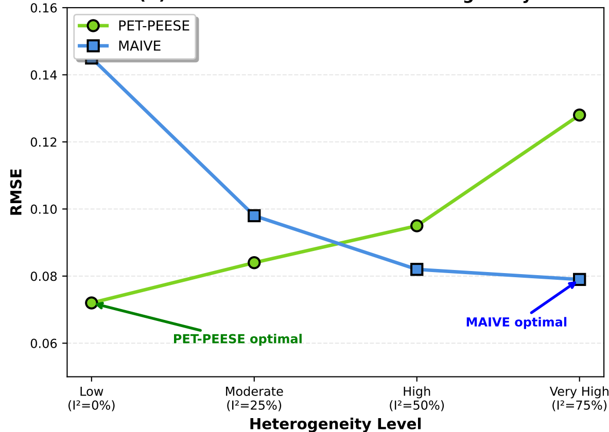
(A) Method Performance vs Heterogeneity
