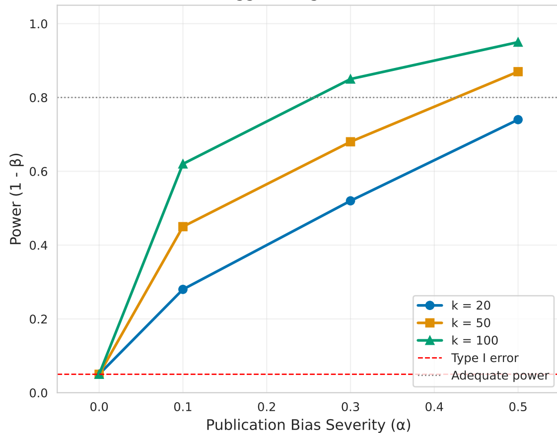
A. Egger's Regression Test
