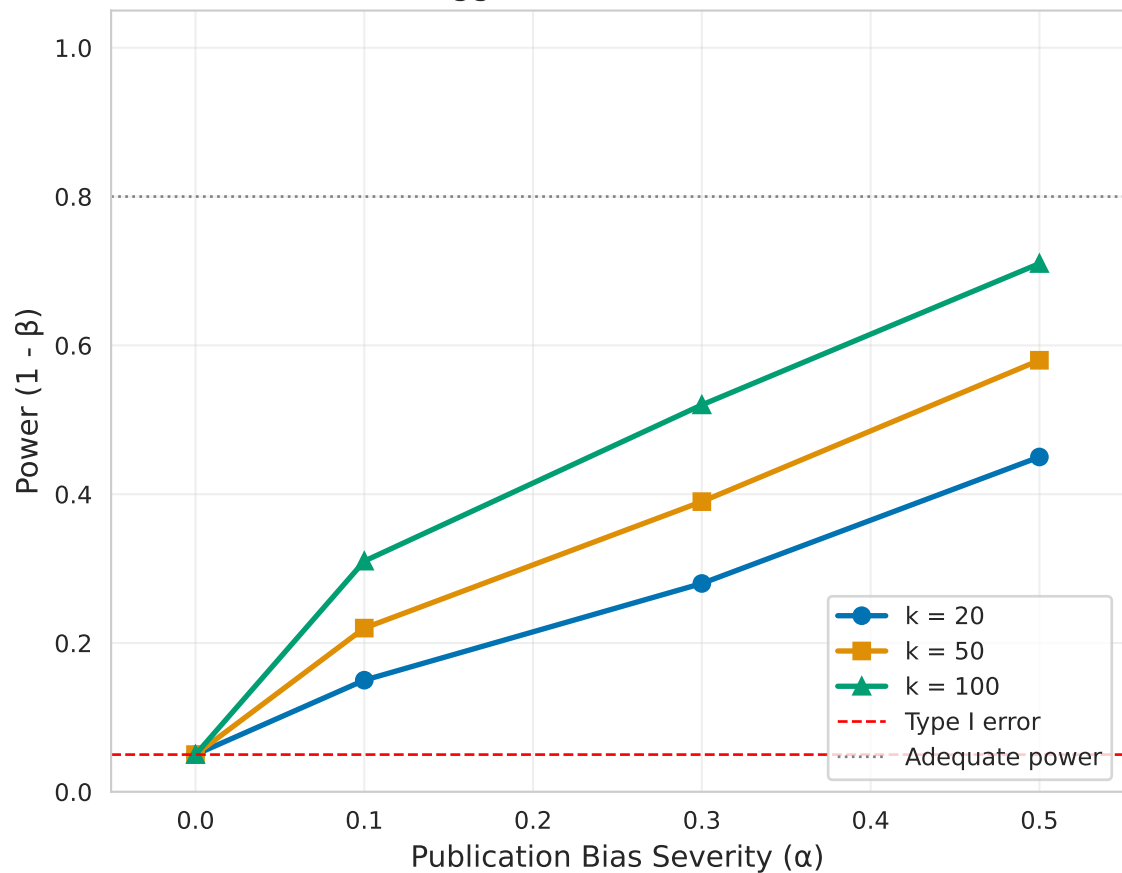
B. Begg's Rank Correlation Test
