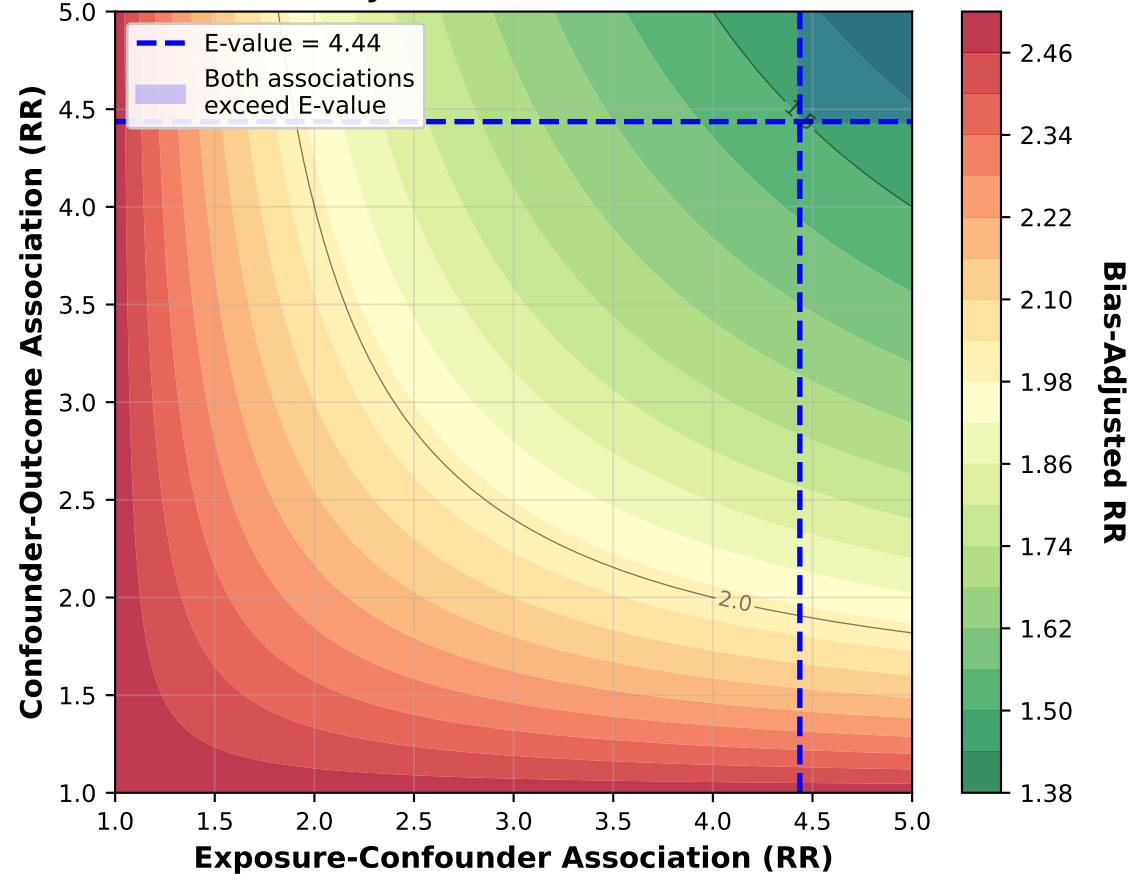
Panel A: Bias-Adjusted RR for Observed RR = 2.5
