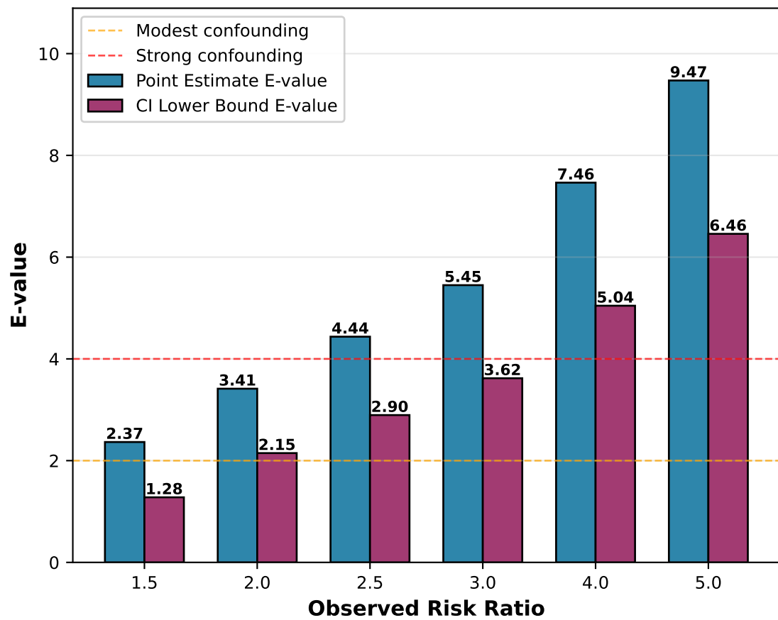
Panel B: E-values for Different Effect Sizes
