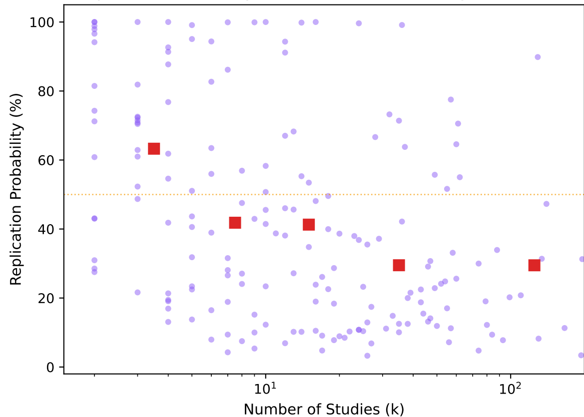
Replication Probability vs Number of Studies (Significant MAs)
