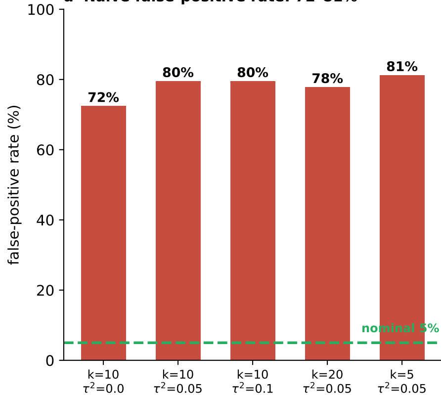
a Naive false-positive rate: 72-81%
