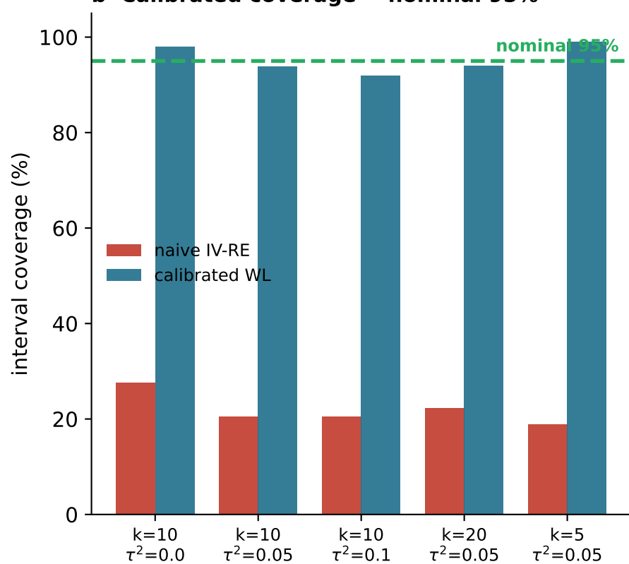
b Calibrated coverage \approx nominal 95%
