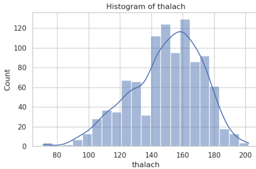
Figure 4: Histogram of the thalach attribute.
