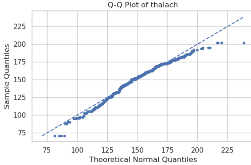
Figure 13: Q-Q plot of the thalach attribute.
