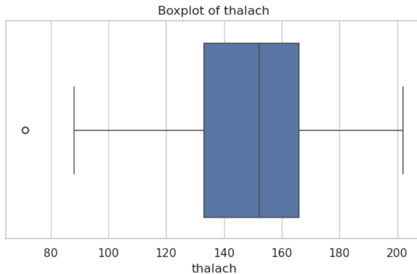
Figure 9: Boxplot of the thalach attribute.
