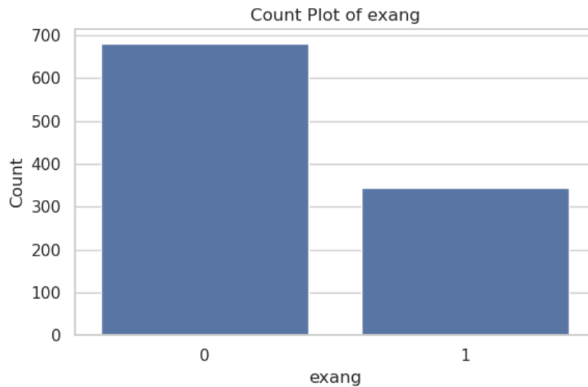
Figure 17: Count plot of the exang attribute.
