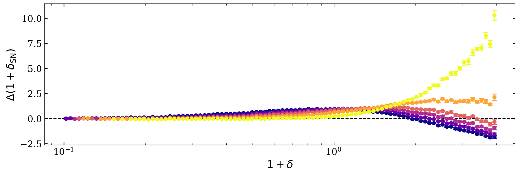
Difference relative to Uchuu-ZTF
