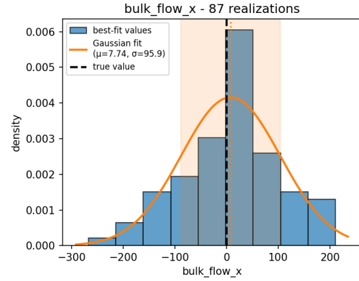
(b) Coverage for V_x
