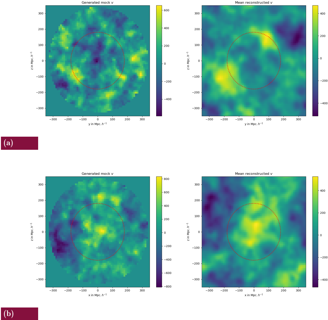
Fig. 6.23 Slices of the velocity field from Uchuu and BORG reconstruction after having gone a CIC mass assignment. The left column shows the Uchuu velocity field. The right column shows the mean posterior from BORG. Each row is a different slice in the box. The first row is a slice in the x axis. The second row is a slice in the y axis.
