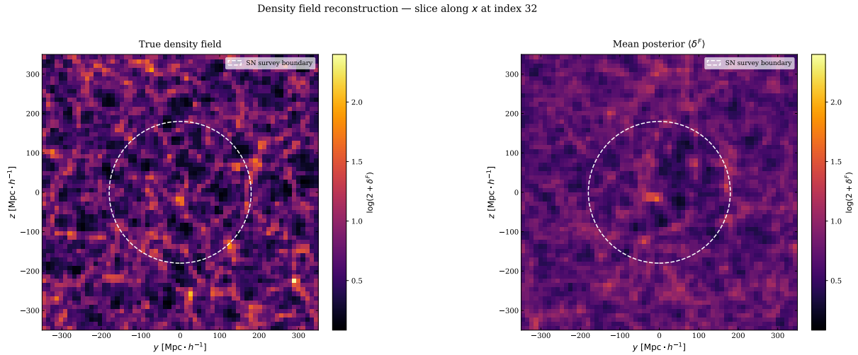
Fig. 6.12 Slice 32 on the x -axis of the generated density field and posterior mean using self-consistent simulations.
