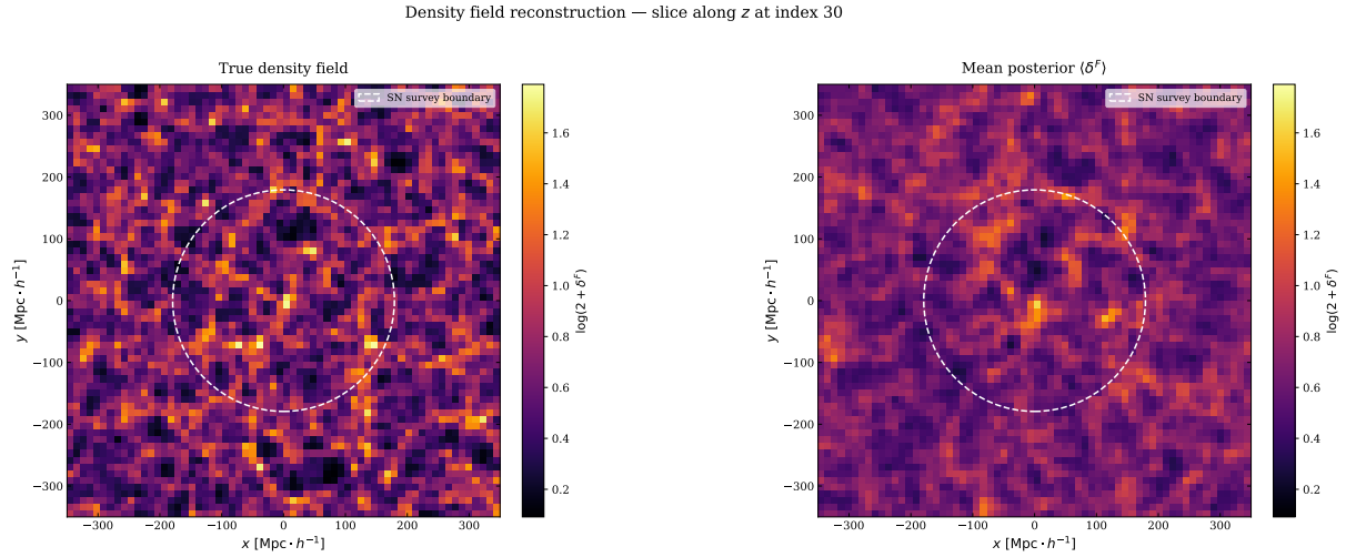
Fig. 6.14 Slice 30 on the z -axis of the generated density field and posterior mean using self-consistent simulations.
