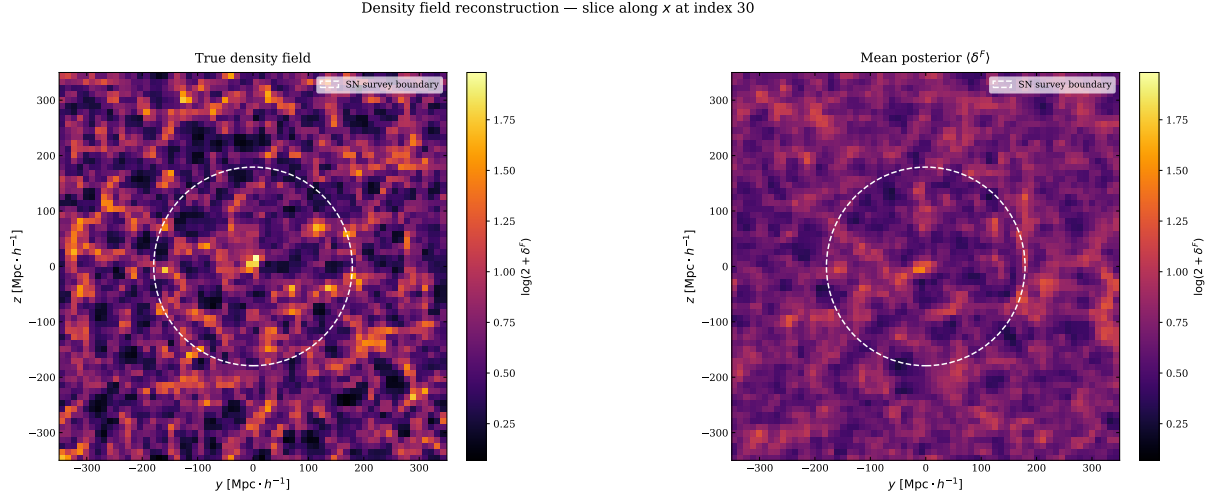
Fig. 6.11 Slice 30 on the x -axis of the generated density field and posterior mean using self-consistent simulations.
