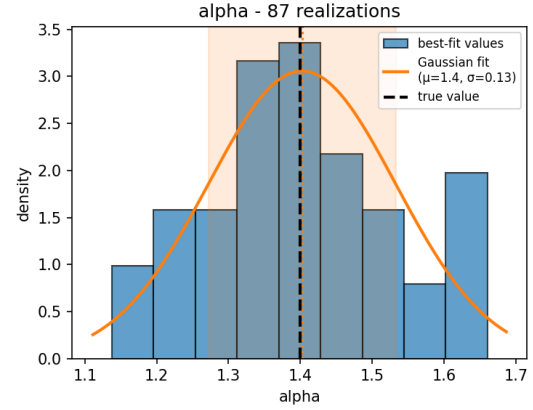
(b) Coverage for \alpha_8
