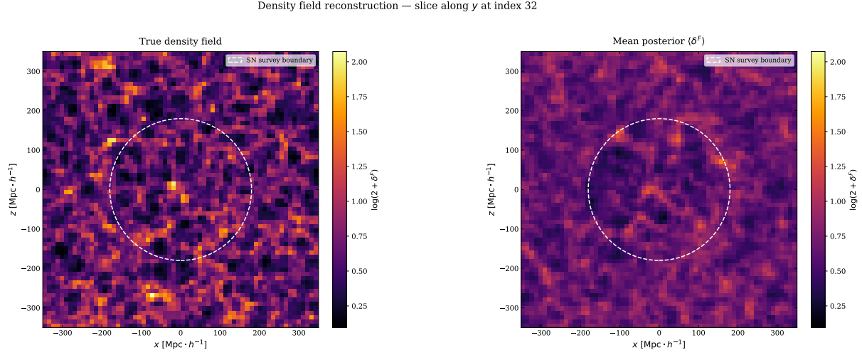
Fig. 6.13 Slice 32 on the y -axis of the generated density field and posterior mean using self-consistent simulations.
