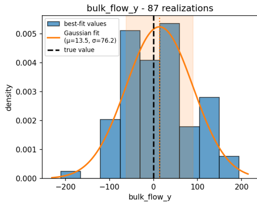
(a) Coverage for V_y
