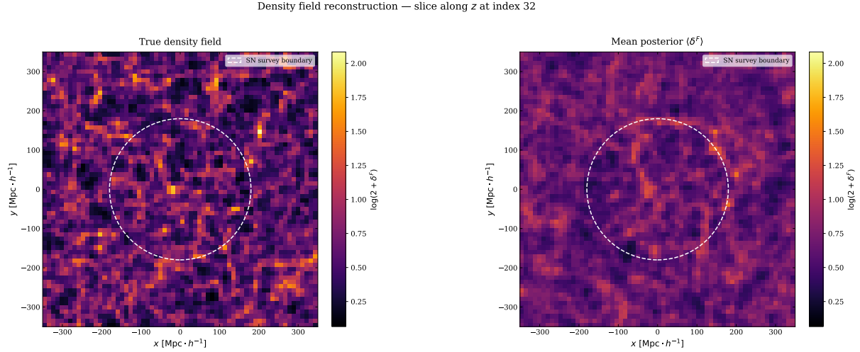
Fig. 6.15 Slice 32 on the z -axis of the generated density field and posterior mean using self-consistent simulations.
