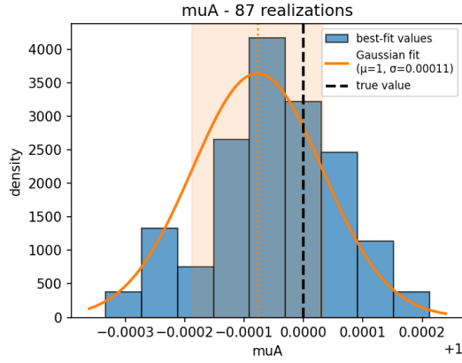
(a) Coverage for \mu_a
