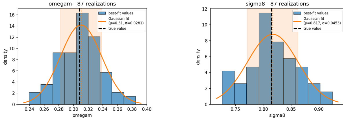
(a) Coverage for \Omega_m
