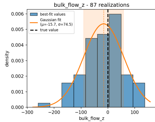
(b) Coverage for V_z
