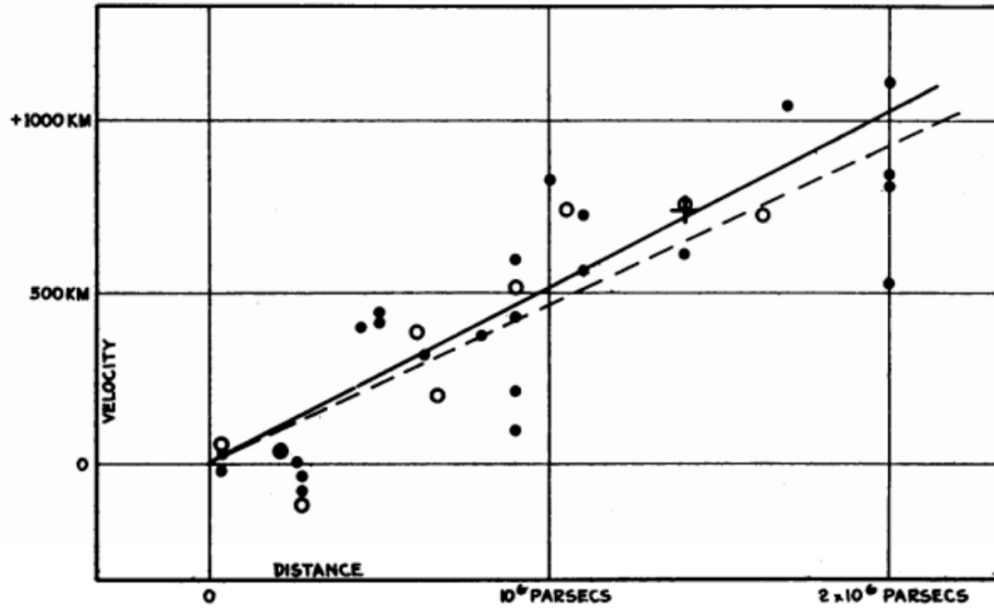
Fig. 1.4 Original Hubble diagram ([Hubble, 1929]) portraying the distance velocity diagram of nearby galaxies.
