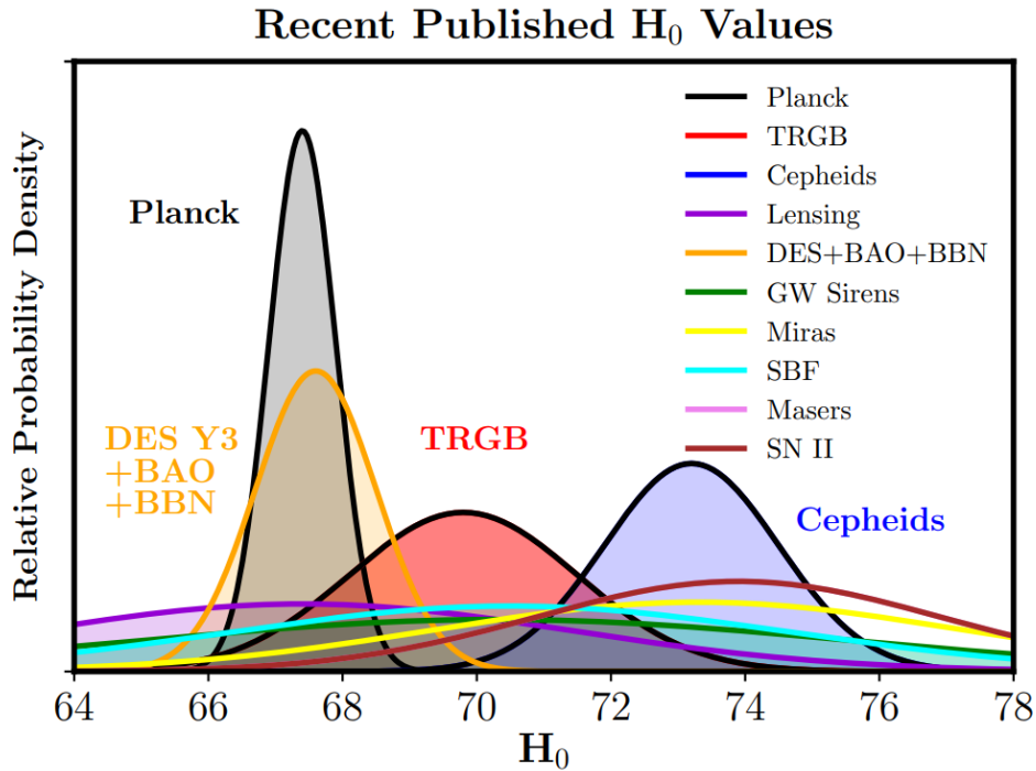
Fig. 1.13 Probability density functions of H_0 from different measurements probed at different redshifts, taken from [Freedman, 2021]. The CMB measurements prefer a lower H_0 value while Cepheids prefer higher values.
