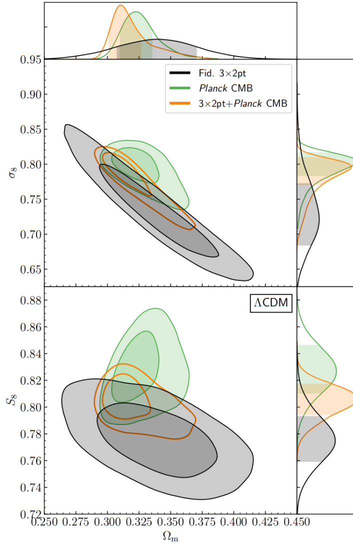
Fig. 1.11 A comparison of the marginalized parameter constraints in the \Lambda CDM model from the Dark Energy Survey ([DES Collaboration et al., 2022a]) with predictions from Planck CMB data (no lensing; green). There is also the fiducial cosmology 3x2pt (black) and the combined Y3 3x2pt and Planck (orange) results.
