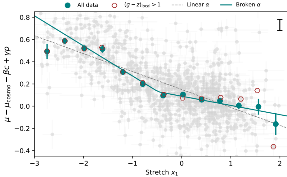
Fig. 2.8 Binned Hubble residuals as a function of the stretch. The data is fitted to highlight the two regimes of the broken alpha relation [Ginolin et al., 2025b].
