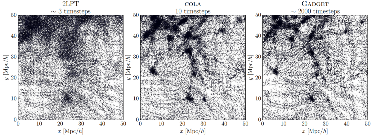
Fig. 6.3 Evolution of the same initial density field with three gravity solvers 2LPT, COLA and GADGET
