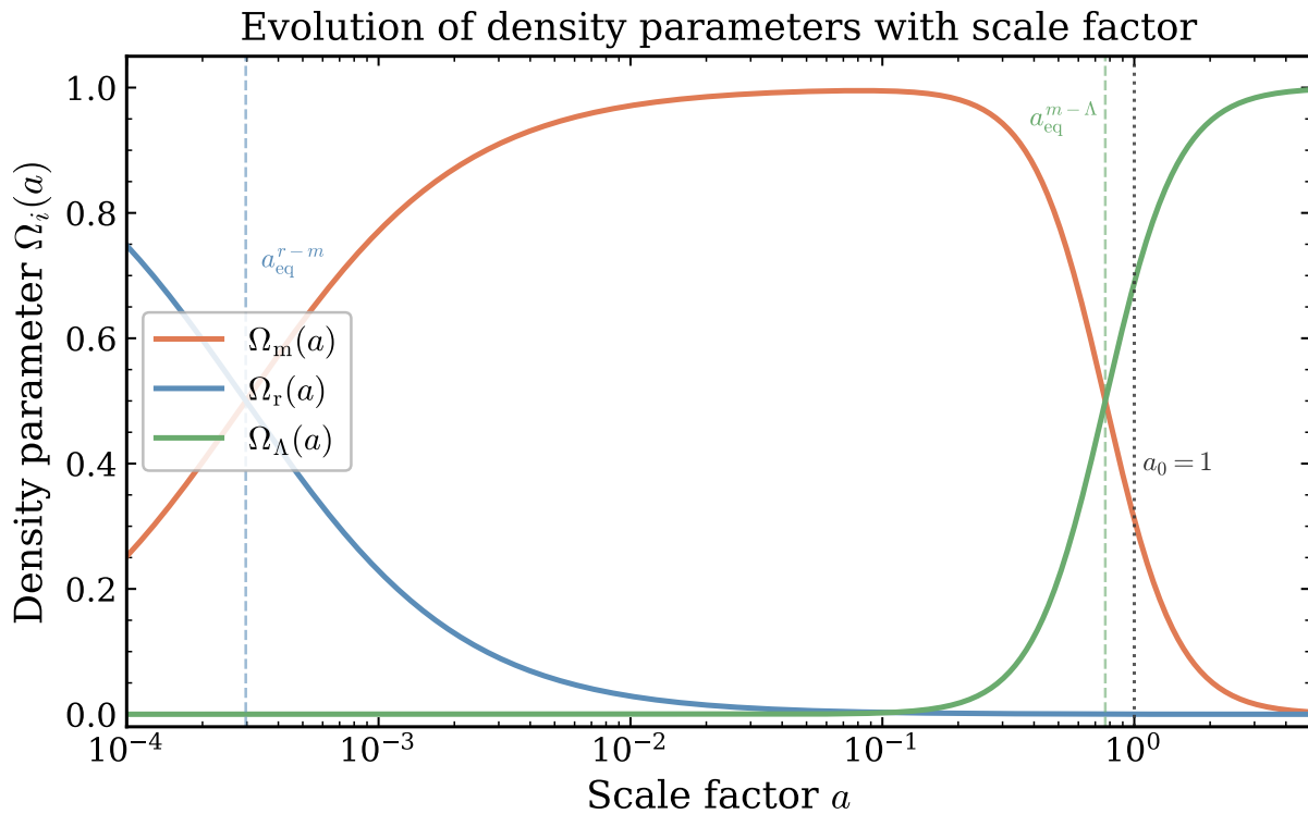
Fig. 1.5 Evolution of the main components of the \Lambda CDM model with respect to the scale factor. This highlights where each component dominates as well as when they become equal.
