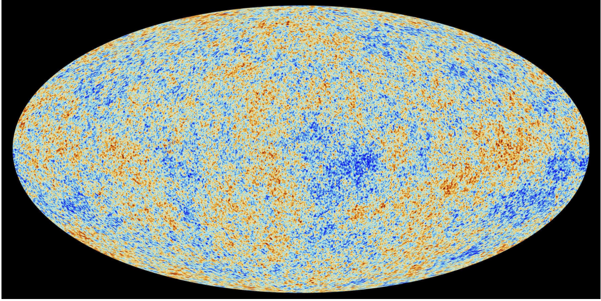
Fig. 1.3 CMB map provided by ESA and the Planck Collaboration.
