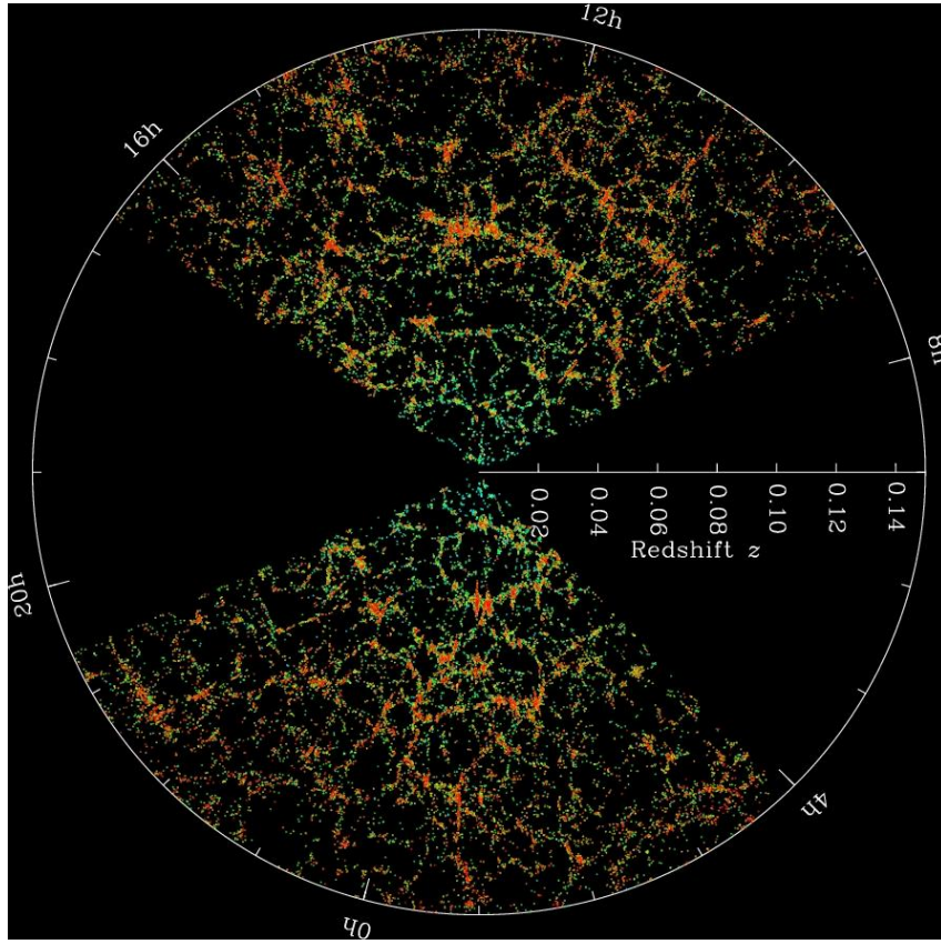
Fig. 1.1 Sky coverage of SDSS portraying the large scale structures of their measured galaxies.
