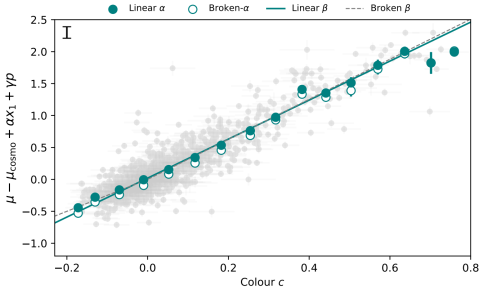
Fig. 2.9 Binned Hubble residuals as a function of color. The data is fitted to highlight the brighter-bluer effect ([Ginolin et al., 2025a]).
