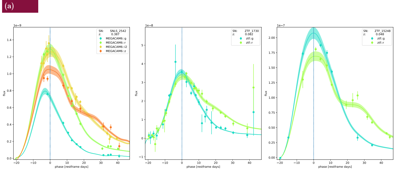
Fig. 4.2 Visual representation of the error snake on simulated lightcurves from DC1 (see section (reference)). In 4.2a we see how the model represents the data without an error snake model. In 4.2b we see a highlighted section for each lightcurves which are the variations modeled by the error snake.
