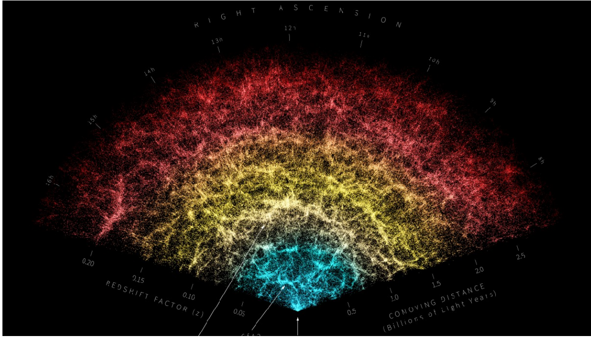
Fig. 1.2 Sky coverage of DESI portraying the large scale structures of their measured galaxies.
