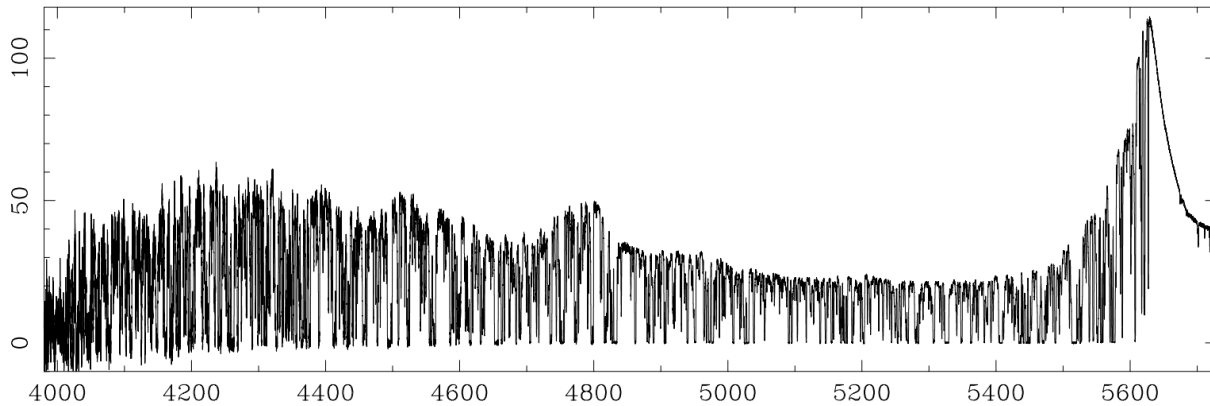
Fig. 1.12 High resolution spectrum of the Lyman- \alpha forest part of a quasar measured at z = 3.63 taken with the HIRES spectrograph on the 10 m Keck telescope in Hawai.
