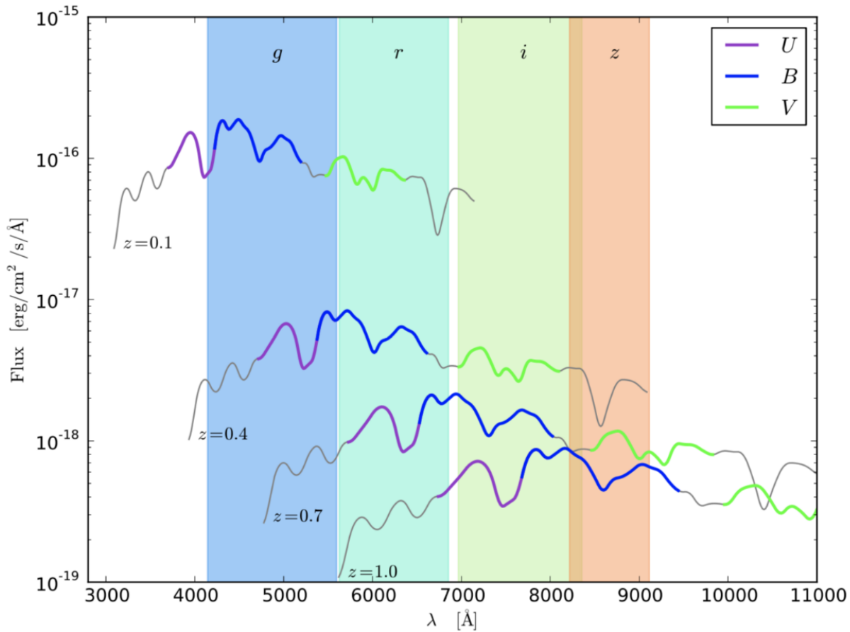
Fig. 2.7 Examples of four spectra at different redshifts 0.1, 0.4, 0.7 and 1.0. The highlighted parts of the spectra represent restframe band would measure. The highlighted areas on the graph are the regions where the observer bands measure.
