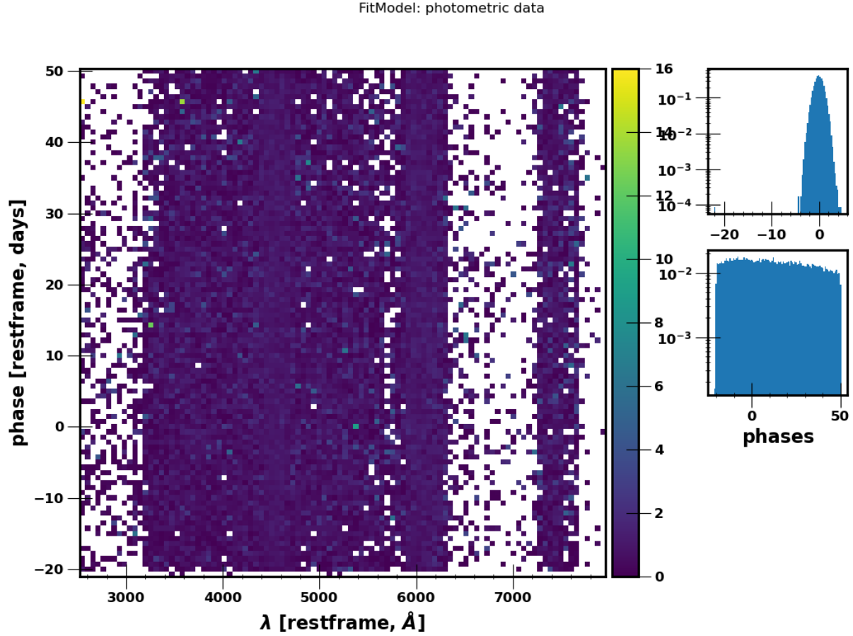
Fig. 5.1 Photometric residuals for 1 realization of pre-DC1
