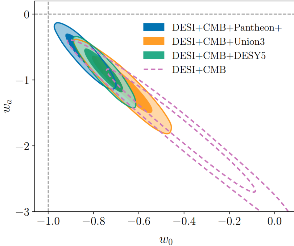
Fig. 1.15 w_0 and w_a contours from the latest [DESI Collaboration et al., 2025] measurements enclosing the the 68% and 95% posterior probability when combined with Pantheon+, UNION3 and DES year 5 data and CMB.
