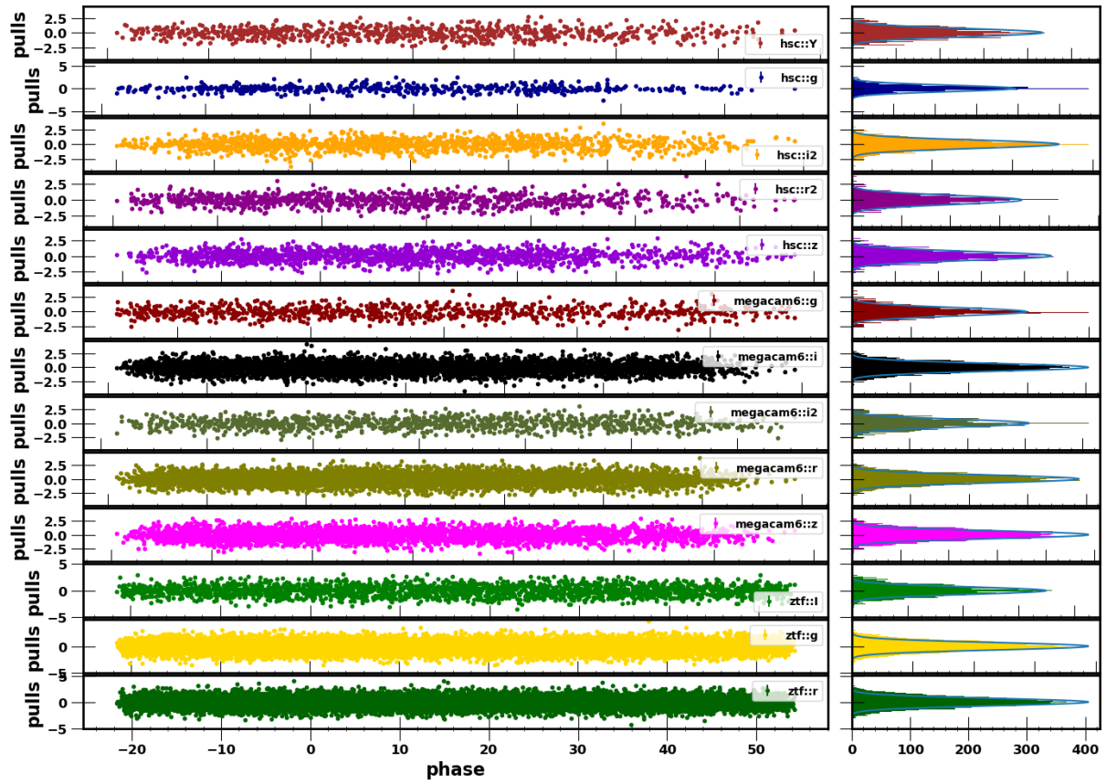
Fig. 5.3 Photometric residuals per band for 1 realization of pre-DC1
