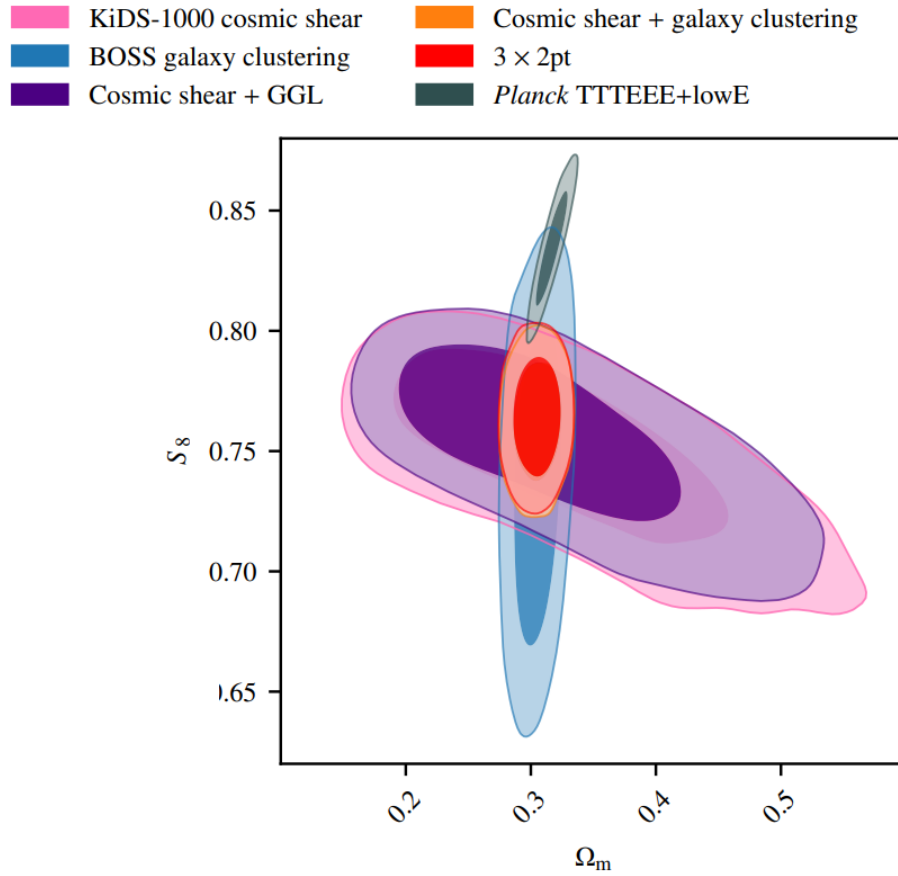
Fig. 1.14 S_8 and \Omega_m contours for different galaxy surveys and CMB taken from [Heymans et al., 2021b] enclosing the 68% and 95% posterior probability. It is highlighted that CMB measurements prefer higher S_8 values to galaxy surveys.
