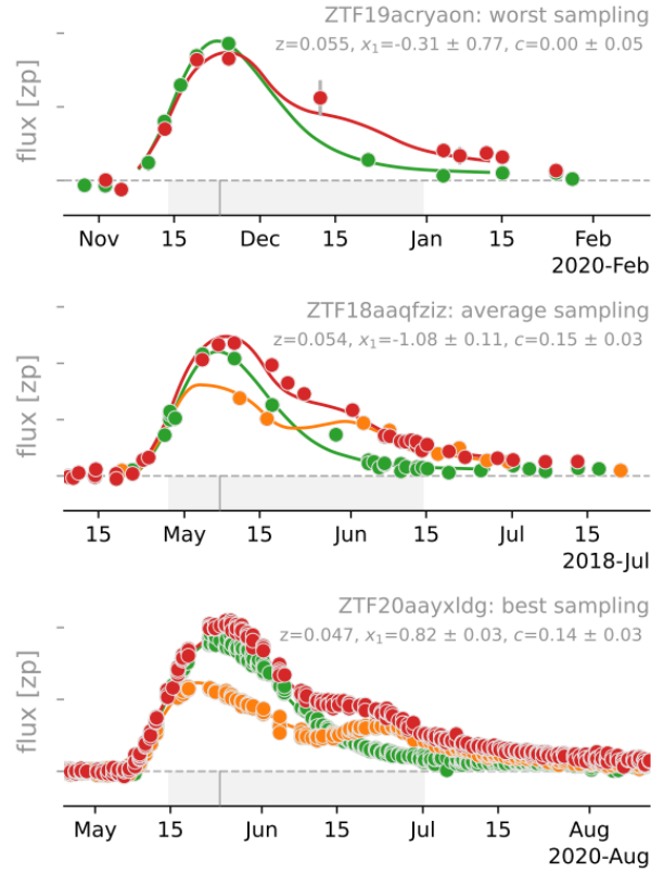
Fig. 3.7 Three supernova Ia lightcurves examples highlighting the worst (top), average (middle) and best (bottom) sampling in DR2. The colors indicate the band they were measured in and the solid lines are the best SALT2 fits. Taken from [Rigault et al., 2020]
