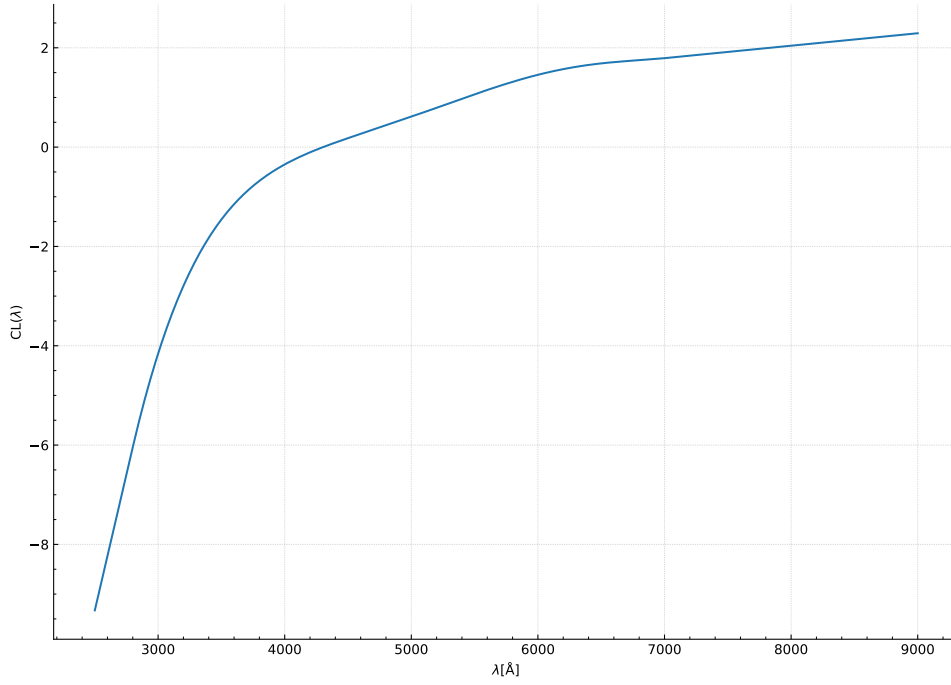
Fig. 2.13 The SALT2.4 color law CL surface with respect to the restframe wavelength
