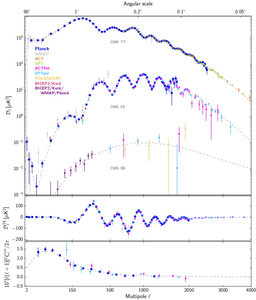
Fig. 1.8 Compilation of CMB angular power spectrum measurements from [Collaboration et al., 2020]. The upper panel shows the power spectra of the temperature and E -mode and B -mode polarization signals, the next panel the cross-correlation spectrum between T and E , while the lower panel shows the lensing deflection power spectrum
