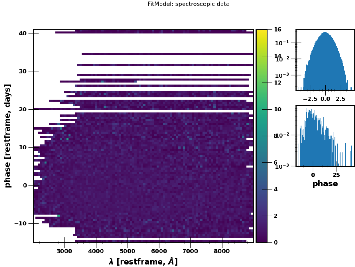
Fig. 5.2 Spectroscopic residuals for 1 realization of pre-DC1
