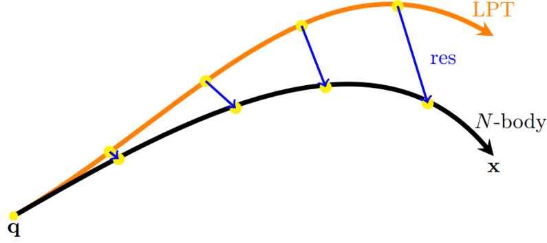
Fig. 6.2 Schematic representing how COLA works found in [Bartlett et al., 2025]. The orange line represents the motion of the particle from the LPT frame of reference and the blue lines are the residuals COLA calculates from the true position to correct for it.
