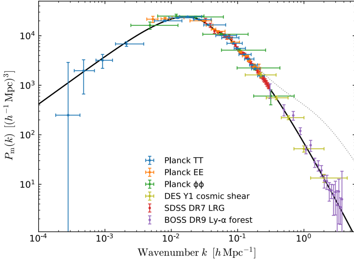
Fig. 1.9 Linear-theory matter power spectrum (at z = 0 ) inferred from different cosmological probes taken from [Collaboration et al., 2020].
