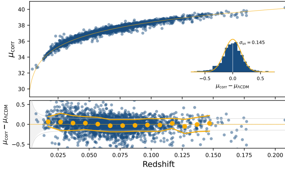
Fig. 3.6 Hubble diagram created with standardized ZTF DR2 type Ia supernovae compared to fiducial \Lambda CDM cosmology anchored on Planck results. Taken from [Rigault et al., 2020].
