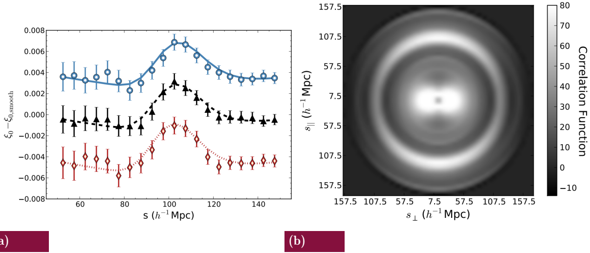
Fig. 1.10 BAO signals in the measured correlation functions from SDD ([Alam et al., 2017]). On the left is the smoothed prediction of the best-fitted model. On the right the redshift bins are decomposed into the component of the separations transverse to and along the line of sight at 0.4 < z < 0.6 .
