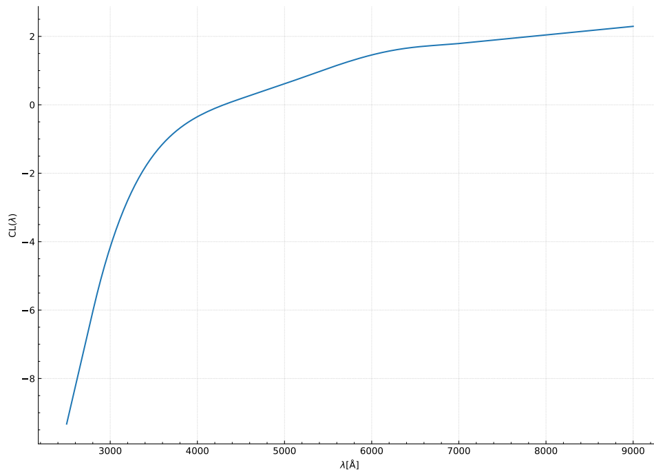
Fig. 2.13 The SALT2.4 color law CL surface with respect to the restframe wavelength
