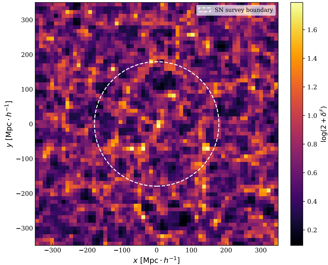
True density field
