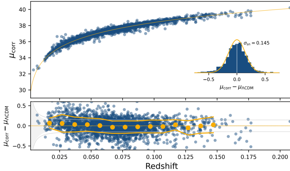
Fig. 3.7 Hubble diagram created with standardized ZTF DR2 type Ia supernovae compared to fiducial \Lambda CDM cosmology anchored on Planck results. Taken from [Rigault et al., 2020].
