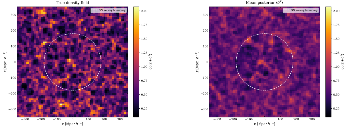
Fig. 6.10 Slice 32 on the y-axis of the generated density field and posterior mean using self-consistent simulations.
