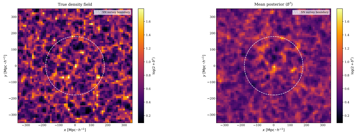
Fig. 6.11 Slice 30 on the z-axis of the generated density field and posterior mean using self-consistent simulations.
