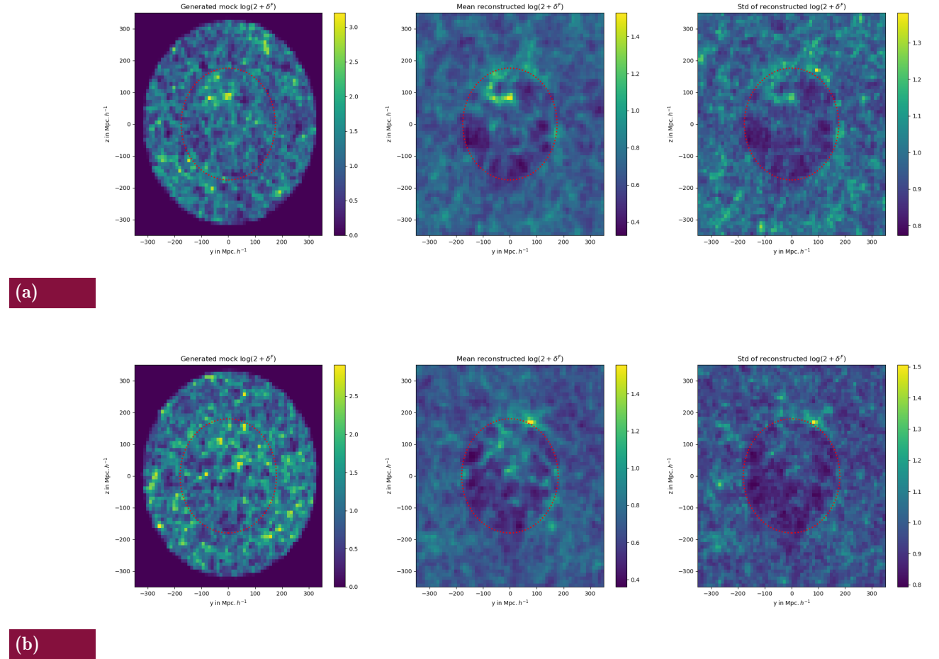
Fig. 6.19 Slices of the density field from Uchuu and BORG reconstruction after having gone a CIC mass assignment. The left column shows the Uchuu density field. The center column shows the mean posterior from BORG. The right column shows the standard deviation. Each row is a different slice in the box.
