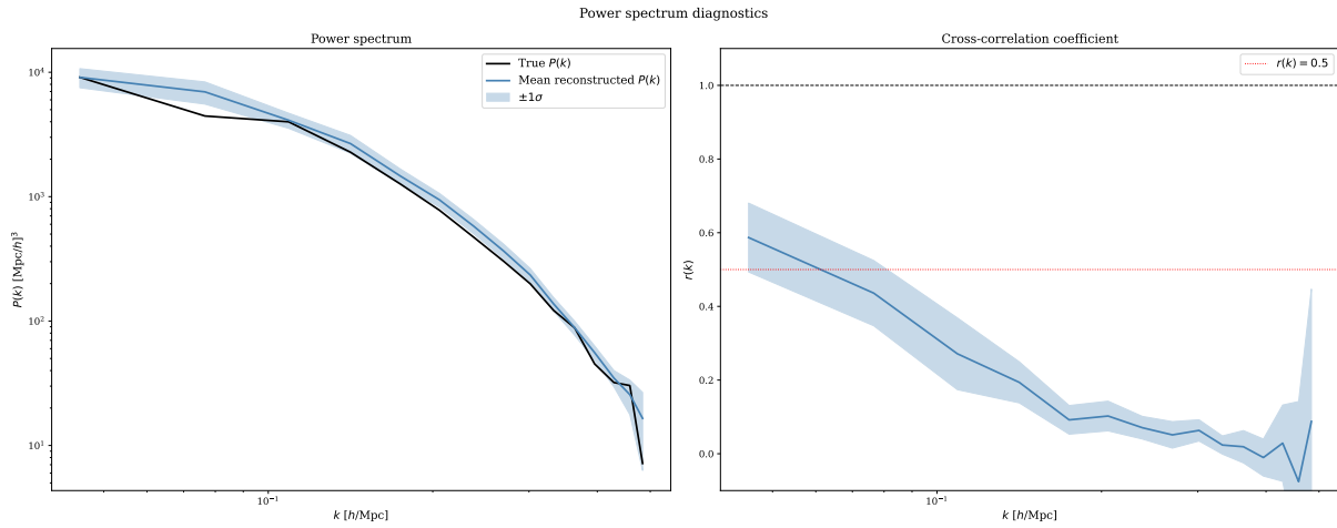
Fig. 6.13 Left: Matter power spectrum of the generated density field as well as the mean power spectrum and its standard deviation from the inference. Right: Cross correlation between the generated density field and the posterior mean field. The red dotted line represents a value of 0.5 where the correlations are at 50%.
