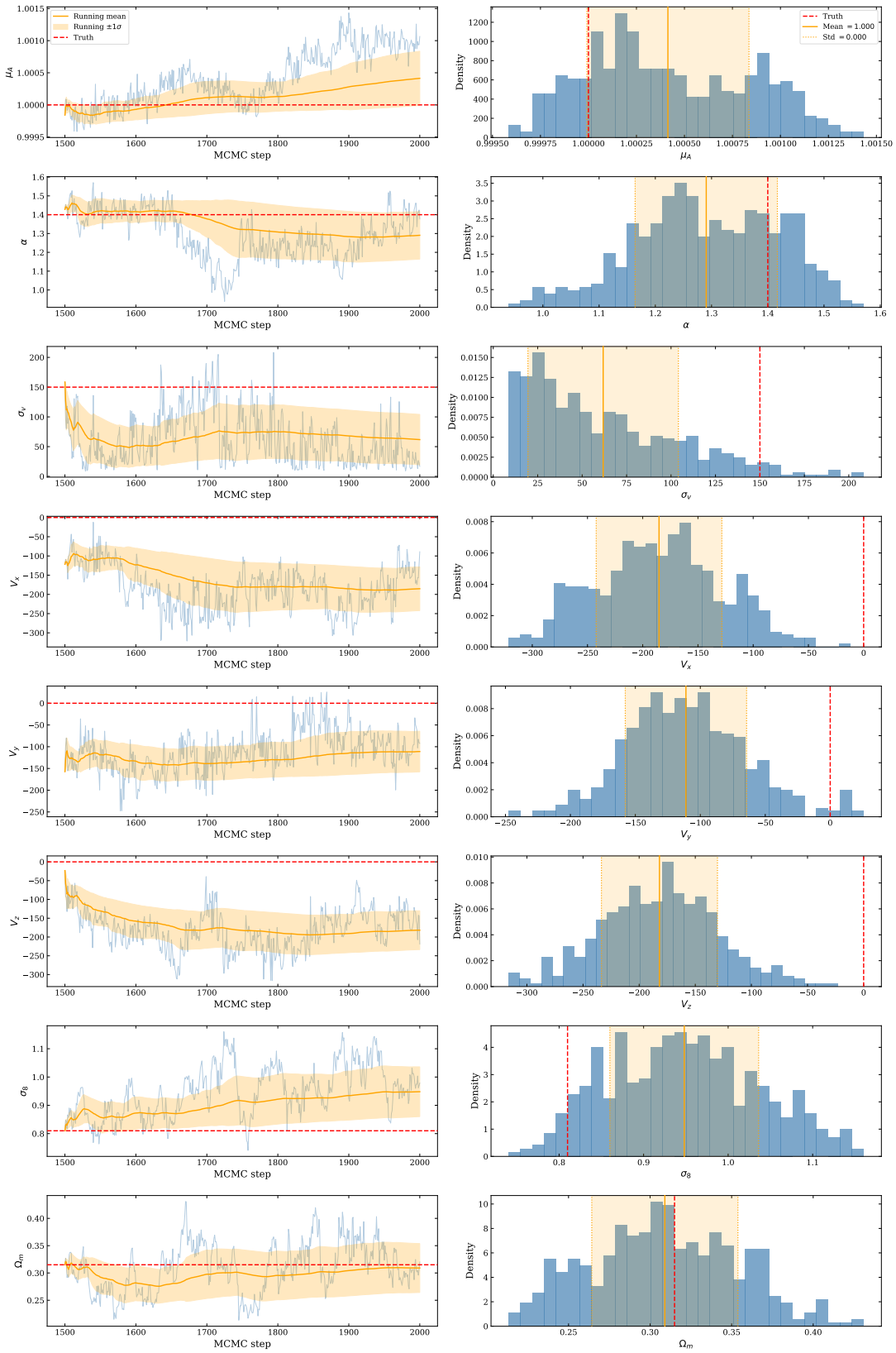
Fig. 6.14 Model and cosmological parameter sampling for the self-consistent simulation run.
