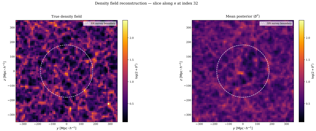
Fig. 6.9 Slice 32 on the x -axis of the generated density field and posterior mean using self-consistent simulations.
