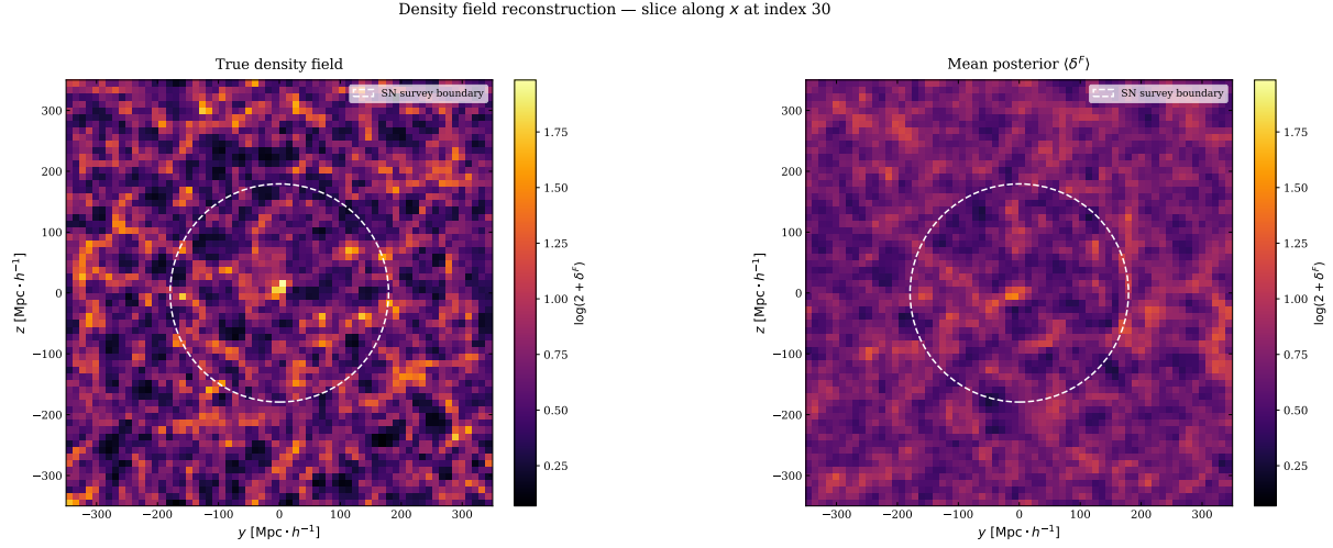
Fig. 6.8 Slice 30 on the x -axis of the generated density field and posterior mean using self-consistent simulations.
