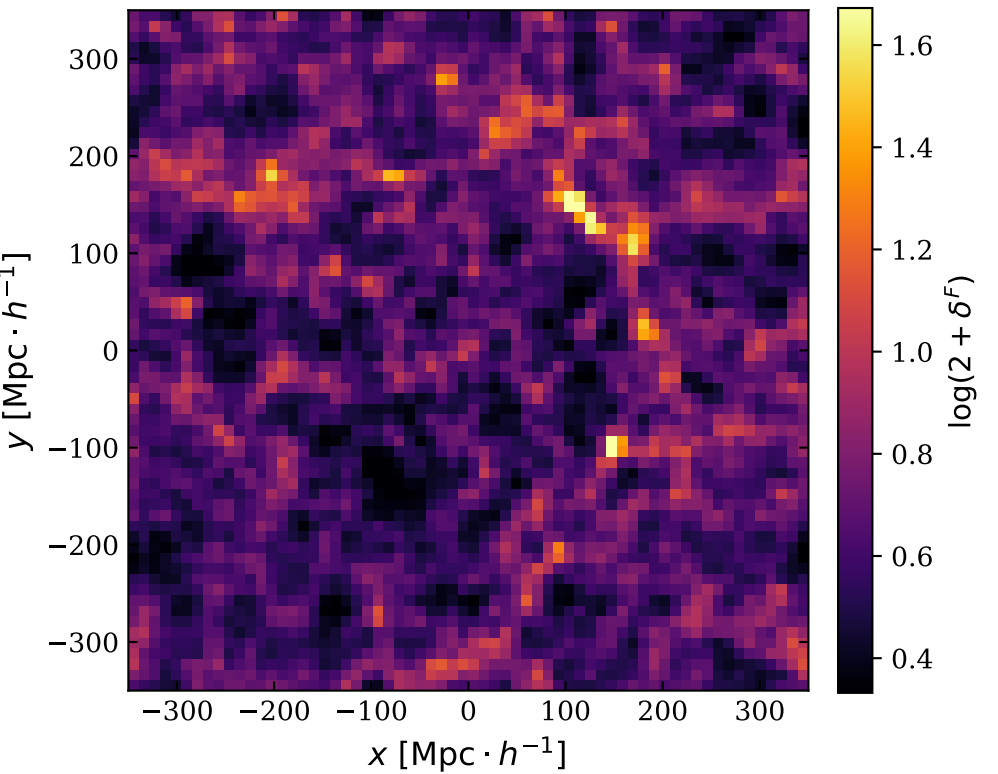
After sampling cosmological parameters
