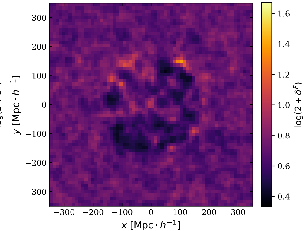
After samling model parameters
