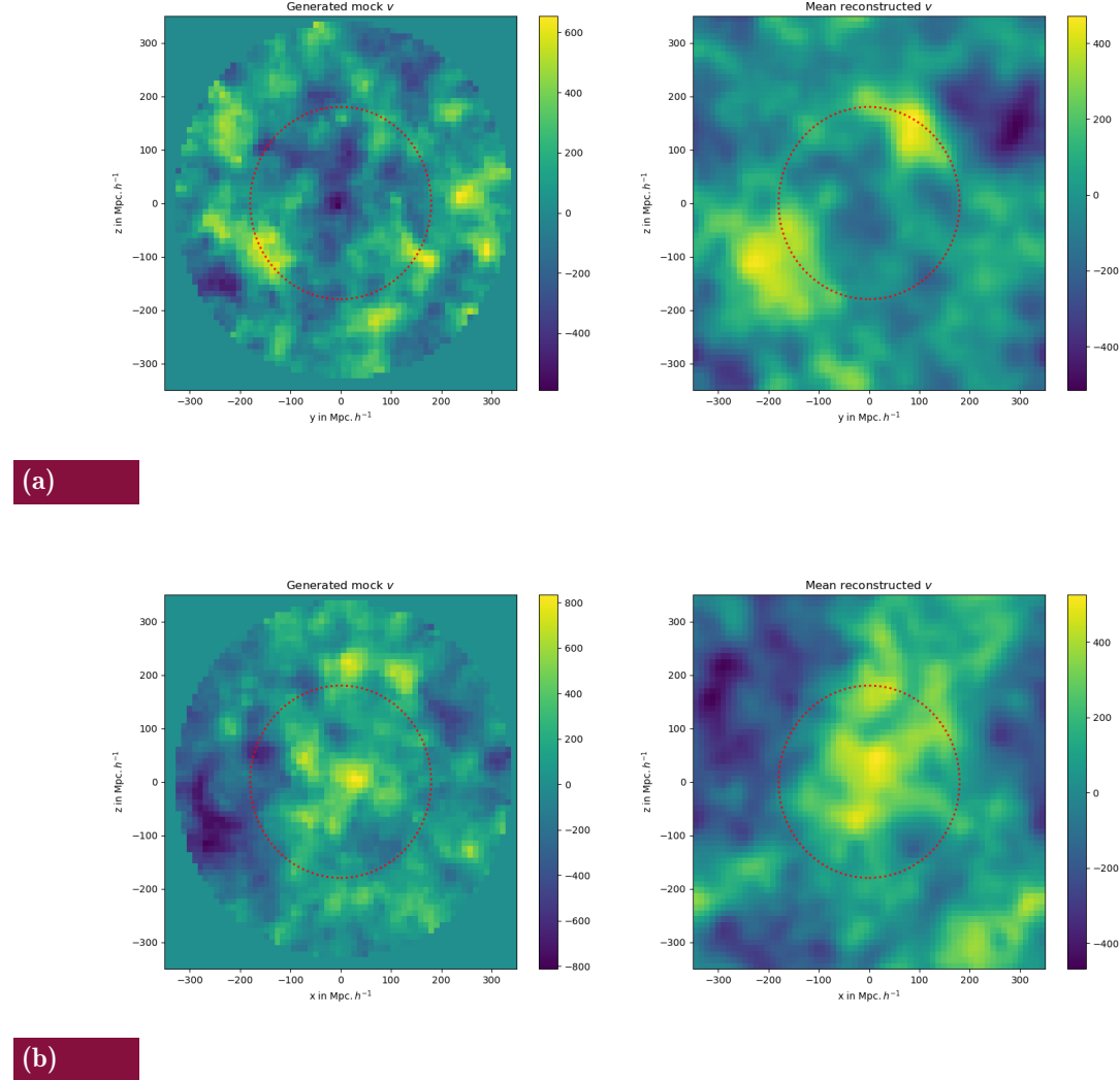
Fig. 6.8 Slices of the velocity field from Uchu and BORG reconstruction after having gone a CIC mass assignment. The left column shows the Uchu velocity field. The right column shows the mean posterior from BORG. Each row is a different slice in the box. The first row is a slice in the x axis. The second row is a slice in the y axis.
