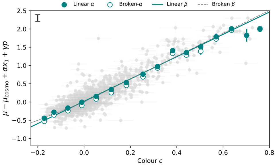
Fig. 2.8 Binned Hubble residuals as a function of color. The data is fitted to highlight the brighter-bluer effect ([Ginolin et al., 2025a]).
