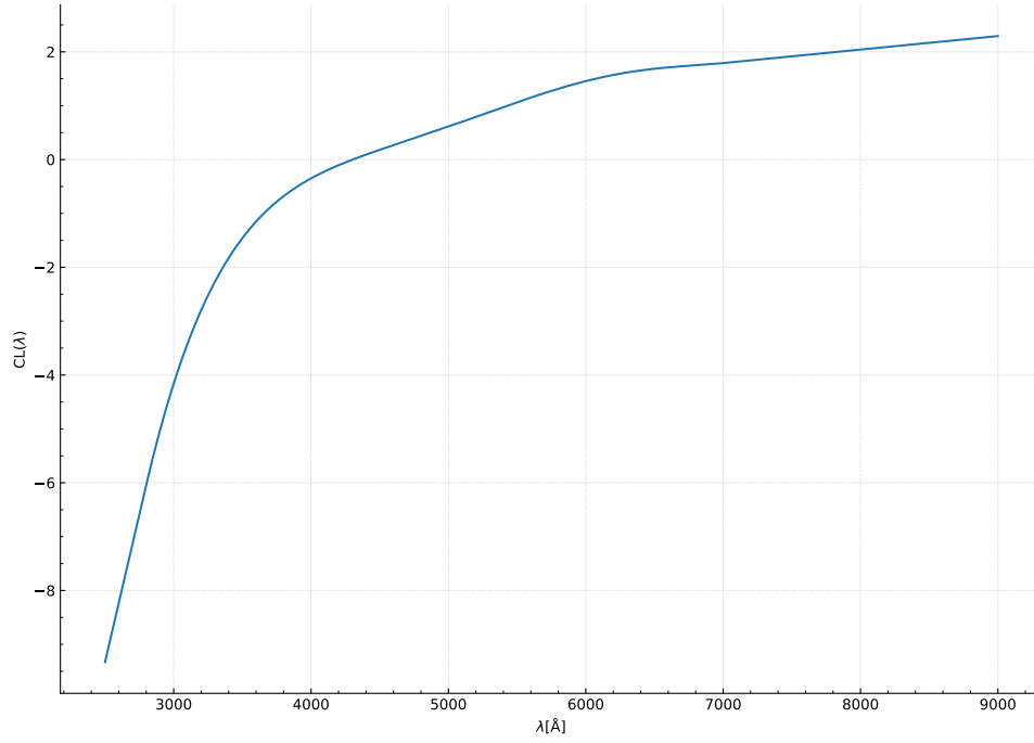
Fig. 4.4 The SALT2.4 color law CL surface with respect to the restframe wavelength
