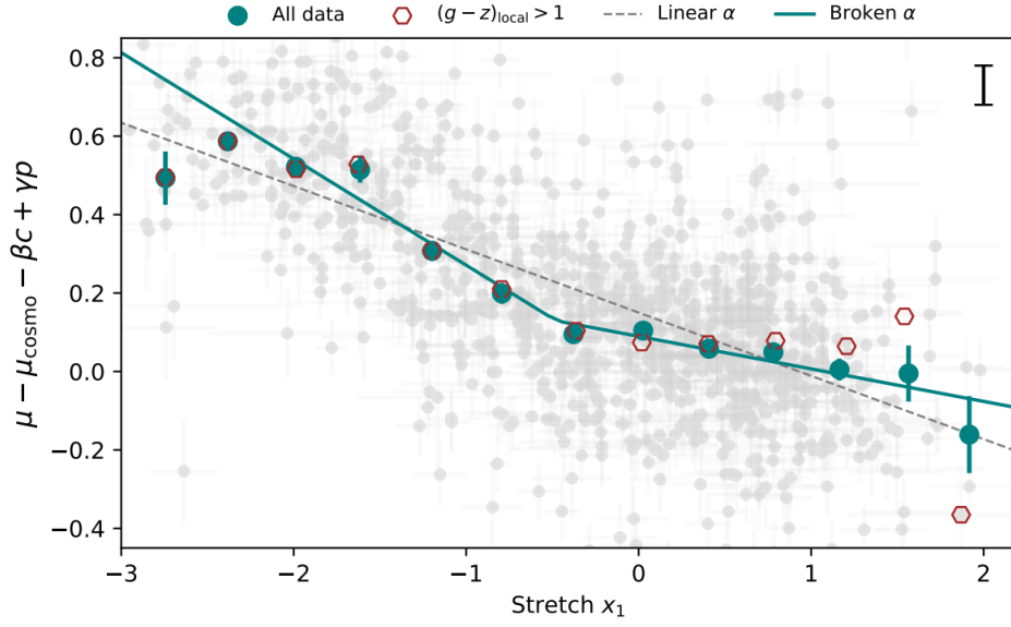
Fig. 2.7 Binned Hubble residuals as a function of the stretch. The data is fitted to highlight the two regimes of the broken alpha relation [Ginolin et al., 2025b].
