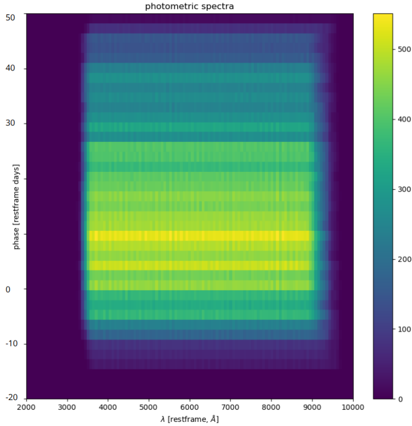
Fig. 4.8 Coverage of the SNfactory data in the \lambda - p space.
