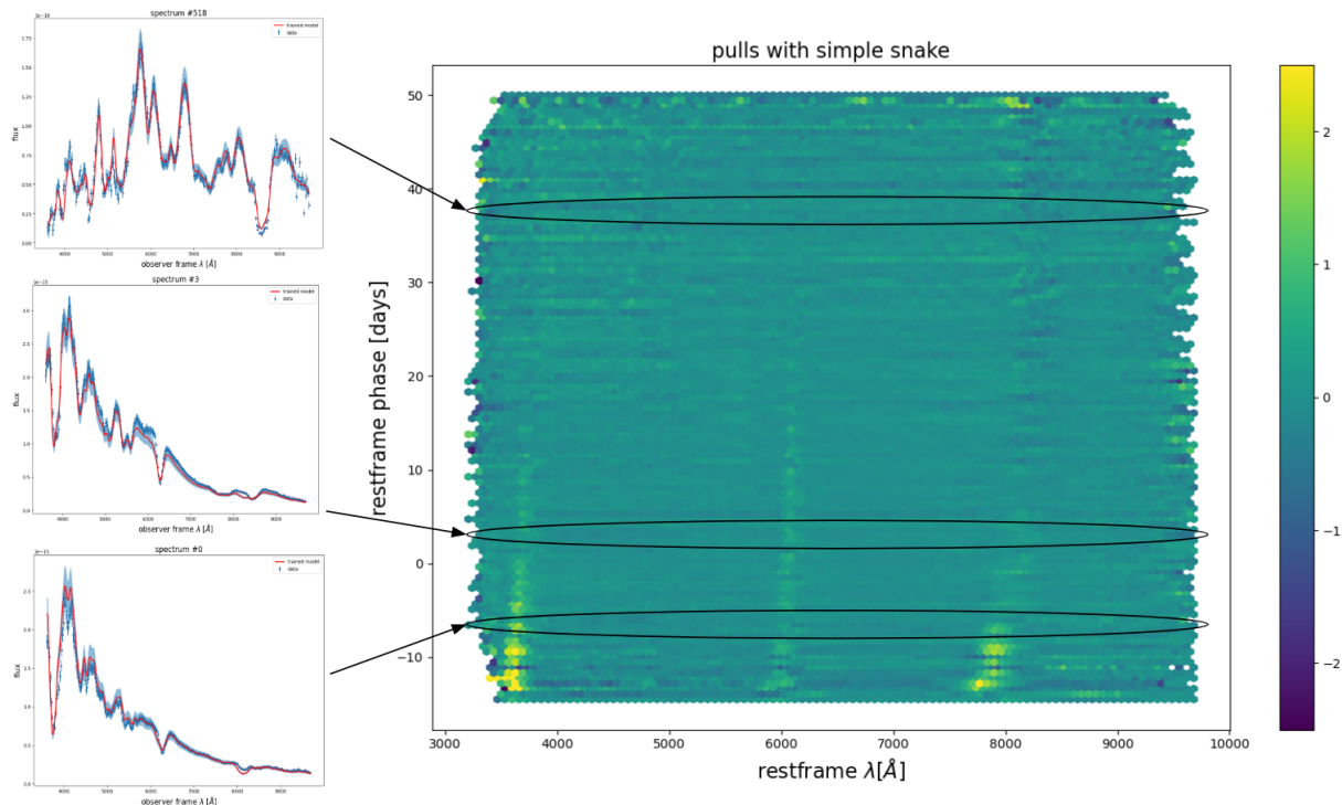
Fig. 4.10 Weighted residuals at the end of the training done with NaCl on the SNfactory data. The color bar represents by how many \sigma our model differs from the data. We also use as examples 3 spectra at 3 different phases and show where they would be present on the plot.
