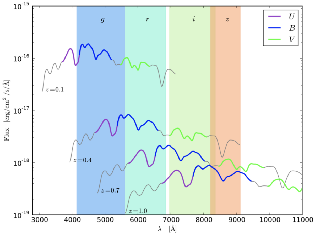
Fig. 4.1 Examples of four spectra at different redshifts 0.1, 0.4, 0.7 and 1.0. The highlighted parts of the spectra represent restframe band would measure. The highlighted areas on the graph are the regions where the observer bands measure.
