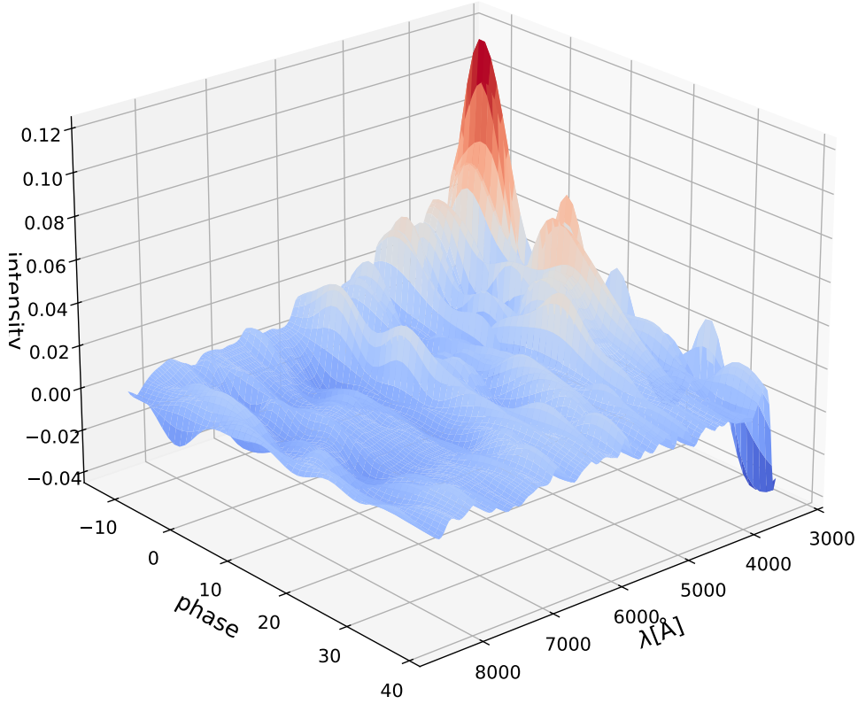
Fig. 4.3 The SALT2.4 M_1 surface with respect to the restframe wavelength and phase
