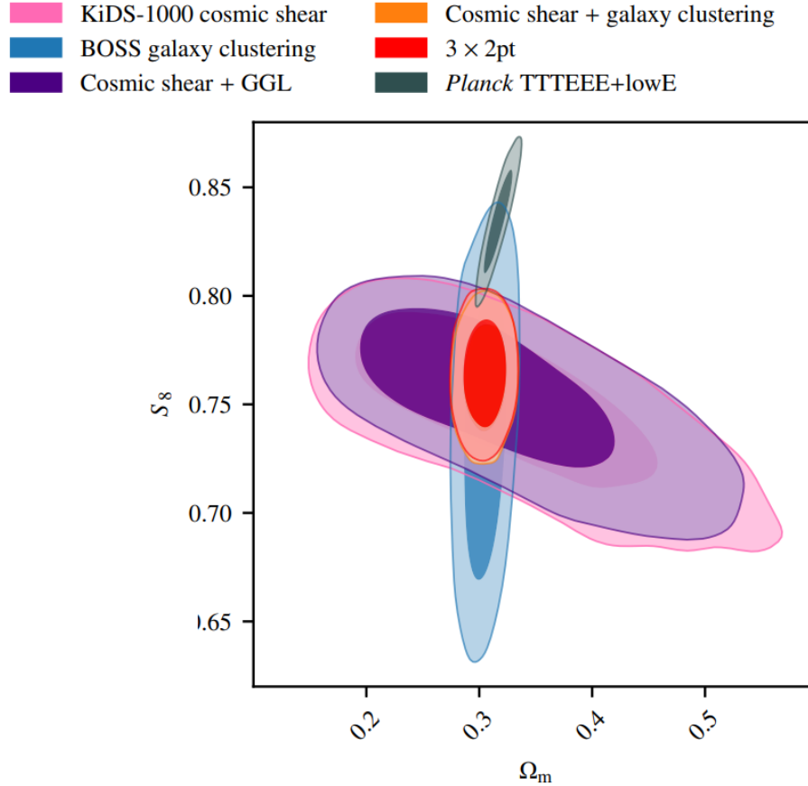
Fig. 1.12 S_8 and \Omega_m contours for different galaxy surveys and CMB taken from [Heymans et al., 2021b] enclosing the 68% and 95% posterior probability. It is highlighted that CMB measurements prefer higher S_8 values to galaxy surveys.
