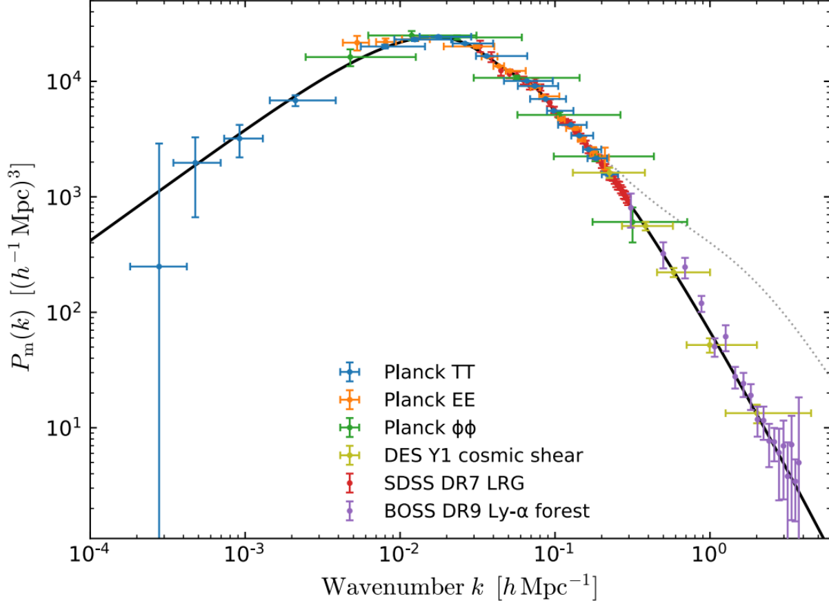
Fig. 1.7 Linear-theory matter power spectrum (at z = 0 ) inferred from different cosmological probes taken from [Collaboration et al., 2020].
