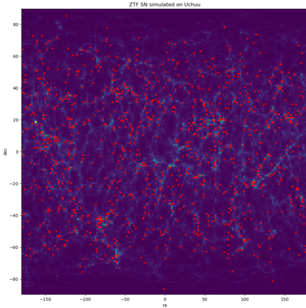
Fig. 6.2 2D full-sky projection of the Uchuu density field at redshift of z \approx 0.04 with the ZTF supernovae simulated on top of it represented by red dots.
