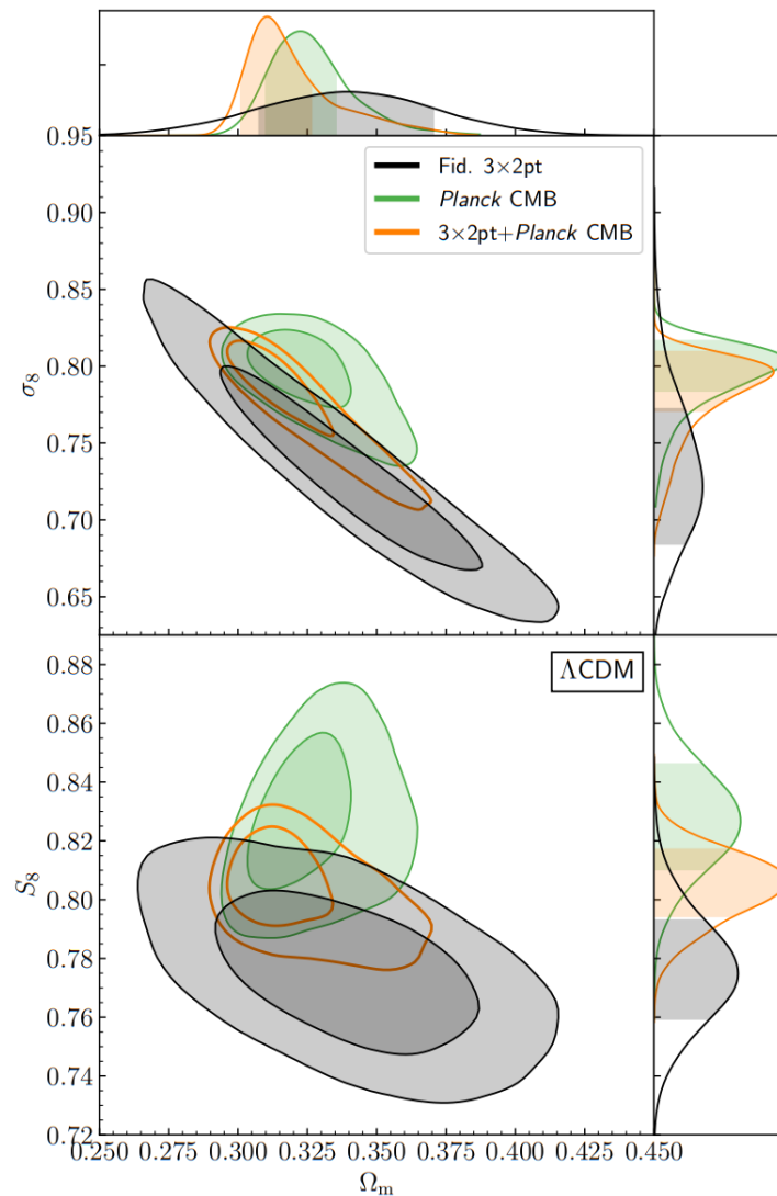
Fig. 1.9 A comparison of the marginalized parameter constraints in the \Lambda CDM model from the Dark Energy Survey ([DES Collaboration et al., 2022a]) with predictions from Planck CMB data (no lensing; green). There is also the fiducial cosmology 3x2pt (black) and the combined Y3 3x2pt and Planck (orange) results.
