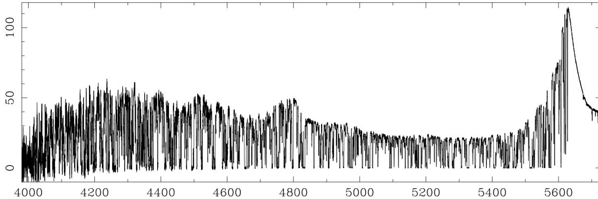
Fig. 1.12 High resolution spectrum of the Lyman- \alpha forest part of a quasar measured at z = 3.63 taken with the HIRES spectrograph on the 10 m Keck telescope in Hawaiï.
