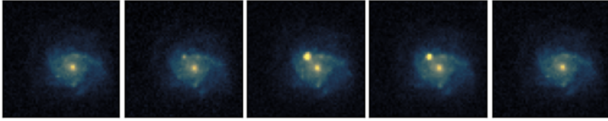
Fig. 3.3 Type Ia supernova detected by ZTF. Photos taken accross 2 months (from left to right 20th of Jan 2020, 25th of Jan 2020, 7th of Feb 2020, 20th of Feb 2020, 20th of March 2020). Credits: Mik  l Rigault.
