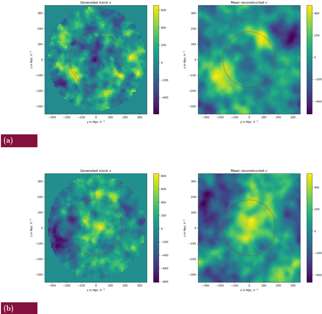
Fig. 6.23 Slices of the velocity field from Uchuu and BORG reconstruction after having gone a CIC mass assignment. The left column shows the Uchuu velocity field. The right column shows the mean posterior from BORG. Each row is a different slice in the box. The first row is a slice in the x axis. The second row is a slice in the y axis.
