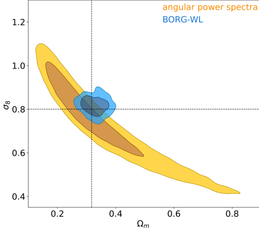
Fig. 5.3 Comparison of \Omega_m - \sigma_8 constraints from BORG-WL (blue) and the angular power spectrum (yellow) for self-consistent mocks.
