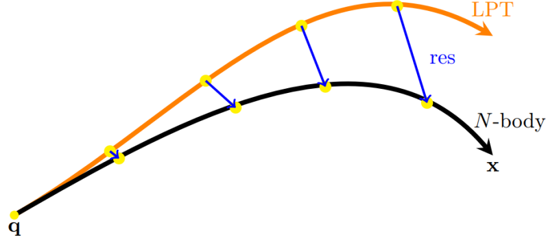
Fig. 5.4 Schematic representing how COLA works found in [Bartlett et al., 2025]. The orange line represents the motion of the particle from the LPT frame of reference and the blue lines are the residuals COLA calculates from the true position to correct for it.
