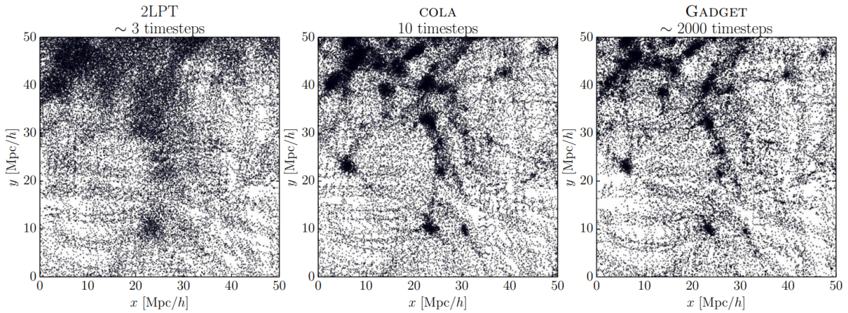
Fig. 5.5 Evolution of the same initial density field with three gravity solvers 2LPT, COLA and GADGET
