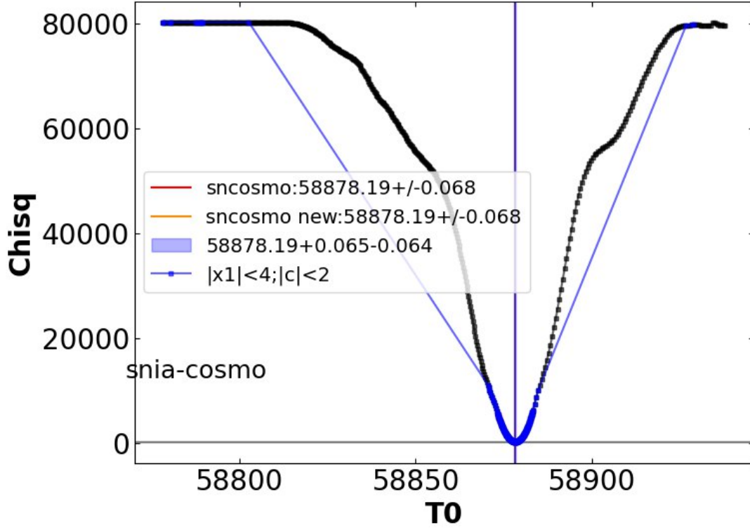
Fig. 3.14 Likelihood profile for a ZTF supernova in black. The blue region highlights where the stretch fit is |X_1| < 4 and the color is |c| < 2 with the SALT 2.4 model. The obtained t_{max} value from PeTS is 58878.19^{+0.065}_{-0.064} which is coherent with two sncosmo fits show values of 58878.19 \pm 0.068 . Credits: Thomas De Jaeger.
