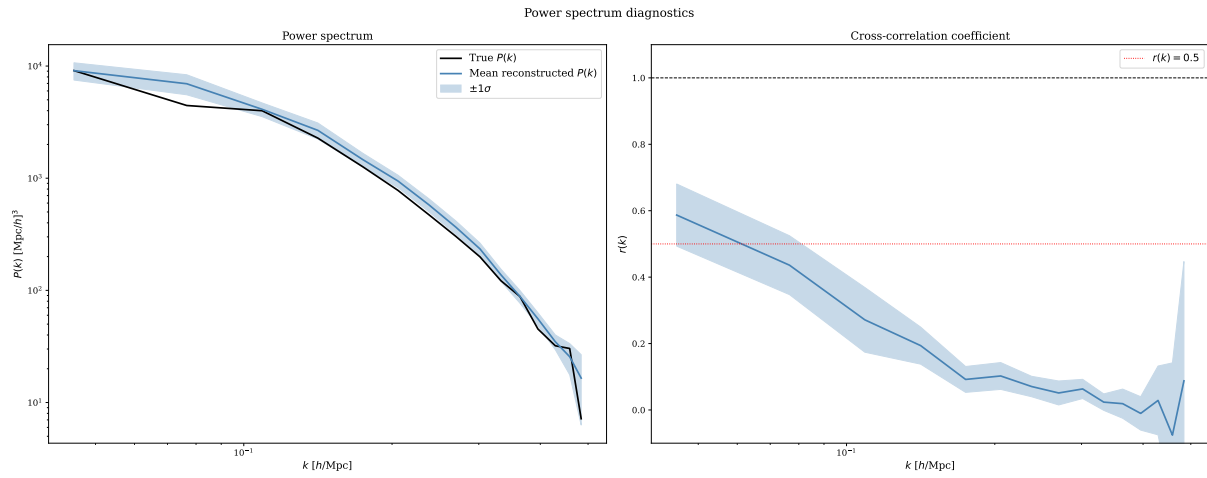
Fig. 6.12 Left: Matter power spectrum of the generated density field as well as the mean power spectrum and its standard deviation from the inference. Right: Cross correlation between the generated density field and the posterior mean field. The red dotted line represents a value of 0.5 where the correlations are at 50%.
