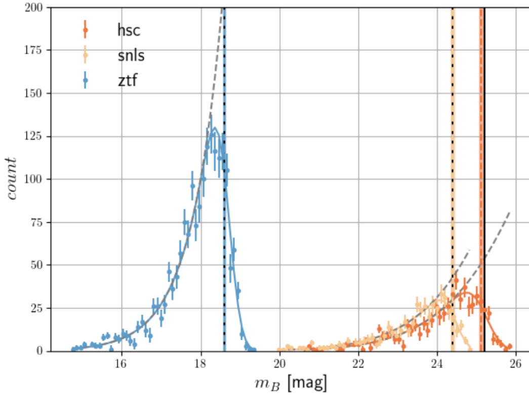
Fig. 3.15 Selection function fittings by EDRIS. The dots are the binned counts of simulated supernova for ZTF (blue), SNLS (light orange) and HSC (dark orange) as a function of magnitude. The solid line are the fitted selection functions for each survey. The dashed grey lines are the expected count distributions if the surveys did not present any selection effects. The vertical lines highlight the limiting magnitude of each survey. Credits: Dylan Kuhn.
