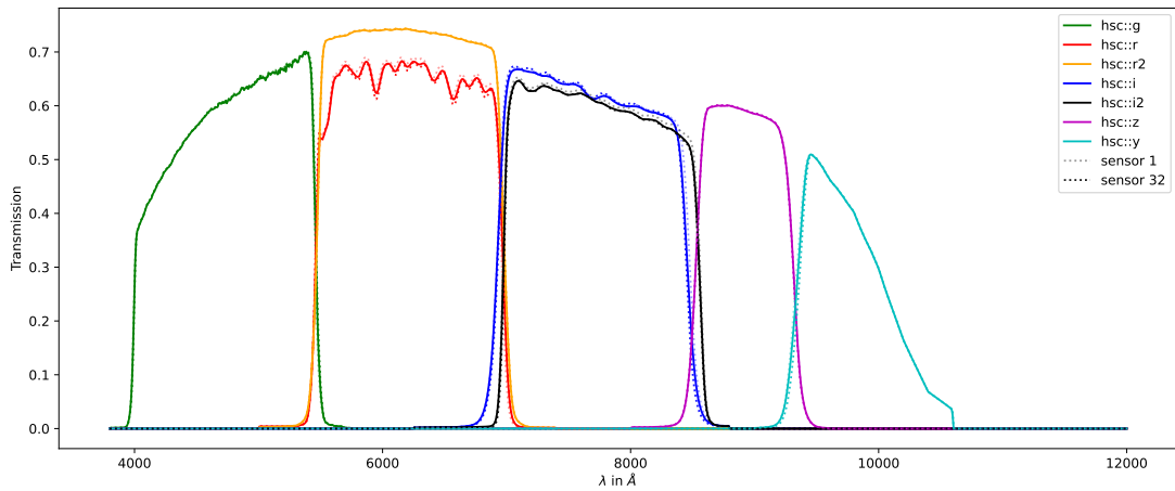
Fig. 3.12 HSC filters. Dotted lines represent transmissions for different sensors. Solid lines represent the average transmissions over all sensors.
