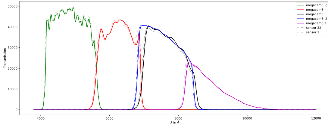
Fig. 3.10 SNLS filters. Dotted lines represent transmissions for different sensors. Solid lines represent the average transmissions over all sensors.
