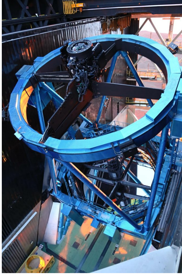
Fig. 3.11 The HSC camera on top of the Subaru telescope. Image from https://hsc.mtk.nao.ac.jp/ssp/gallery/
