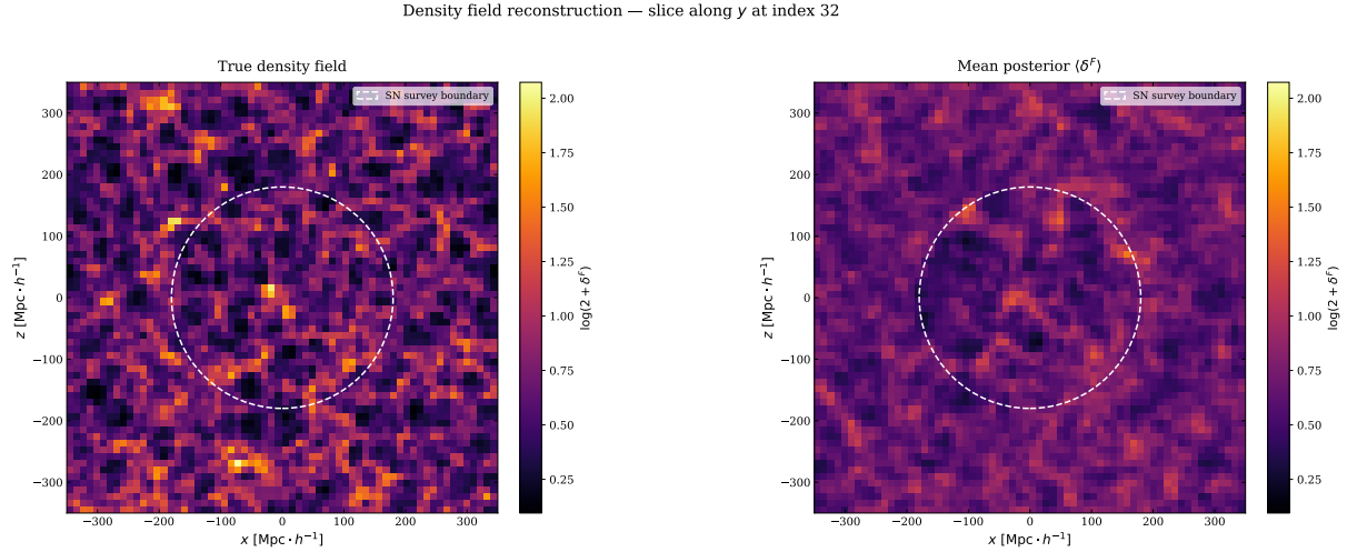
Fig. 6.9 Slice 32 on the y -axis of the generated density field and posterior mean using self-consistent simulations.
