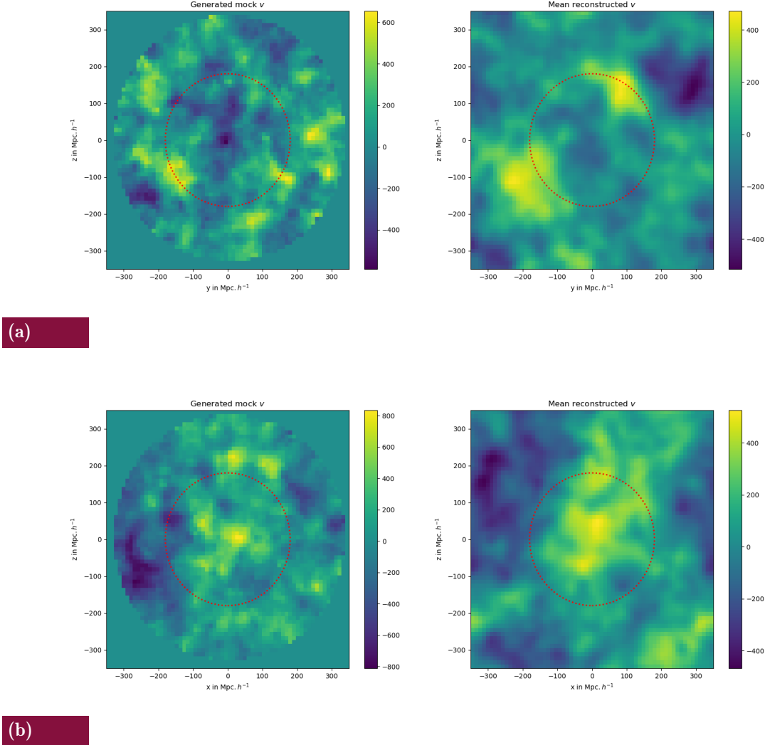
Fig. 6.19 Slices of the velocity field from Uchuu and BORG reconstruction after having gone a CIC mass assignment. The left column shows the Uchuu velocity field. The right column shows the mean posterior from BORG. Each row is a different slice in the box. The first row is a slice in the x axis. The second row is a slice in the y axis.
