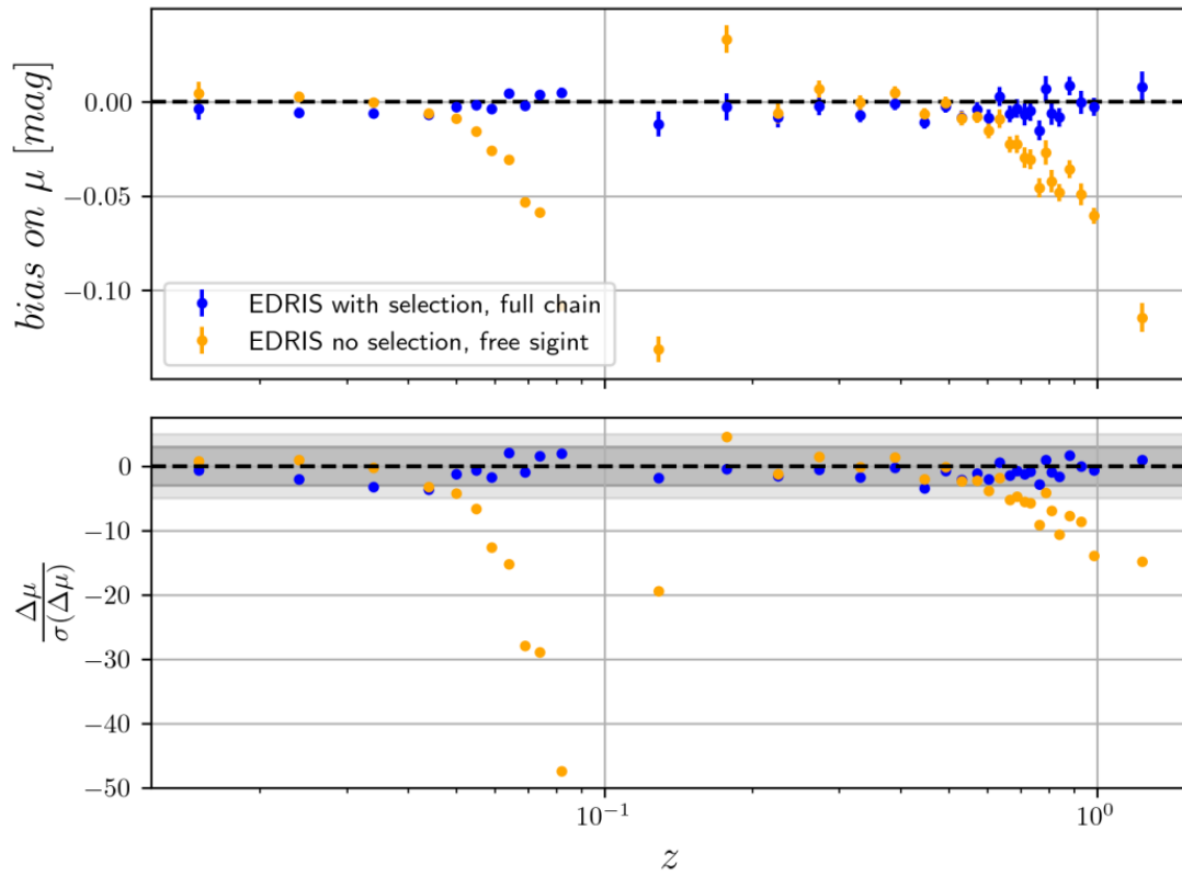
Fig. 3.16 Top: Bias on the reconstructed binned distance moduli for simulated supernovae when accounting for selection effects (blue) and when the selection effects are not accounted for (orange). Bottom: the weighted residuals for the reconstructed binned distance moduli for both cases.
