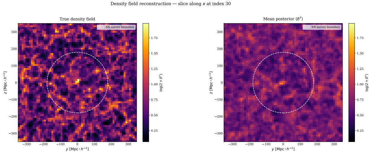
Fig. 6.7 Slice 30 on the x-axis of the generated density field and posterior mean using self-consistent simulations.
