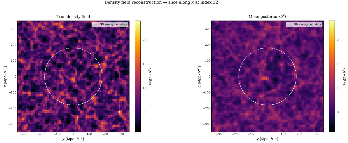
Fig. 6.8 Slice 32 on the x -axis of the generated density field and posterior mean using self-consistent simulations.
