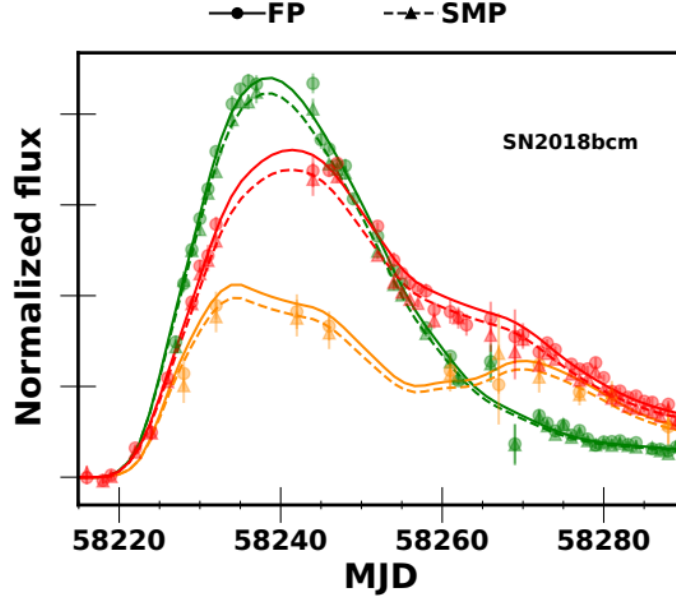
Fig. 3.13 Applications of the forced photometry (FP) model (circles) vs the SMP model (triangles) on a supernova lightcurves in the three ZTF bands as well as their SALT2.4 fits with sncoemo (solid and dashed lines). Taken from [Lacroix et al., 2025].
