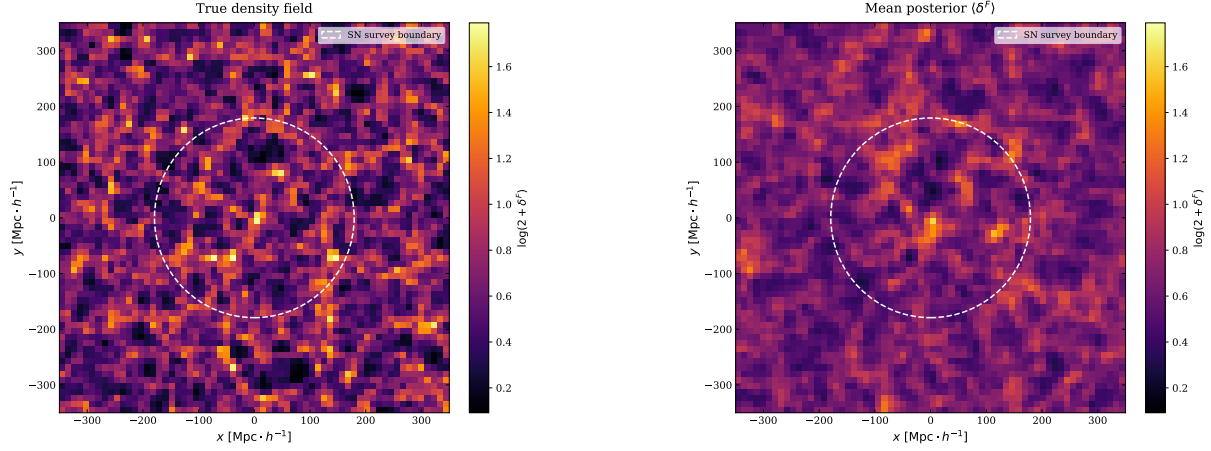
Fig. 6.10 Slice 30 on the z -axis of the generated density field and posterior mean using self-consistent simulations.
