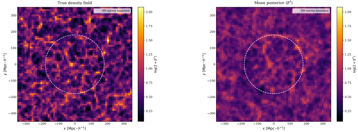
Fig. 6.11 Slice 32 on the z -axis of the generated density field and posterior mean using self-consistent simulations.
