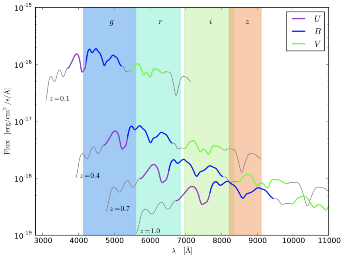
Fig. 2.9 Examples of four spectra at different redshifts 0.1, 0.4, 0.7 and 1.0. The highlighted parts of the spectra represent restframe band would measure. The highlighted areas on the graph are the regions where the observer bands measure.
