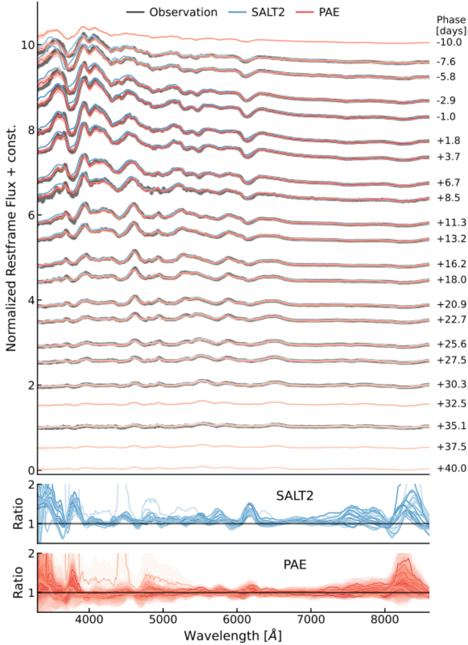
Fig. 2.20 Model comparisons from SuPAErnova (red) and SALT2 (blue) on the spectral series of the SN2010dt supernova observed by SNfactory (black) as well as ratios between model and data. Taken from [Stein et al., 2022]
