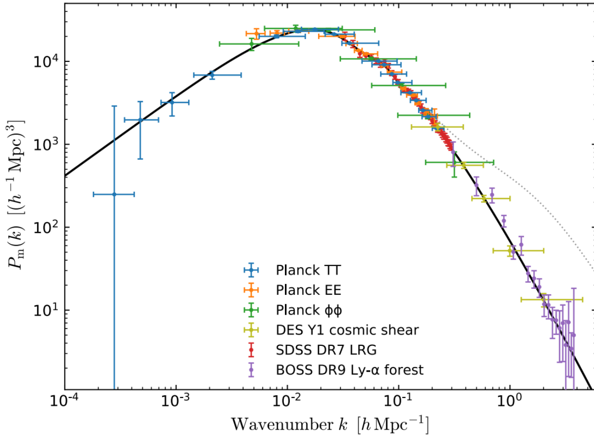
Fig. 1.8 Linear-theory matter power spectrum (at z = 0 ) inferred from different cosmological probes taken from [Collaboration et al., 2020].
