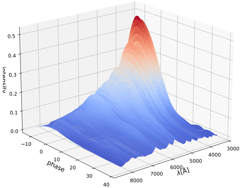
Fig. 2.13 The SALT2.4 M_0 surface with respect to the restframe wavelength and phase
