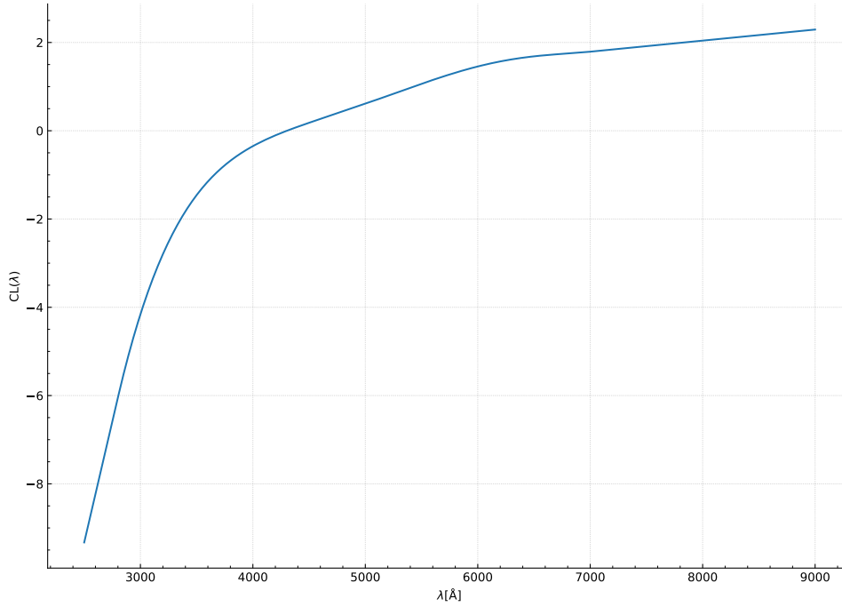
Fig. 2.15 The SALT2.4 color law CL surface with respect to the restframe wavelength
