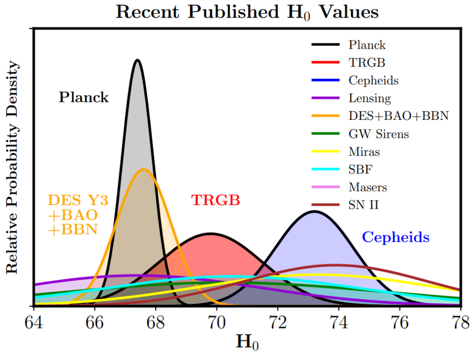
Fig. 1.12 Probability density functions of H_0 from different measurements probed at different redshifts, taken from [Freedman, 2021]. The CMB measurements prefer a lower H_0 value while Cepheids prefer higher values.
