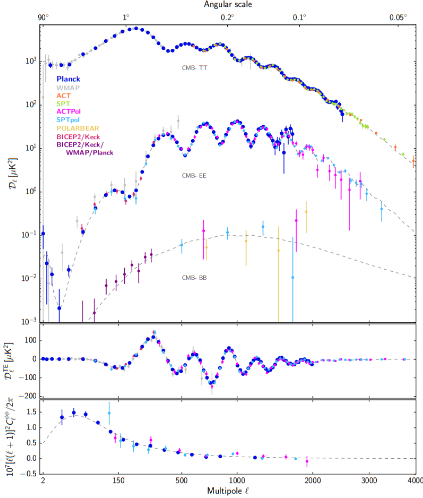
Fig. 1.7 Compilation of CMB angular power spectrum measurements from [Collaboration et al., 2020]. The upper panel shows the power spectra of the temperature and E -mode and B -mode polarization signals, the next panel the cross-correlation spectrum between T and E , while the lower panel shows the lensing deflection power spectrum
