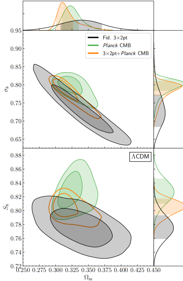
Fig. 1.10 A comparison of the marginalized parameter constraints in the \Lambda CDM model from the Dark Energy Survey ([DES Collaboration et al., 2022a]) with predictions from Planck CMB data (no lensing; green). There is also the fiducial cosmology 3x2pt (black) and the combined Y3 3x2pt and Planck (orange) results.
