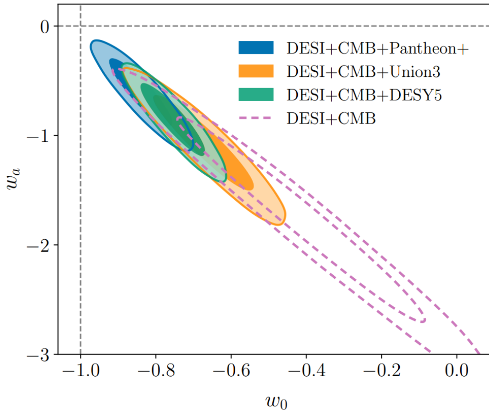
Fig. 1.14 w_0 and w_a contours from the latest [DESI Collaboration et al., 2025] measurements enclosing the the 68% and 95% posterior probability when combined with Pantheon+, UNION3 and DES year 5 data and CMB.
