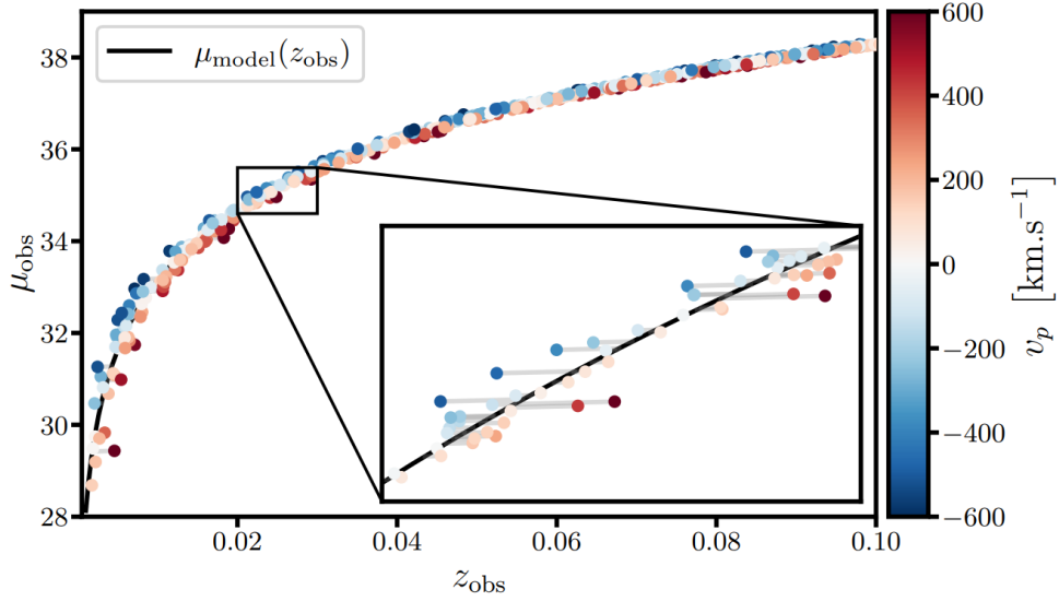
Fig. 2.8 Illustration of the impact of peculiar velocities on the distance modulus on a Hubble diagram from [Carreres et al., 2023]. The velocities were drawn randomly from a Gaussian distribution. The blue and red colors indicate the radial velocity of the supernova.
