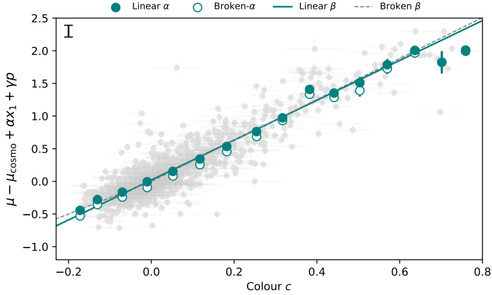
Fig. 2.11 Binned Hubble residuals as a function of color. The data is fitted to highlight the brighter-bluer effect ([Ginolin et al., 2025a]).
