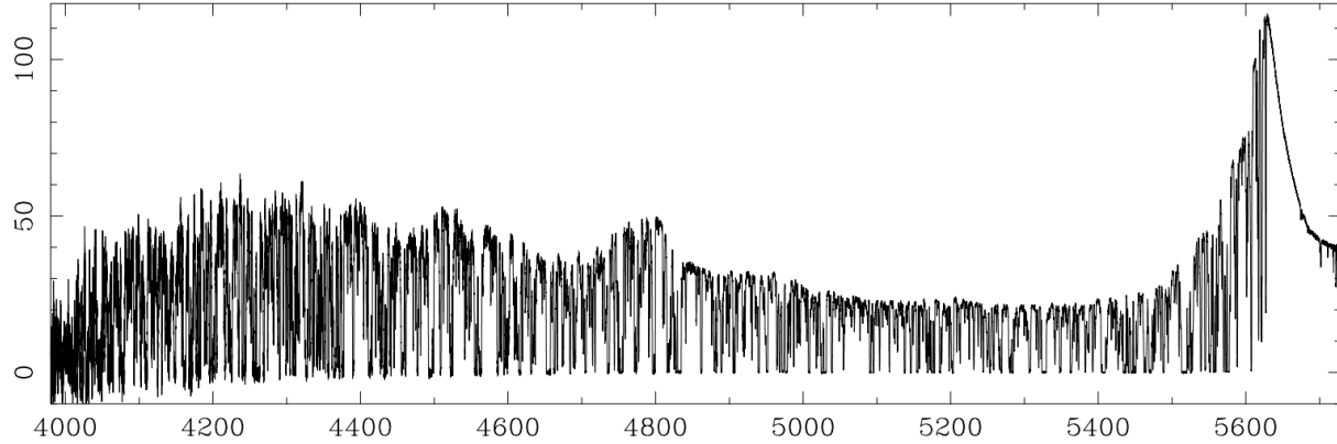
Fig. 1.11 High resolution spectrum of the Lyman- \alpha forest part of a quasar measured at z = 3.63 taken with the HIRES spectrograph on the 10 m Keck telescope in Hawaiï.
