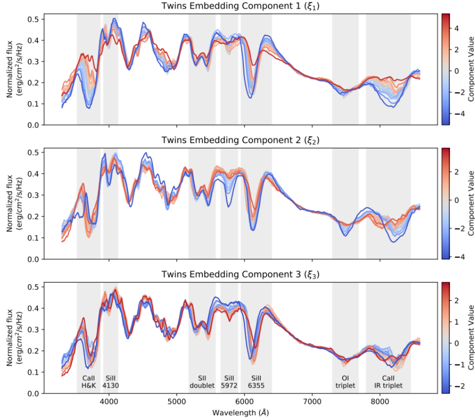
Fig. 2.19 Variations of the Twins Embedding model near maximum light when varying each one of its components \xi_1 , \xi_2 and \xi_3 . For each component, the spectrum shown is the median of 20 evenly populated bins of the coordinates of that component. Taken from [Boone et al., 2021].
