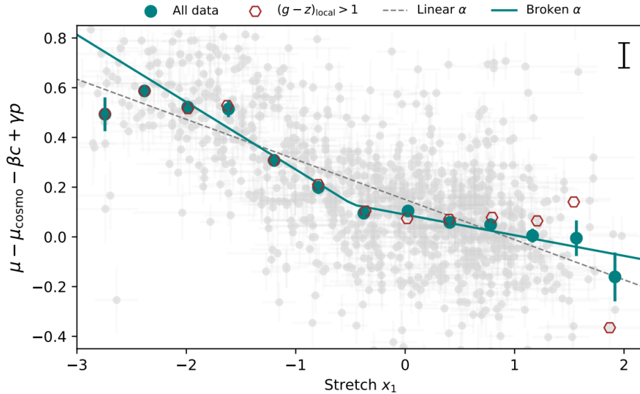
Fig. 2.10 Binned Hubble residuals as a function of the stretch. The data is fitted to highlight the two regimes of the broken alpha relation [Ginolin et al., 2025b].
