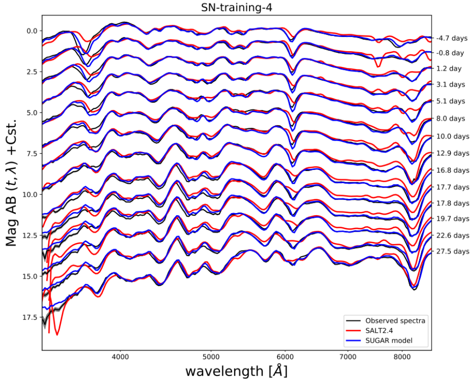
Fig. 2.17 SUGAR model (blue) vs SALT2.4 (red) on top of the SNfactory data (black) taken from [Léget et al., 2020].
