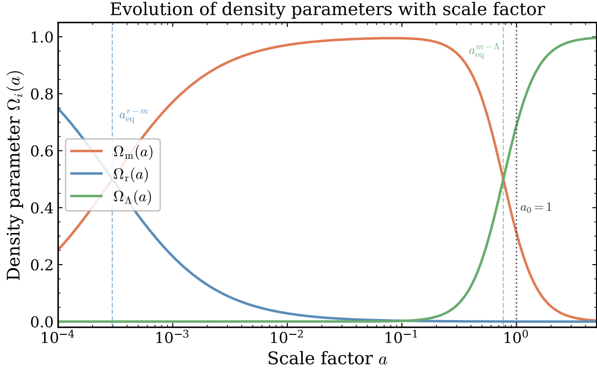
Fig. 1.4 Evolution of the main components of the \Lambda CDM model with respect to the scale factor. This highlights where each component dominates as well as when they become equal.
