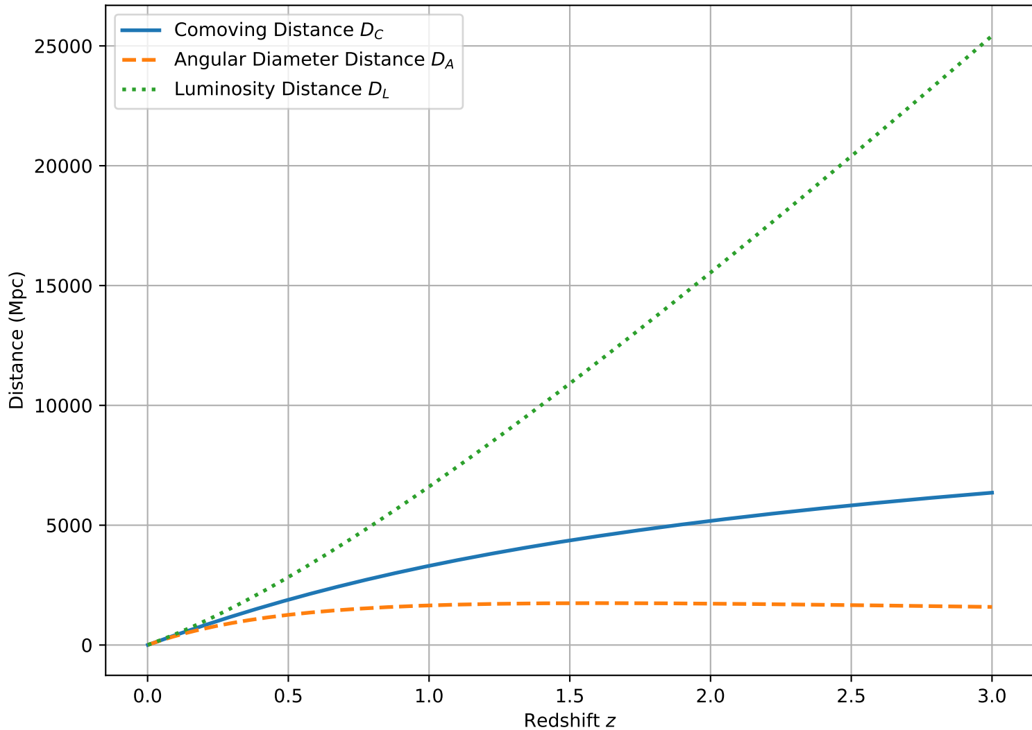
Cosmological Distance Measures
