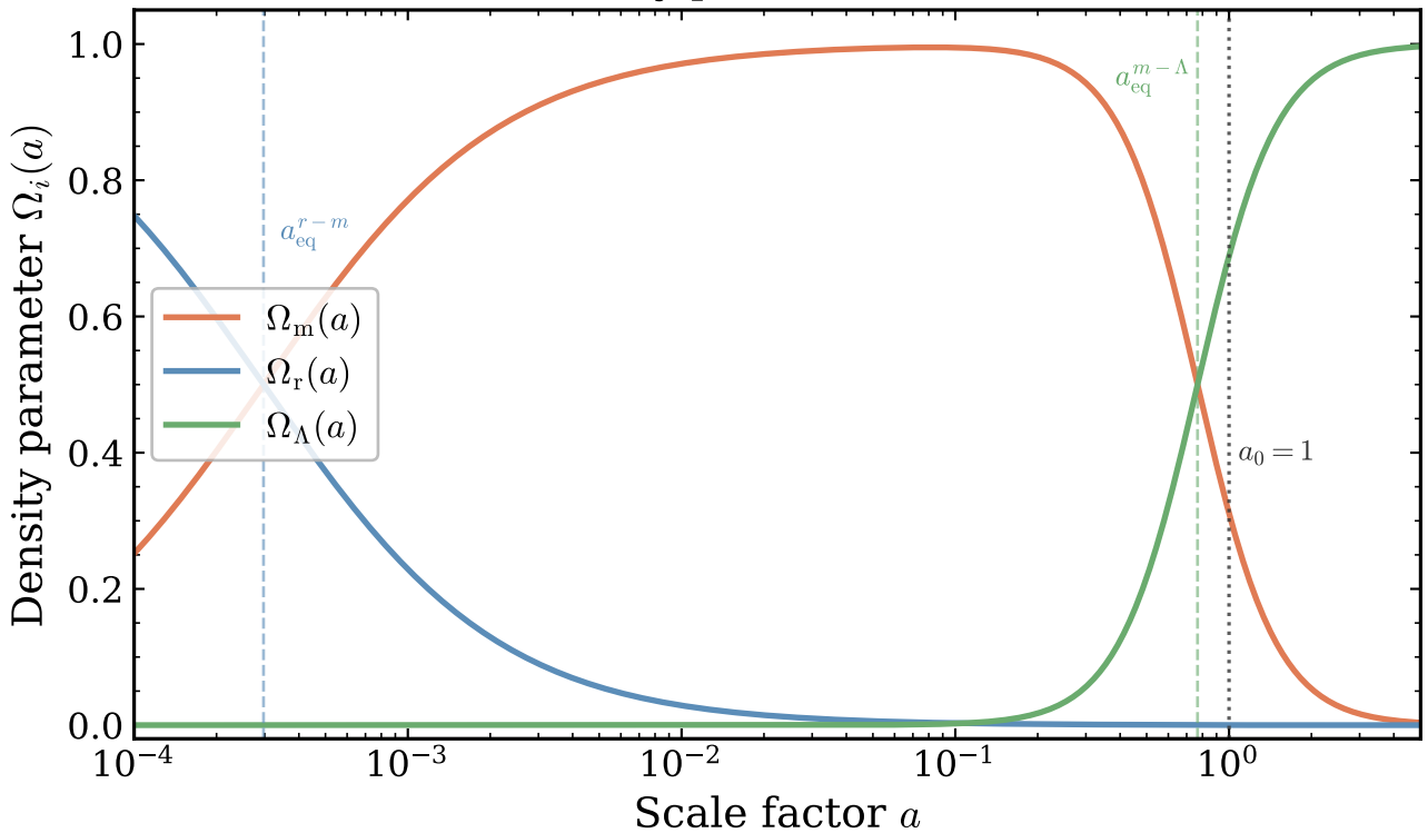
Evolution of density parameters with scale factor
