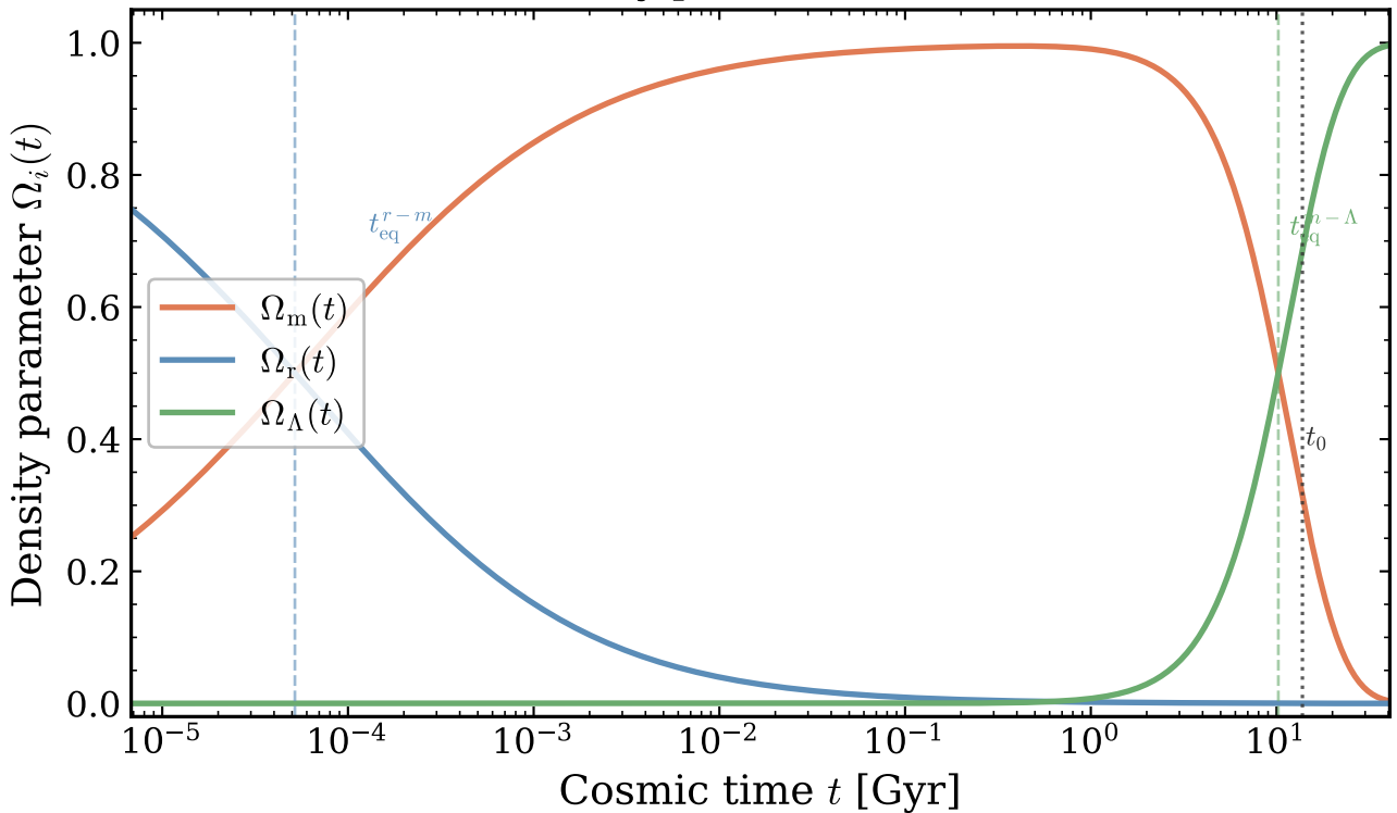
Evolution of density parameters with cosmic time
