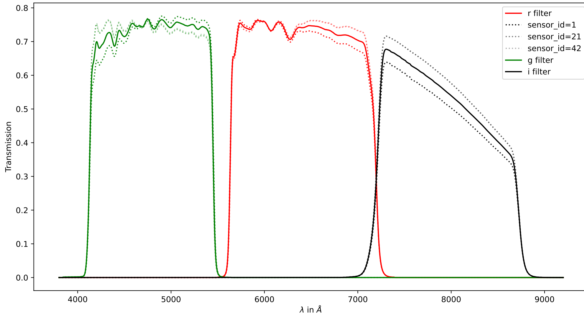
ZTF filters
