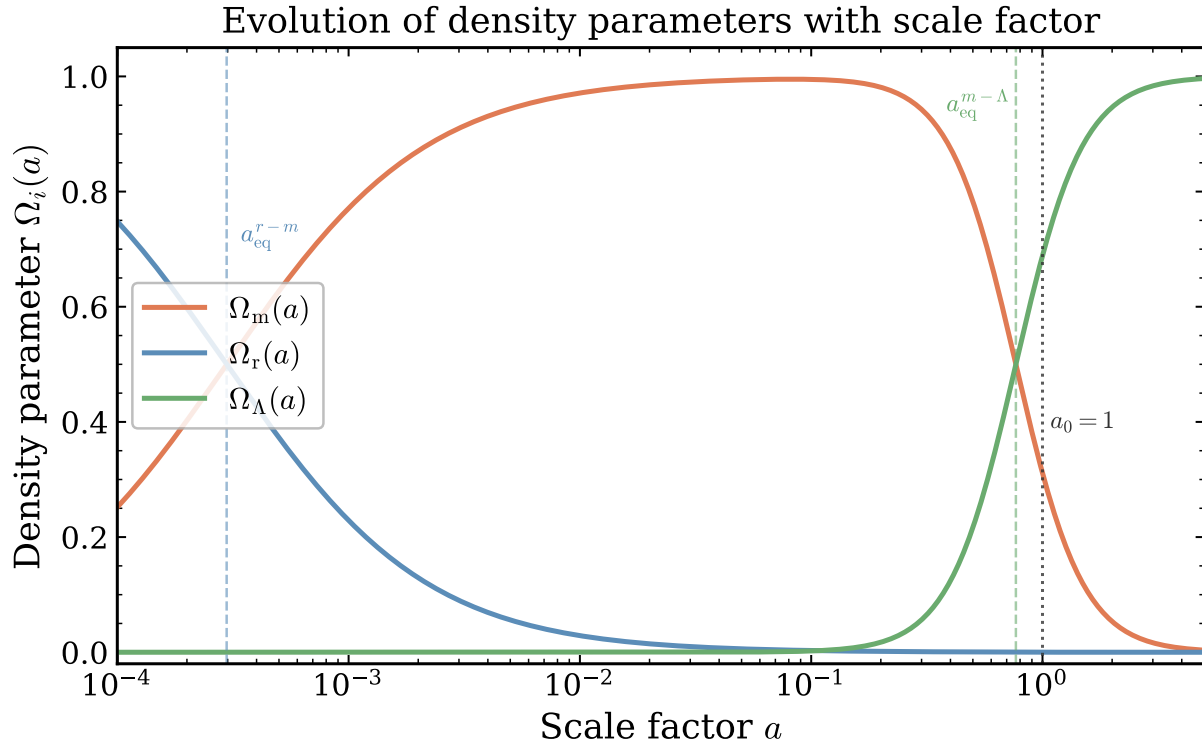
Fig. 1.5 Evolution of the main components of the \Lambda CDM model with respect to the scale factor. This highlights where each component dominates as well as when they become equal.
