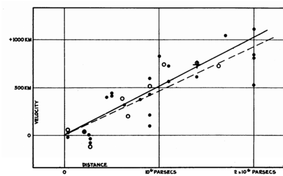
Fig. 1.4 Original Hubble diagram ([Hubble, 1929]) portraying the distance velocity diagram of nearby galaxies.
