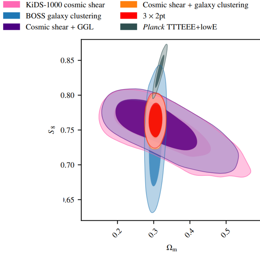
Fig. 1.14 S_8 and \Omega_m contours for different galaxy surveys and CMB taken from [Heymans et al., 2021b] enclosing the 68% and 95% posterior probability. It is highlighted that CMB measurements prefer higher S_8 values to galaxy surveys.
