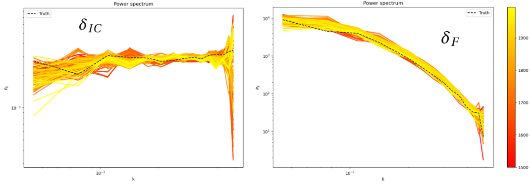
Fig. 6.7 (PLOT NEEDS TO BE REMADE) Reconstructed power spectra at each mcmc step vs the true power spectrum in black for the initial conditions (Left) and final density field (Right).
