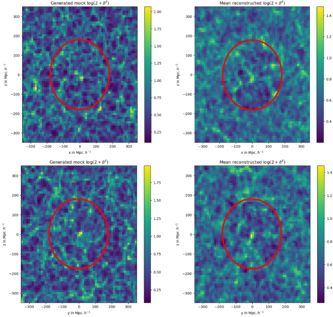
Fig. 6.6 (PLOT NEEDS TO BE REMADE) Two slices of the generated and reconstructed density fields using self-consistent simulations in each row.
