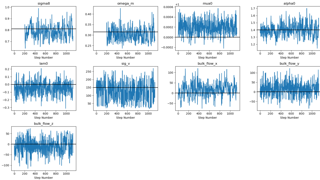
Fig. 6.8 (PLOTS FROM DEAGLAN REDO THEM) Model and cosmological parameter sampling for the self-consistent simulation run.
